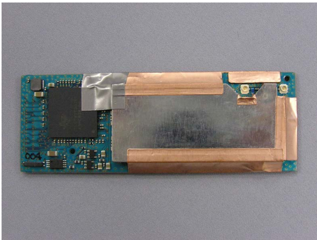
Front View of Wireless LAN Module with Shielding
