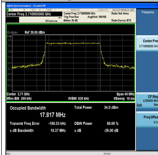
NTNV-n77(3700-3980)-PC2-30-20-L-DFT-256QAM-Outer_Full-Ant1-PASS
