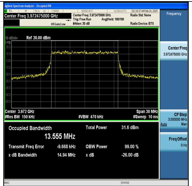
NTNV-n77(3700-3980)-PC2-30-15-H-CP-256QAM- Outer_Full-Ant1-PASS
