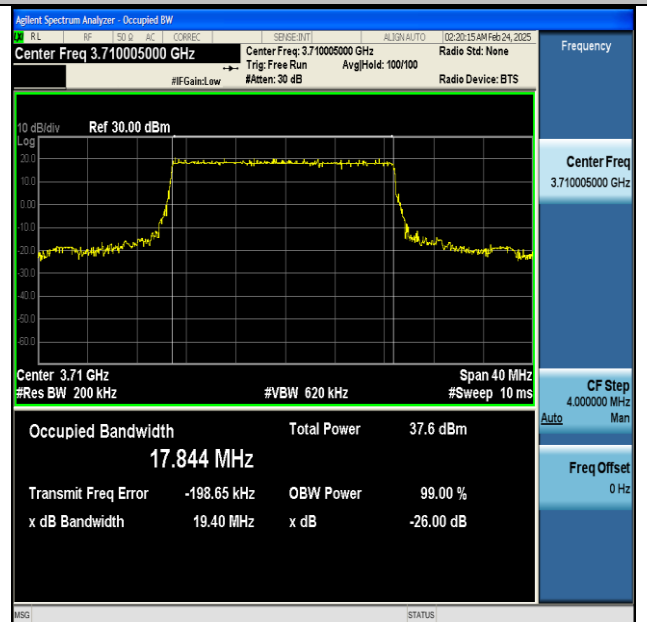
NTNV-n77(3700-3980)-PC2-30-20-L-DFT-QPSK- Outer_Full-Ant1-PASS
