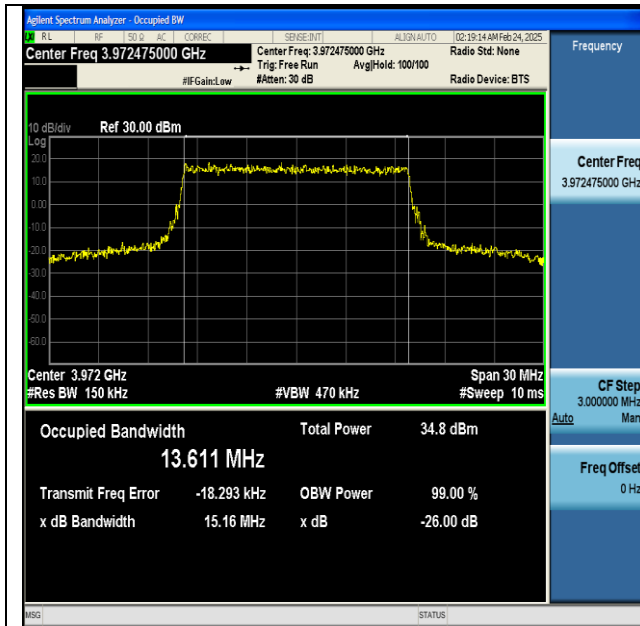
NTNV-n77(3700-3980)-PC2-30-15-H-CP-64QAM- Outer_Full-Ant1-PASS
