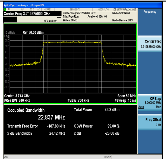
NTNV-n77(3700-3980)-PC2-30-25-L-DFT-16QAM- Outer_Full-Ant1-PASS
