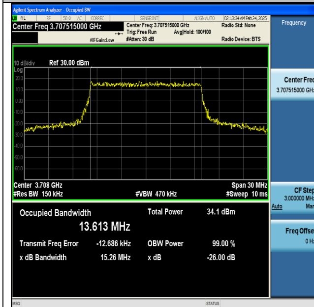
NTNV-n77(3700-3980)-PC2-30-15-L-CP-64QAM- Outer_Full-Ant1-PASS
