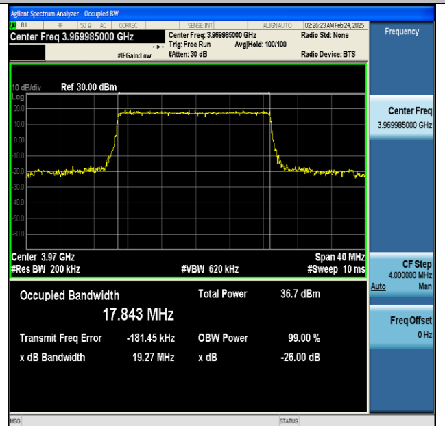
NTNV-n77(3700-3980)-PC2-30-20-H-DFT-64QAM-Outer_Full-Ant1-PASS
