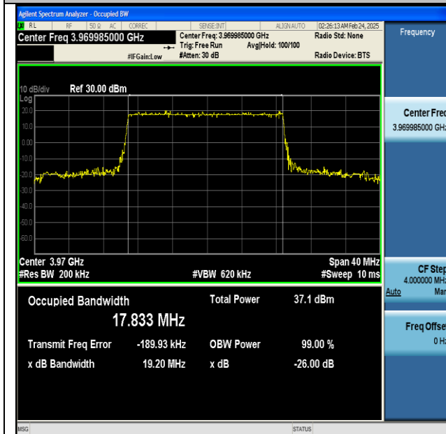
NTNV-n77(3700-3980)-PC2-30-20-H-DFT-16QAM-Outer_Full-Ant1-PASS
