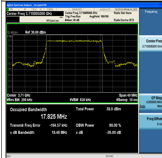
NTNV-n77(3700-3980)-PC2-30-20-L-DFT-BPSK- Outer_Full-Ant1-PASS
