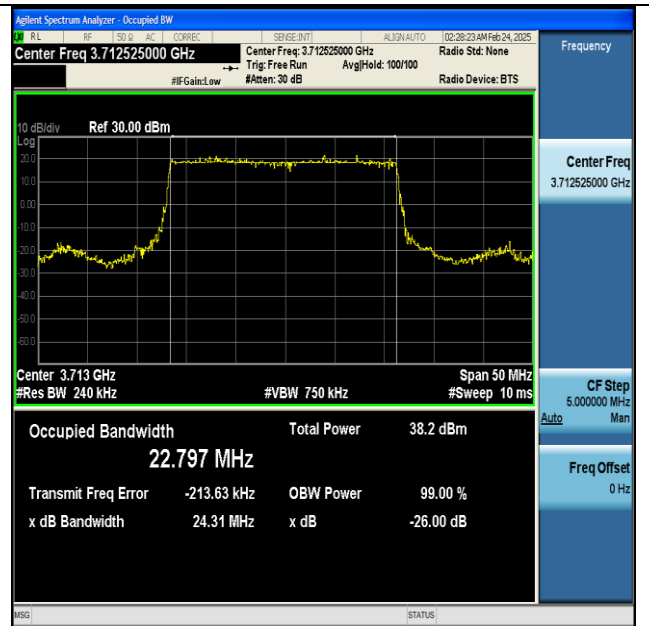
NTNV-n77(3700-3980)-PC2-30-25-L-DFT-BPSK- Outer_Full-Ant1-PASS
