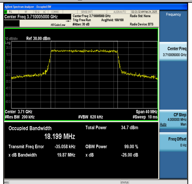
NTNV-n77(3700-3980)-PC2-30-20-L-CP-QPSK-Outer_Full-Ant1-PASS
