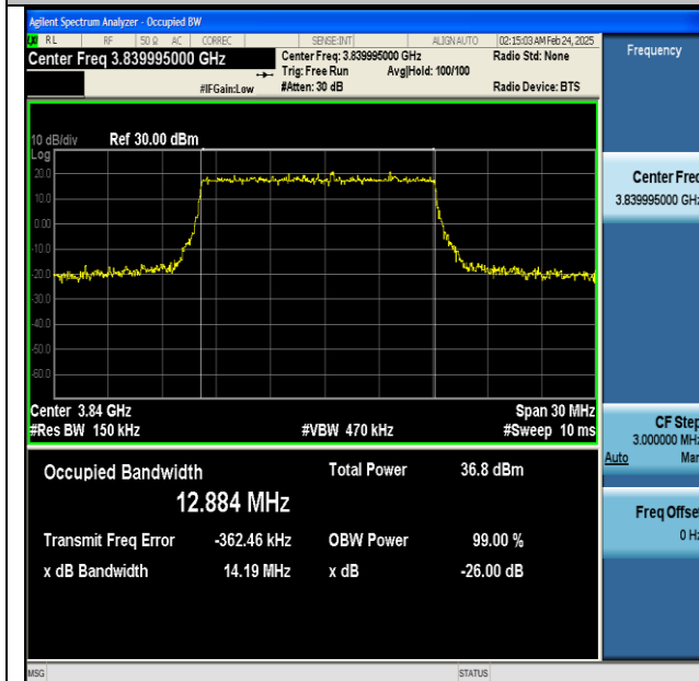
NTNV-n77(3700-3980)-PC2-30-15-M-DFT-16QAM- Outer_Full-Ant1-PASS
