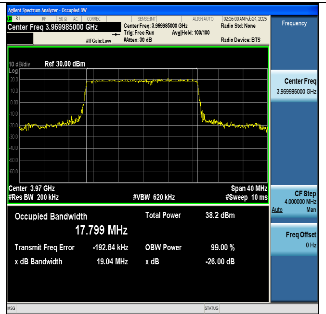
NTNV-n77(3700-3980)-PC2-30-20-H-DFT-QPSK-Outer_Full-Ant1-PASS
