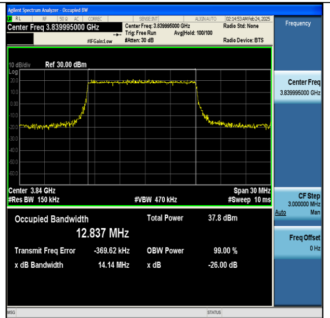
NTNV-n77(3700-3980)-PC2-30-15-M-DFT-QPSK- Outer_Full-Ant1-PASS
