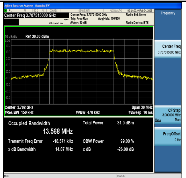
NTNV-n77(3700-3980)-PC2-30-15-L-CP-256QAM- Outer_Full-Ant1-PASS
