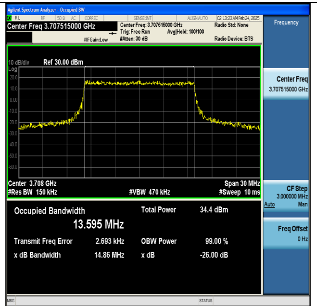
NTNV-n77(3700-3980)-PC2-30-15-L-CP-16QAM- Outer_Full-Ant1-PASS
