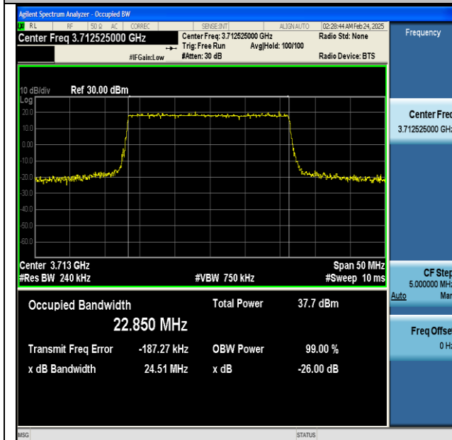
NTNV-n77(3700-3980)-PC2-30-25-L-DFT-QPSK- Outer_Full-Ant1-PASS
