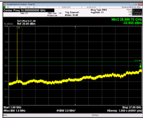
41-41-20MHz-5MHz-64QAM-64QAM-41440-41557-1RB#0- 0RB#0-1000~27000MHz-PASS
