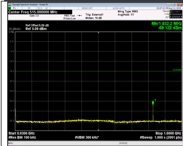
41-41-20MHz-10MHz-16QAM-16QAM-40571-40715-100 RB#0-50RB#0-30~1000MHz-PASS
