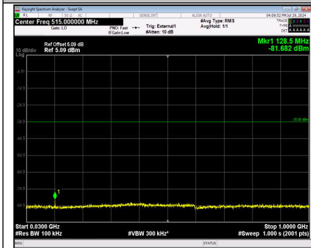
41-41-20MHz-10MHz-64QAM-64QAM-39750-39894-1RB #0-0RB#0-30~1000MHz-PASS
