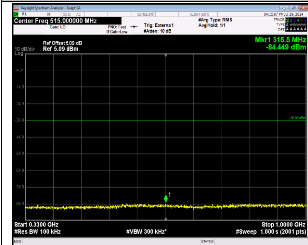
41-41-20MHz-10MHz-64QAM-64QAM-40571-40715-1RB #0-1RB#49-30~1000MHz-PASS
