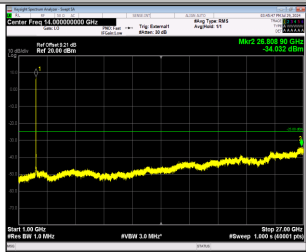
41-41-20MHz-5MHz-64QAM-64QAM-40595-40712-100RB# 0-25RB#0-1000~27000MHz-PASS
