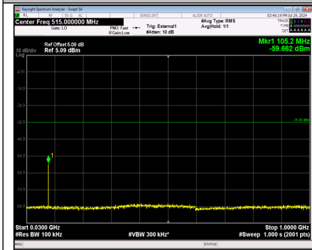
41-41-20MHz-5MHz-64QAM-64QAM-41440-41557-1RB# 0-0RB#0-30~1000MHz-PASS
