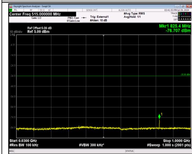
41-41-20MHz-5MHz-64QAM-64QAM-39750-39867-100RB# B#0-25RB#0-30~1000MHz-PASS
