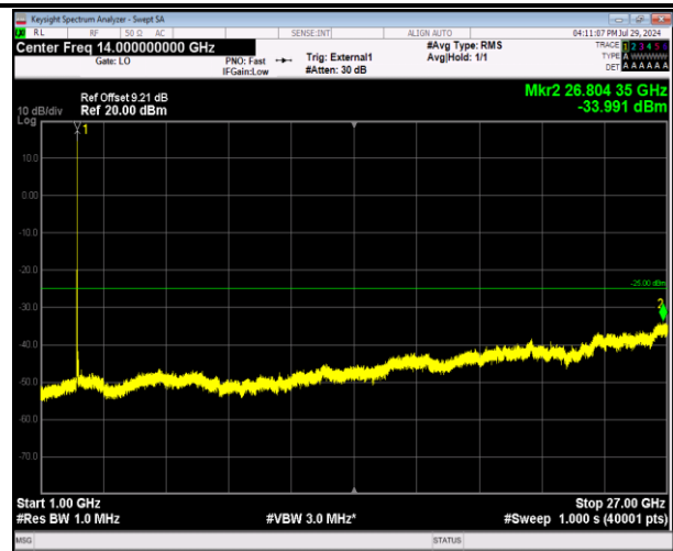
41-41-20MHz-10MHz-64QAM-64QAM-39750-39894-1RB#9 9-0RB#0-1000~27000MHz-PASS
