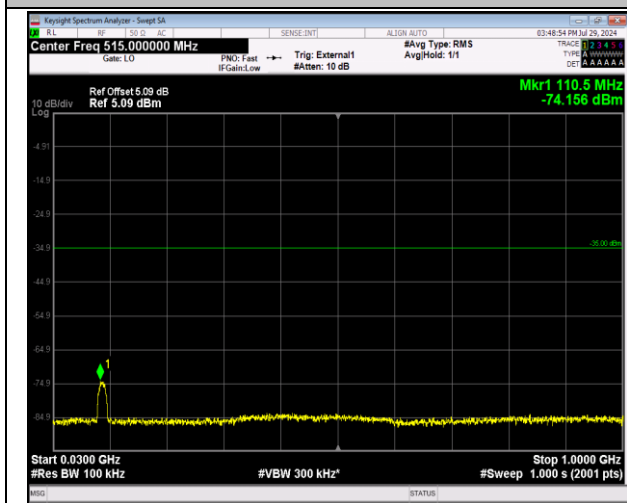
41-41-20MHz-5MHz-64QAM-64QAM-41440-41557-100RB# B#0-25RB#0-30~1000MHz-PASS
