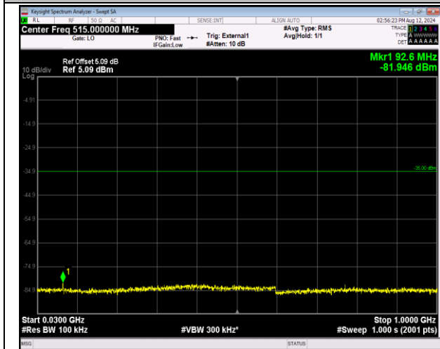
41-41-20MHz-10MHz-16QAM-16QAM-39750-39894-1RB #99-ORB#0-30~1000MHz-PASS
