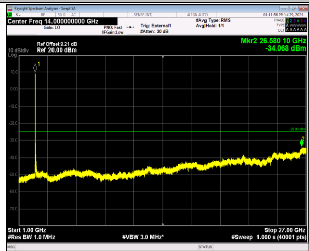
41-41-20MHz-10MHz-64QAM-64QAM-39750-39894-1RB#0 -1RB#49-1000~27000MHz-PASS
