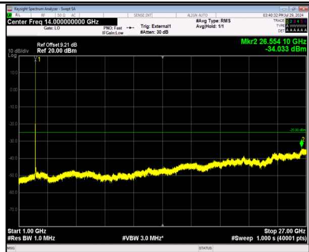
41-41-20MHz-5MHz-64QAM-64QAM-39750-39867-1RB#99 -ORB#0-1000~27000MHz-PASS
