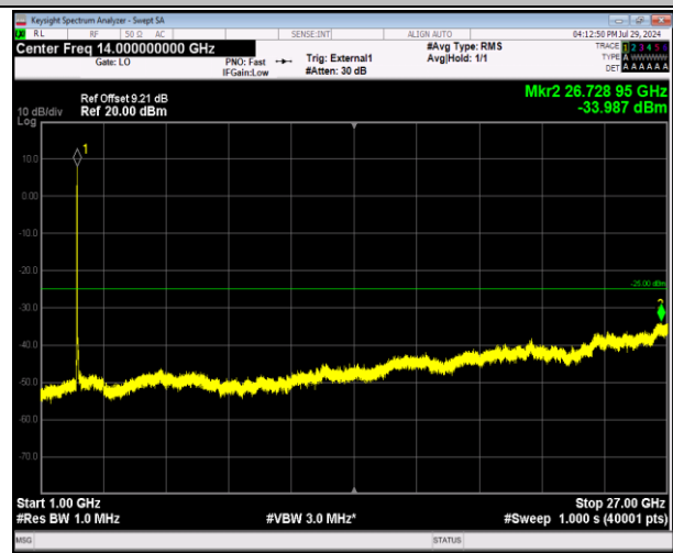
41-41-20MHz-10MHz-64QAM-64QAM-39750-39894-100RB #0-50RB#0-1000~27000MHz-PASS
