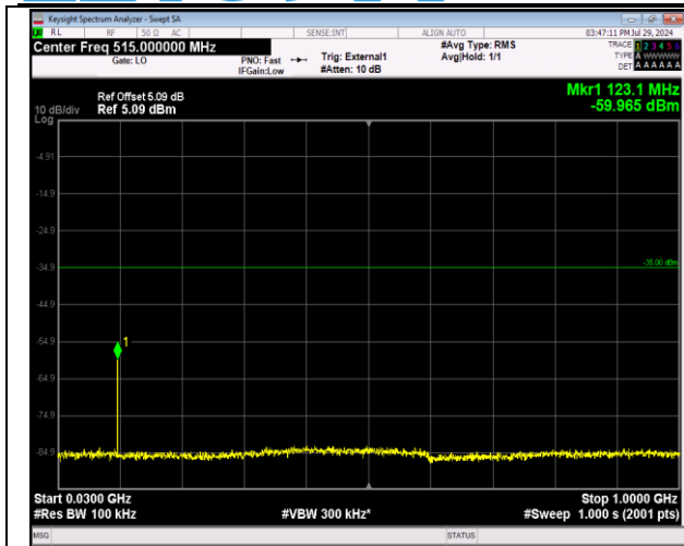
41-41-20MHz-5MHz-64QAM-64QAM-41440-41557-1RB# 99-ORB#0-30~1000MHz-PASS
