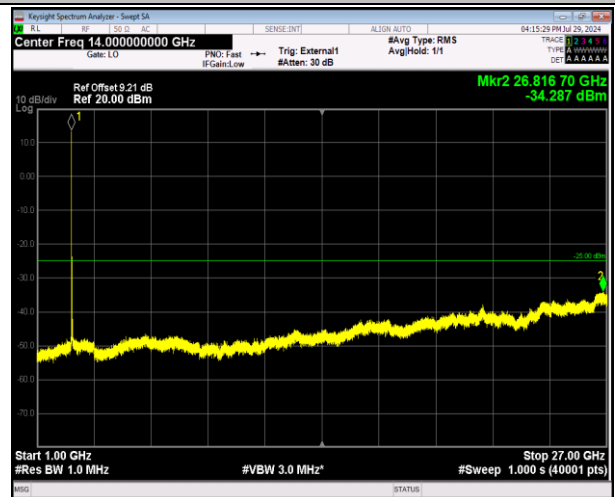
41-41-20MHz-10MHz-64QAM-64QAM-40571-40715-1RB#0 -1RB#49-1000~27000MHz-PASS
