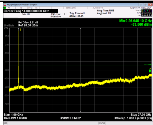
41-41-20MHz-5MHz-16QAM-16QAM-41440-41557-1RB#99 -ORB#0-1000~27000MHz-PASS
