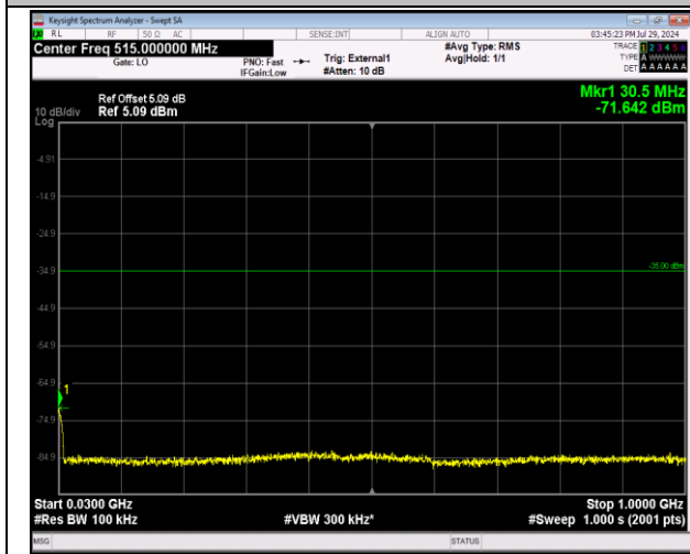
41-41-20MHz-5MHz-64QAM-64QAM-40595-40712-100R B#0-25RB#0-30~1000MHz-PASS
