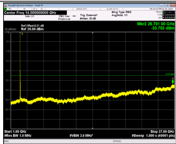
41-41-20MHz-10MHz-64QAM-64QAM-39750-39894-1RB#0 -0RB#0-1000~27000MHz-PASS
