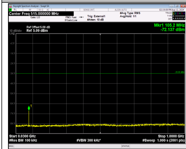
41-41-20MHz-5MHz-16QAM-16QAM-41440-41557-1RB# 0-1RB#24-30~1000MHz-PASS
