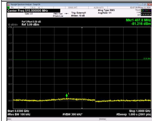
41-41-20MHz-5MHz-QPSK-QPSK-40595-40712-1RB#0- ORB#0-30~1000MHz-PASS
