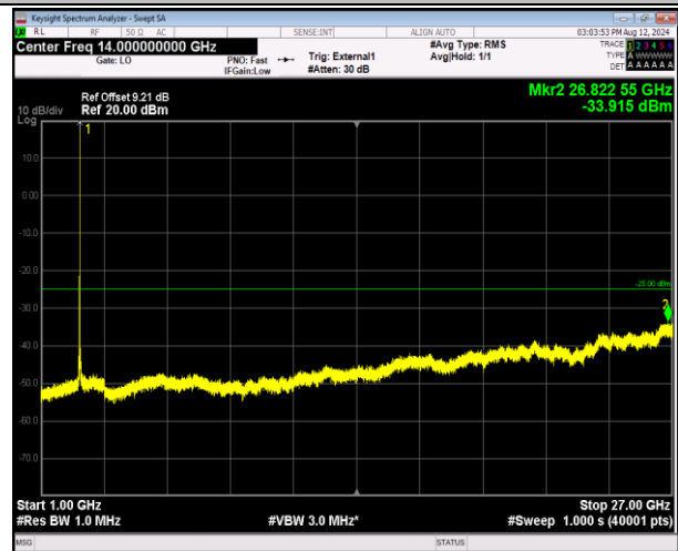
41-41-20MHz-10MHz-16QAM-16QAM-40571-40715-1RB#9 9-ORB#0-1000~27000MHz-PASS
