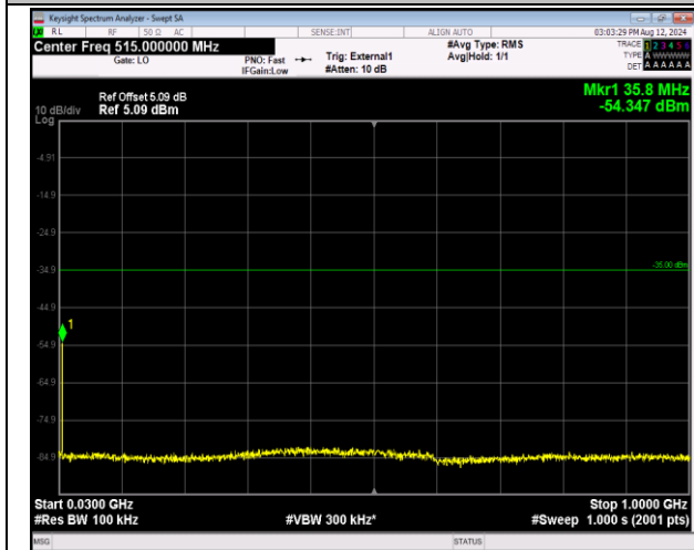
41-41-20MHz-10MHz-16QAM-16QAM-40571-40715-1RB #99-ORB#0-30~1000MHz-PASS
