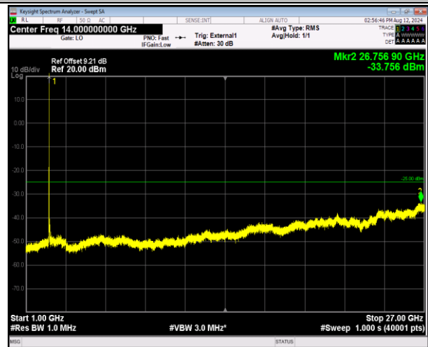
41-41-20MHz-10MHz-16QAM-16QAM-39750-39894-1RB#9 9-ORB#0-1000~27000MHz-PASS
