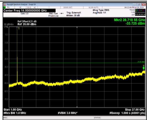
41-41-20MHz-10MHz-64QAM-64QAM-40571-40715-1RB#0 -0RB#0-1000~27000MHz-PASS
