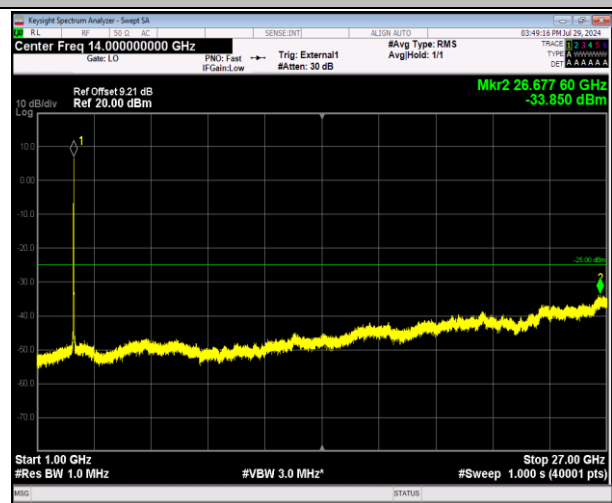
41-41-20MHz-5MHz-64QAM-64QAM-41440-41557-100RB# 0-25RB#0-1000~27000MHz-PASS
