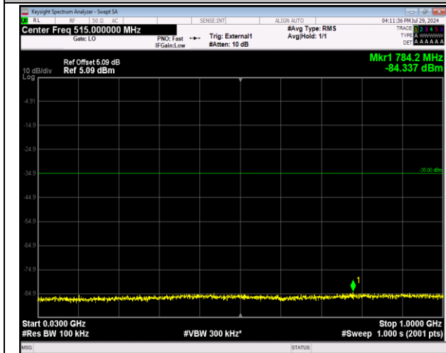
41-41-20MHz-10MHz-64QAM-64QAM-39750-39894-1RB #0-1RB#49-30~1000MHz-PASS
