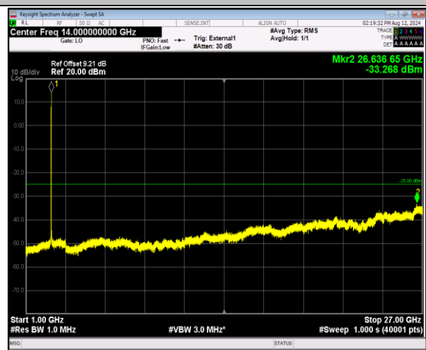
41-41-20MHz-5MHz-16QAM-16QAM-41440-41557-1RB#0- 1RB#24-1000~27000MHz-PASS
