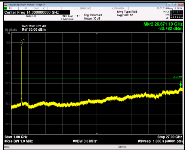
41-41-20MHz-10MHz-16QAM-16QAM-40571-40715-100RB #0-50RB#0-1000~27000MHz-PASS
