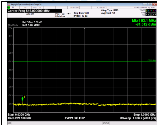
41-41-20MHz-5MHz-64QAM-64QAM-39750-39867-1RB# 99-ORB#0-30~1000MHz-PASS
