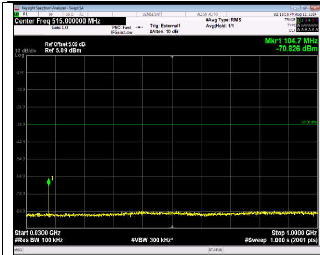
41-41-20MHz-5MHz-QPSK-QPSK-41440-41557-1RB#0-1RB#24-30~1000MHz-PASS
