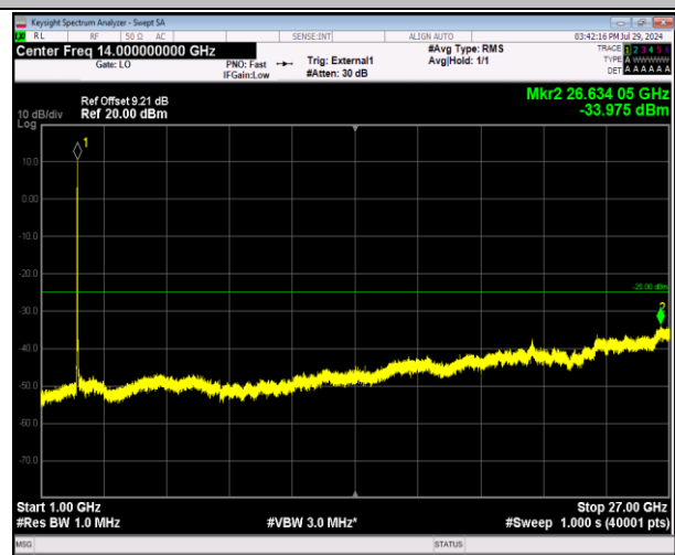
41-41-20MHz-5MHz-64QAM-64QAM-39750-39867-100RB# 0-25RB#0-1000~27000MHz-PASS
