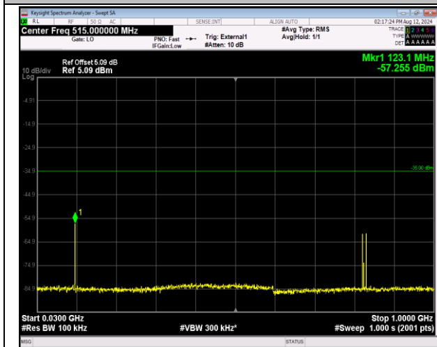
41-41-20MHz-5MHz-16QAM-16QAM-41440-41557-1RB# 99-ORB#0-30~1000MHz-PASS
