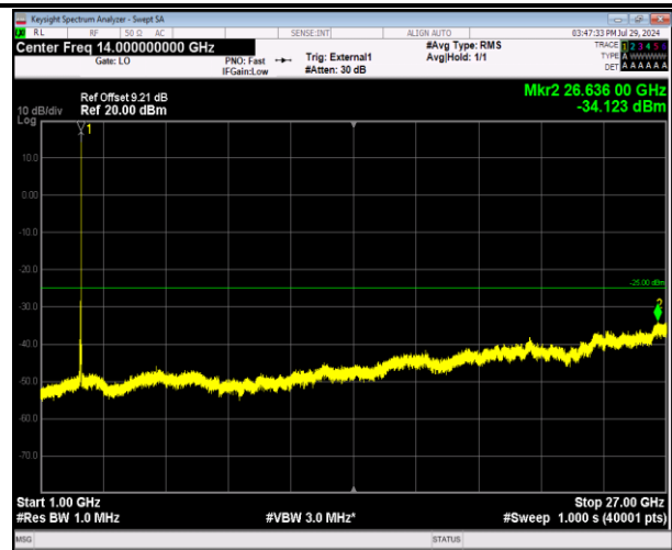
41-41-20MHz-5MHz-64QAM-64QAM-41440-41557-1RB#99 -ORB#0-1000~27000MHz-PASS
