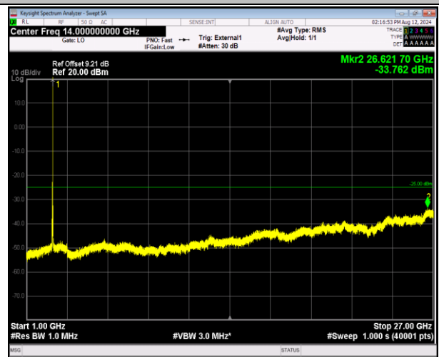
41-41-20MHz-5MHz-QPSK-QPSK-41440-41557-1RB#99-0RB#0-1000~27000MHz-PASS
