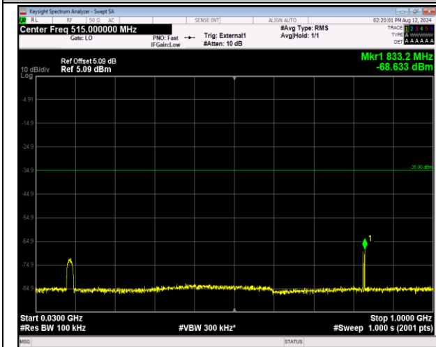
41-41-20MHz-5MHz-QPSK-QPSK-41440-41557-100RB#0-25RB#0-30~1000MHz-PASS
