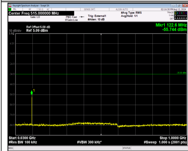
41-41-20MHz-5MHz-QPSK-QPSK-41440-41557-1RB#99-0RB#0-30~1000MHz-PASS
