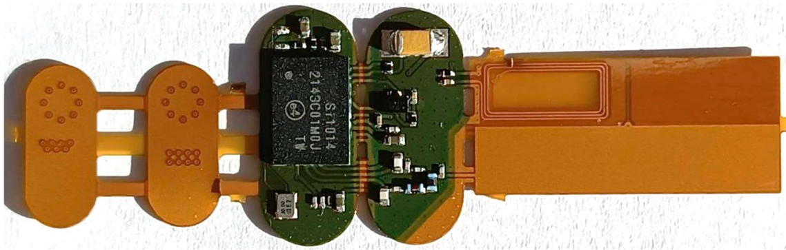
PCB Top view
