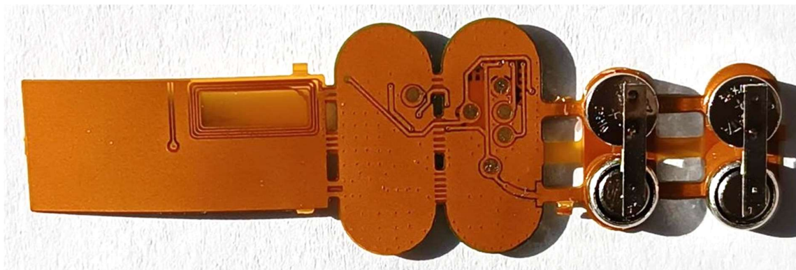
PCB Bottom View
