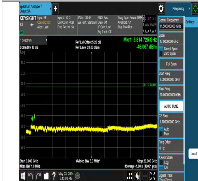
Band2_3MHz_QPSK_19185_1RB#0_3000~20000_3000~20000
