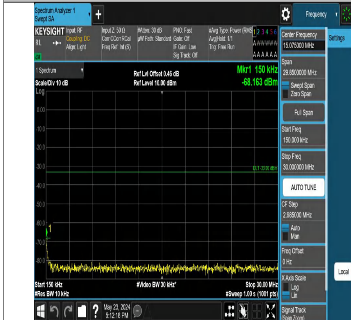
Band2_3MHz_QPSK_18900_1RB#14_0.15~30_0.15~30
