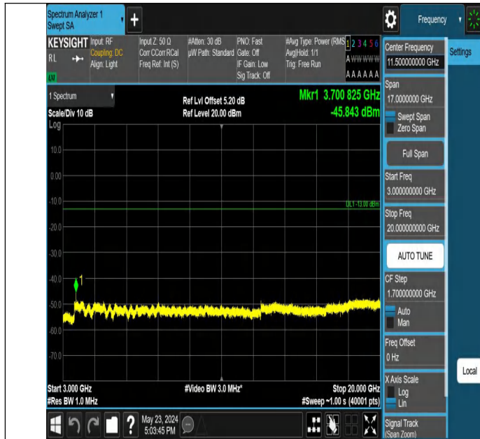
Band2_1.4MHz_QPSK_18607_1RB#0_3000~20000_3000~20000
