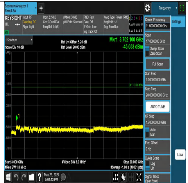
Band2_1.4MHz_QPSK_18607_1RB#5_3000~20000_3000~20000
