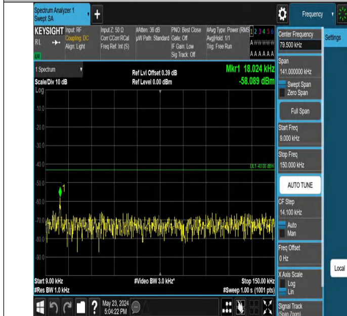
Band2_1.4MHz_QPSK_18900_1RB#0_0.009~0.15_0.009~0.15
