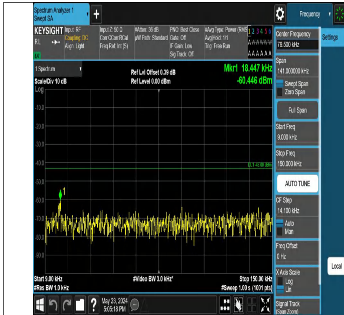
Band2_1.4MHz_QPSK_19193_1RB#0_0.009~0.15_0.009~0.15
