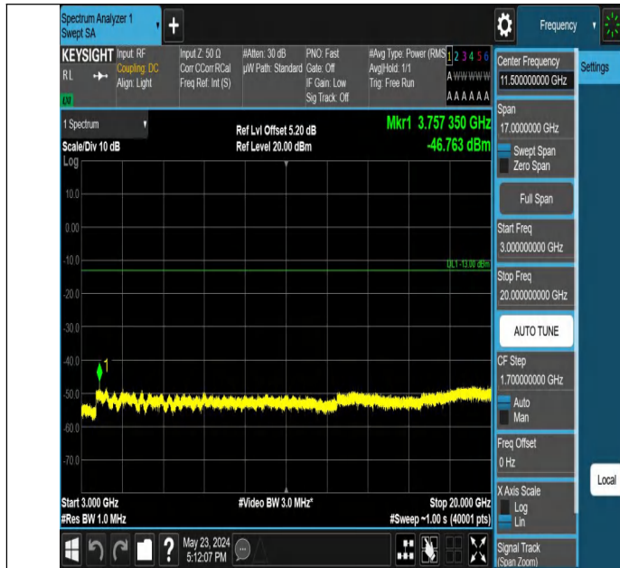
Band2_3MHz_QPSK_18900_1RB#0_3000~20000_3000~20000
