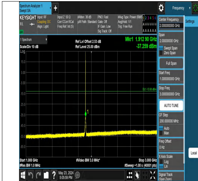
Band2_1.4MHz_QPSK_19193_1RB#5_1000~3000_1000~3000
