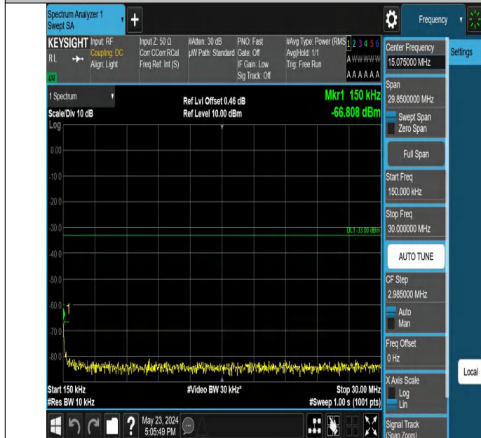
Band2_1.4MHz_QPSK_19193_1RB#5_0.15~30_0.15~30
