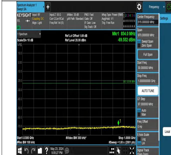
Band2_1.4MHz_QPSK_19193_1RB#0_30~1000_30~1000
