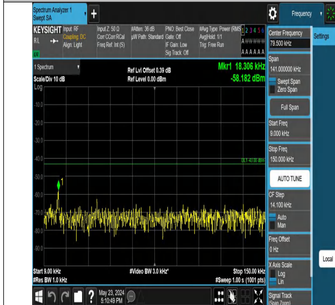
Band2_3MHz_QPSK_18615_1RB#0_0.009~0.15_0.009~0.15
