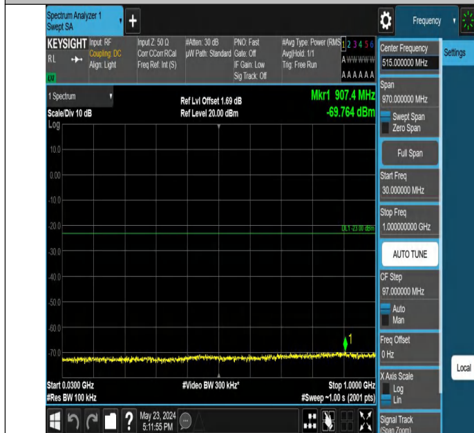
Band2_3MHz_QPSK_18900_1RB#0_30~1000_30~1000
