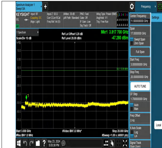
Band2_1.4MHz_QPSK_19193_1RB#0_3000~20000_3000~20000
