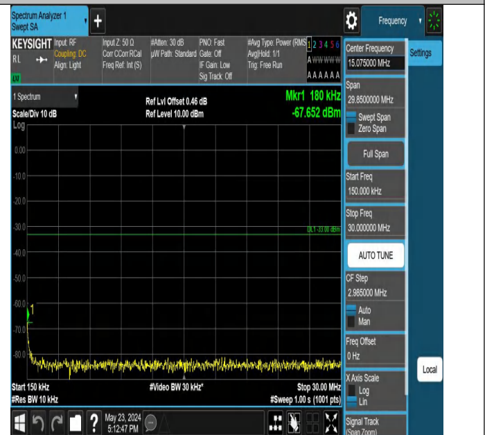
Band2_3MHz_QPSK_19185_1RB#0_0.15~30_0.15~30
