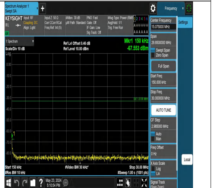
Band2_3MHz_QPSK_18615_1RB#0_0.15~30_0.15~30
