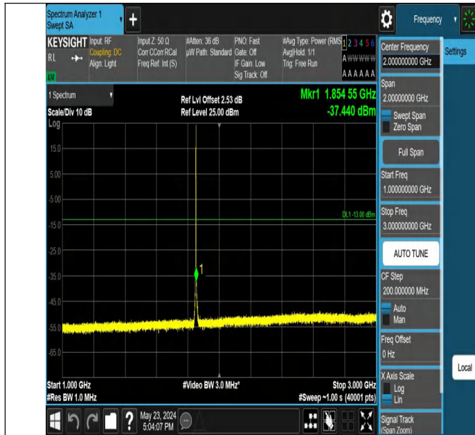
Band2_1.4MHz_QPSK_18607_1RB#5_1000~3000_1000~3000
