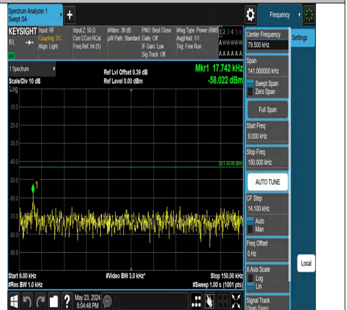
Band2_1.4MHz_QPSK_18900_1RB#5_0.009~0.15_0.009~0.15
