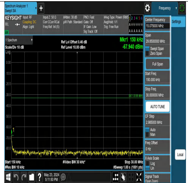
Band2_3MHz_QPSK_18900_1RB#0_0.15~30_0.15~30
