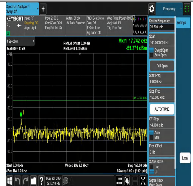
Band2_3MHz_QPSK_19185_1RB#14_0.009~0.15_0.009~0.15
