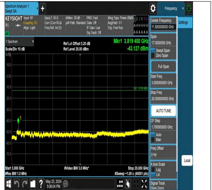
Band2_1.4MHz_QPSK_19193_1RB#5_3000~20000_3000~20000
