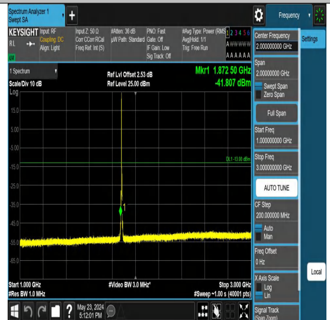
Band2_3MHz_QPSK_18900_1RB#0_1000~3000_1000~3000
