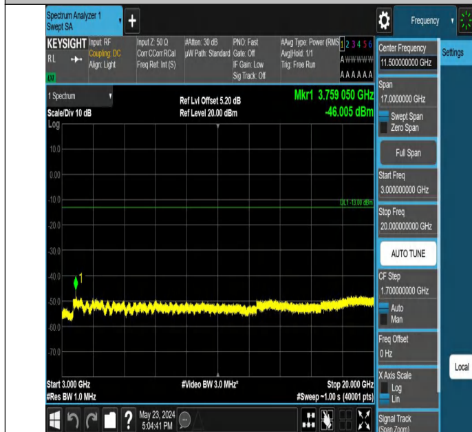
Band2_1.4MHz_QPSK_18900_1RB#0_3000~20000_3000~20000
