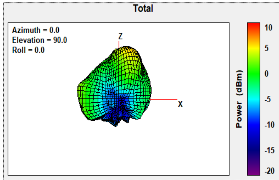
Band 1-5.200GHz X-Z plane View
