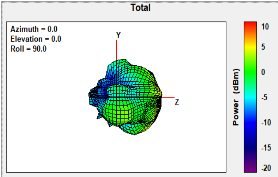
Band 4-5.800GHz Y-Z plane View
