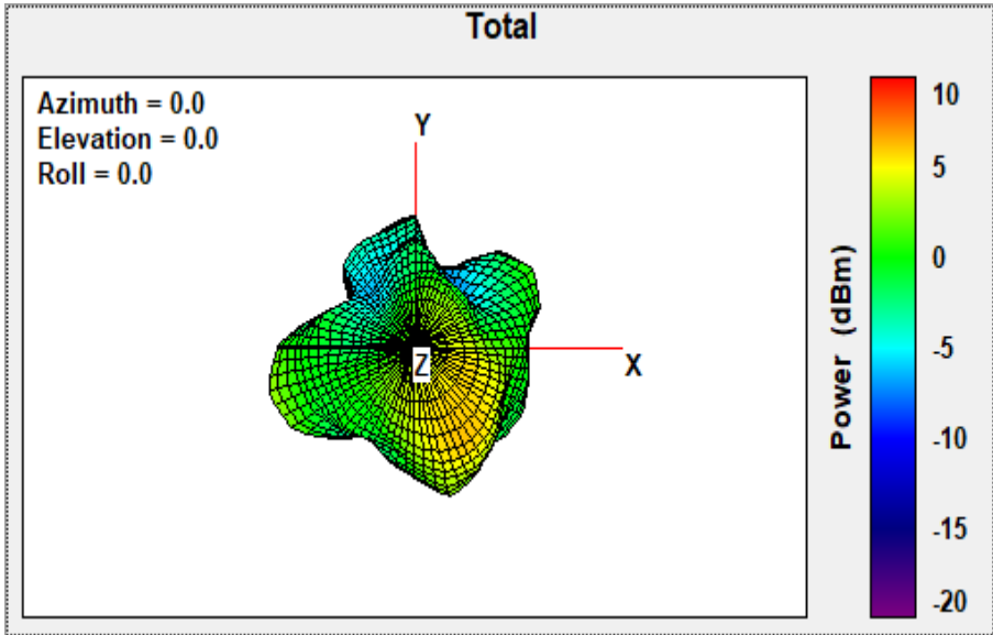
Band 1-5.200GHz X-Y plane View
