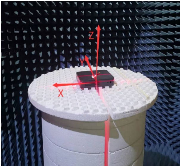
Physical object layout (with coordinate axis)
