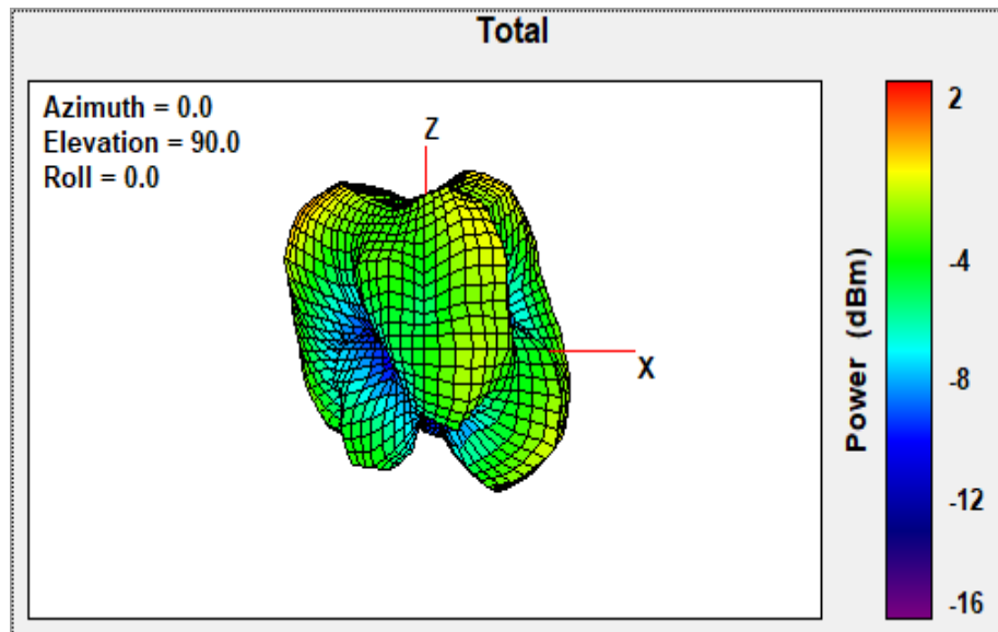
2.44GHz X-Z plane View
