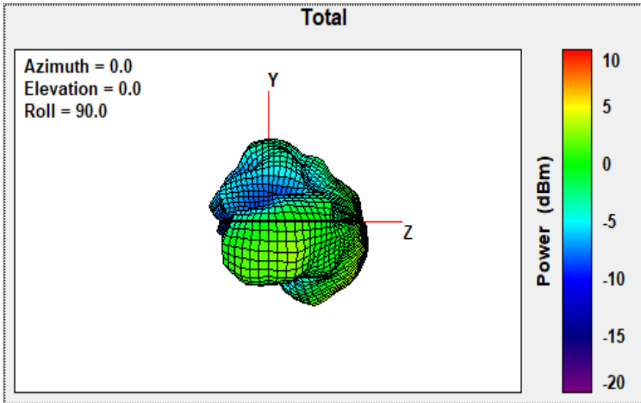
Band 1-5.200GHz Y-Z plane View
