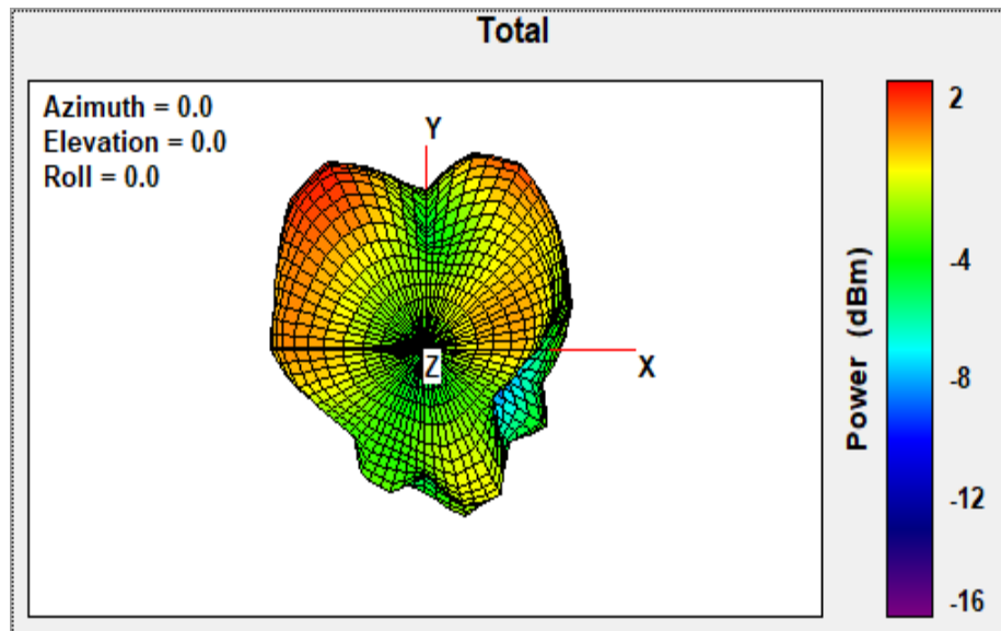
2.44GHz X-Y plane View
