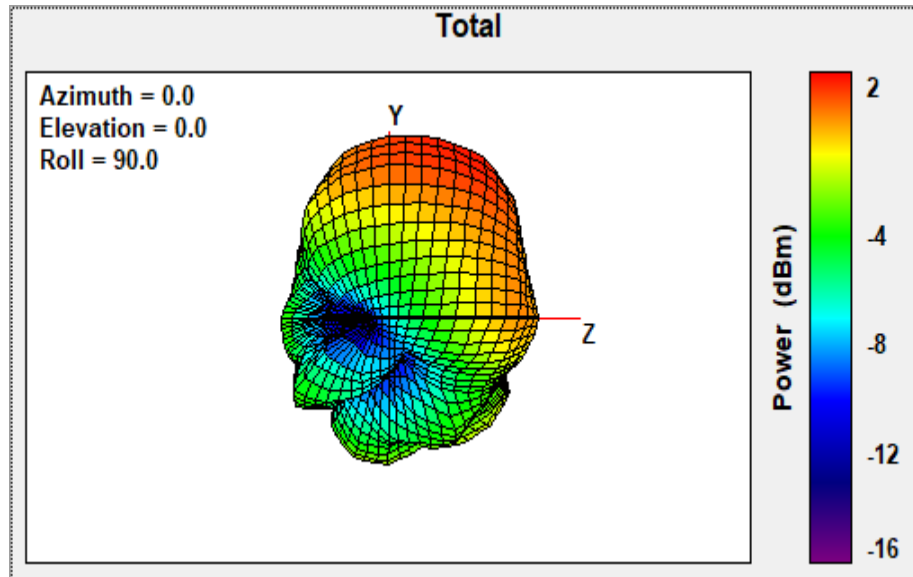
2.44GHz Y-Z plane View
