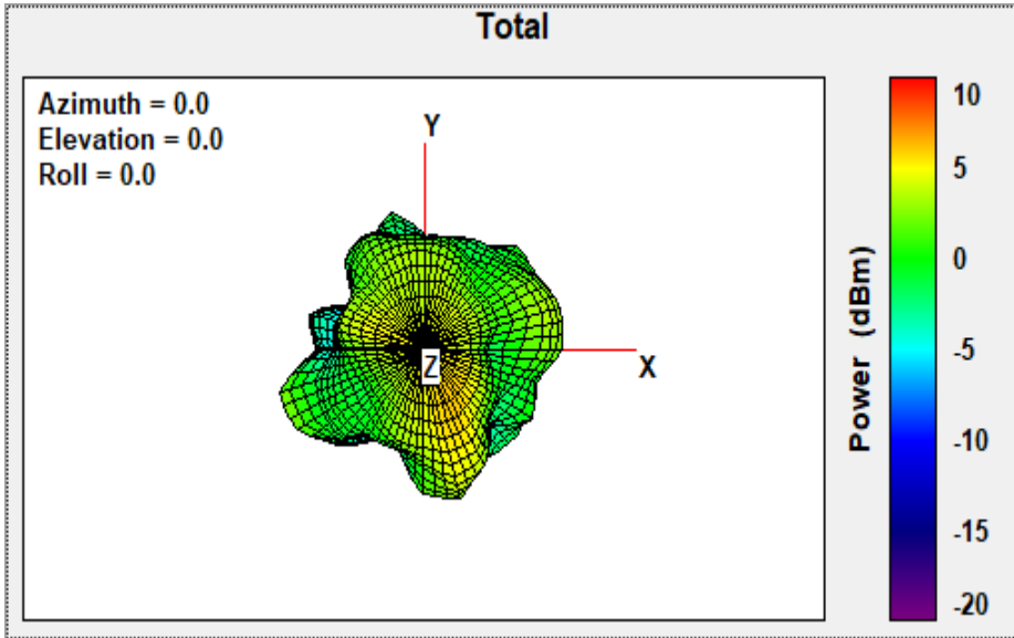
Band 4-5.800GHz X-Y plane View
