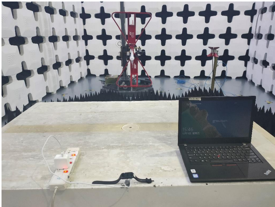
2. Radiated Emissions (Part 15B Bluetooth ,1GHz-18GHz)
