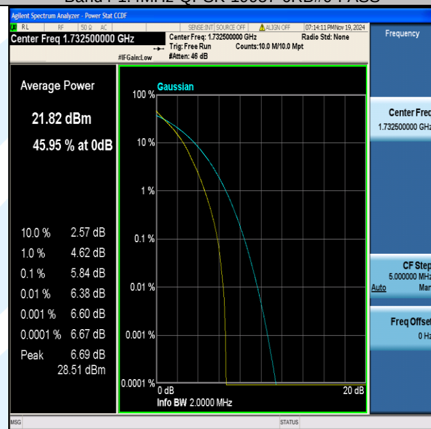
Band4-1.4MHz-QPSK-20175-6RB#0-PASS
