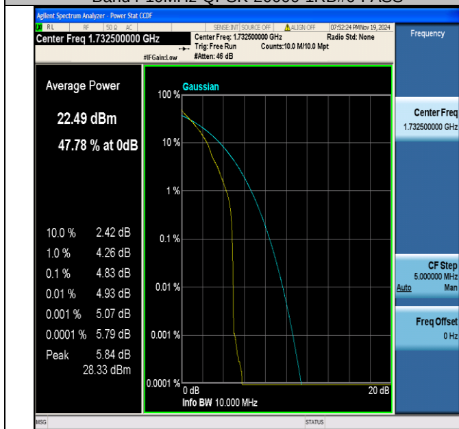
Band4-10MHz-QPSK-20175-1RB#0-PASS
