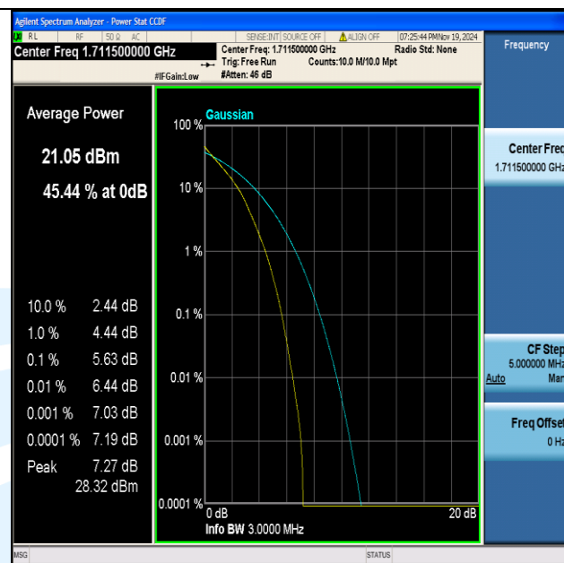
Band4-3MHz-QPSK-19965-15RB#0-PASS
