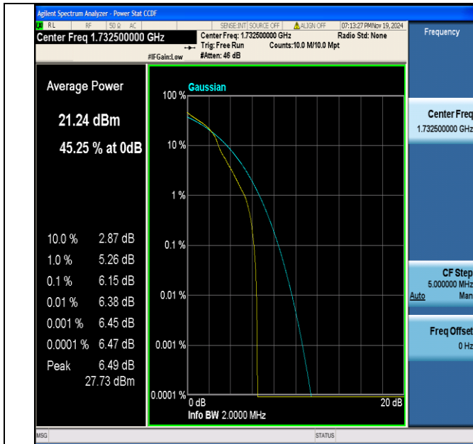
Band4-1.4MHz-16QAM-20175-1RB#0-PASS
