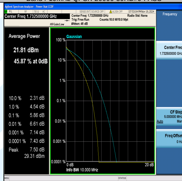
Band4-10MHz-QPSK-20175-50RB#0-PASS
