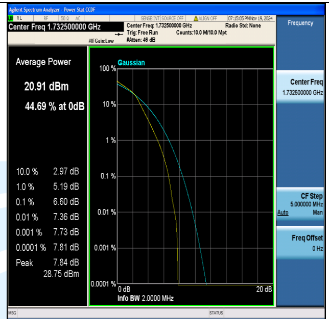
Band4-1.4MHz-16QAM-20175-6RB#0-PASS
