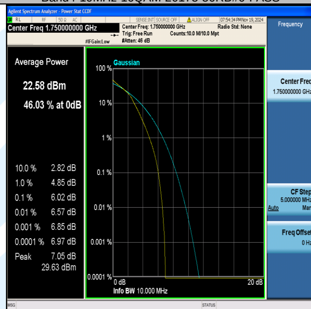
Band4-10MHz-16QAM-20350-50RB#0-PASS
