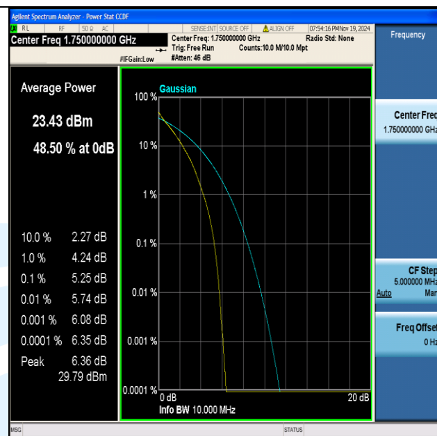
Band4-10MHz-QPSK-20350-50RB#0-PASS
