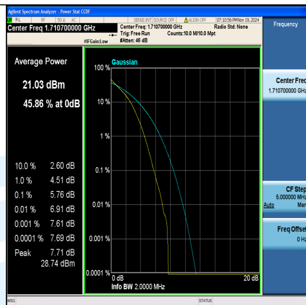
Band4-1.4MHz-QPSK-19957-6RB#0-PASS
