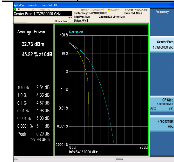
Band4-3MHz-QPSK-20175-1RB#0-PASS
