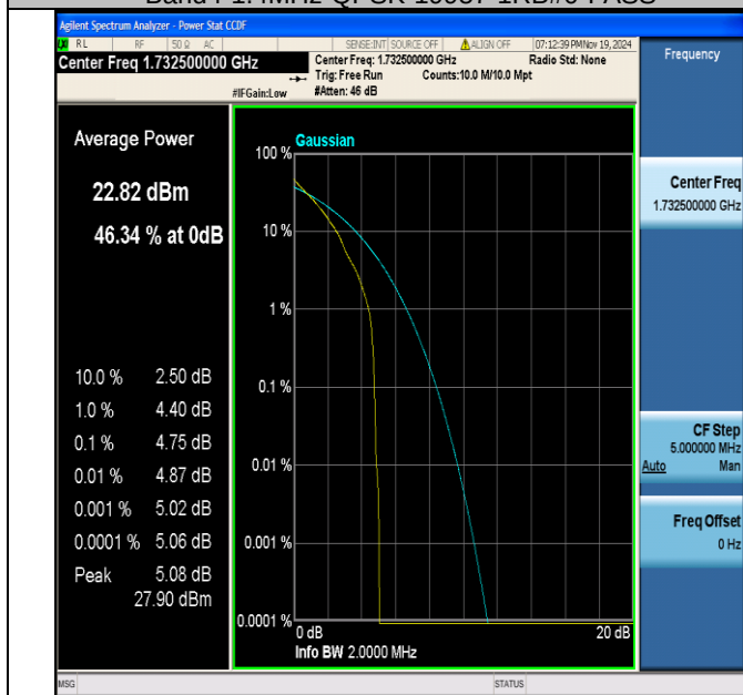
Band4-1.4MHz-QPSK-20175-1RB#0-PASS
