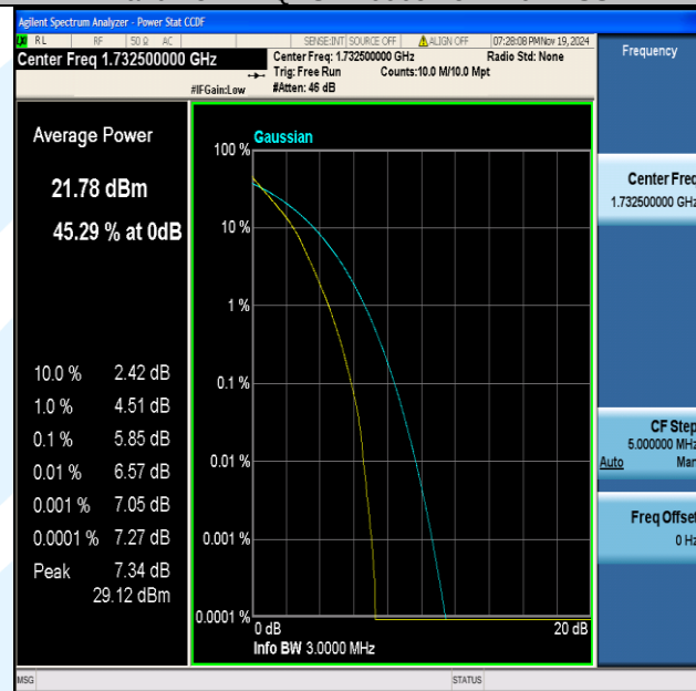
Band4-3MHz-QPSK-20175-15RB#0-PASS
