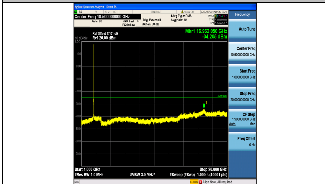
Band38_20MHz_QPSK_38150_100RB#0_1000~20000_1000~20000
