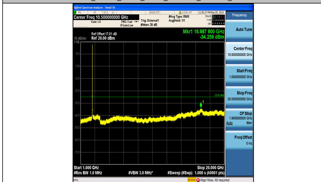
Band38_20MHz_QPSK_37850_100RB#0_1000~20000_1000~20000
