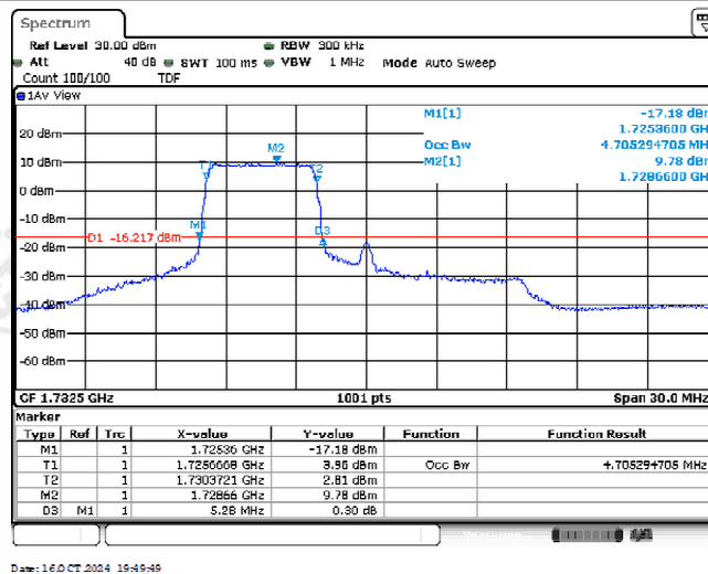
Band4-15MHz-16QAM-20175-25RB#0-4.705
