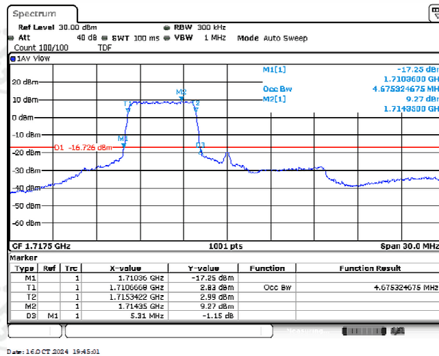
Band4-15MHz-16QAM-20025-25RB#0-4.675
