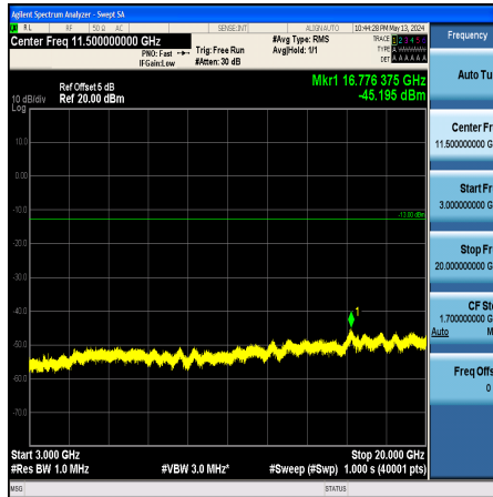
Band2_5MHz_QPSK_19175_1RB#0_3000~20000_3000~20000
