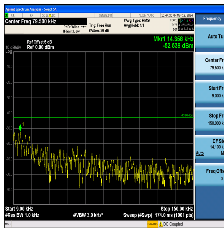
Band2_5MHz_16QAM_19175_1RB#0_0.009~0.15_0.009~0.15
