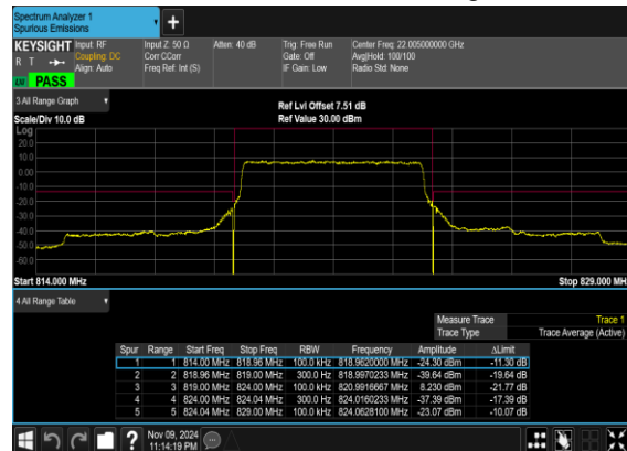
N26(5M)_DFT-s- OFDM_BPSK_Outer_Full_High_CH
