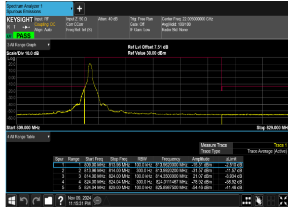
N26(10M)_DFT-s- OFDM_BPSK_Edge_1RB_Left_Mid_CH
