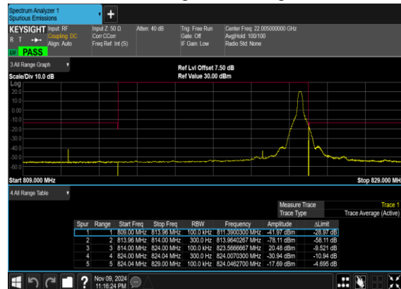
N26(10M)_DFT-s- OFDM_BPSK_Edge_1RB_Right_Mid_CH
