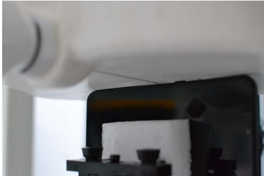
SAR Test Setup Photo 17 Left Edge 0 mm
