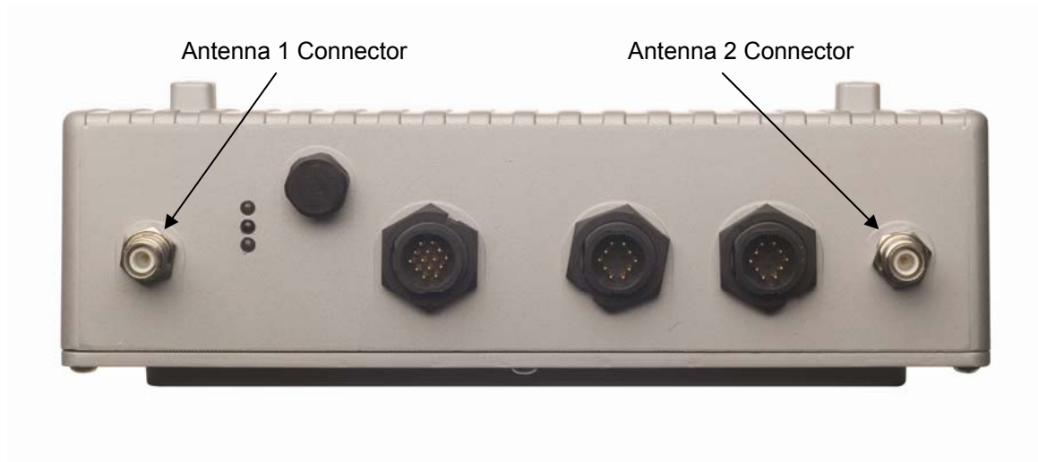
HotPort 3203 Rear/Bottom Panel
