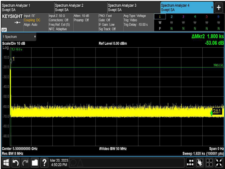
Figure 604 - 30 minute Non-Occupancy Period
