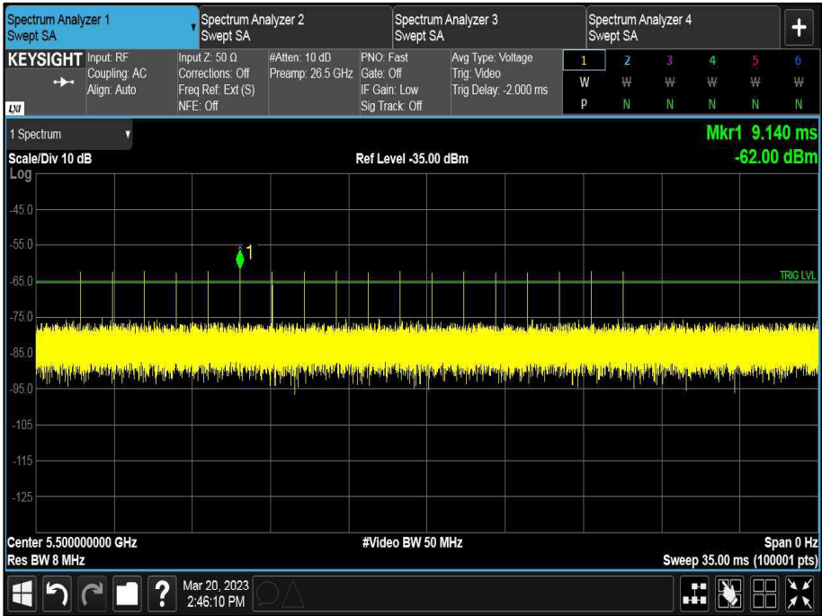
Figure 600 - Verification of Radar Type 0
