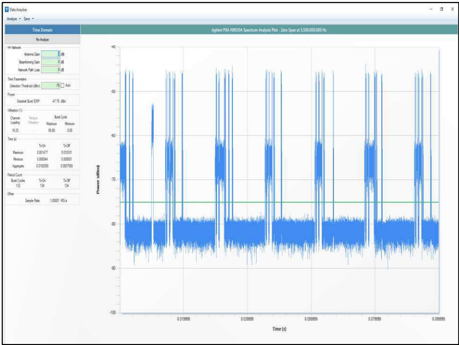
Figure 595 - Channel Loading
