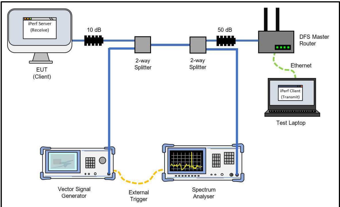
Figure 593 - Test Equipment Setup Diagram for Client without Radar Detection with Injection at the Master
