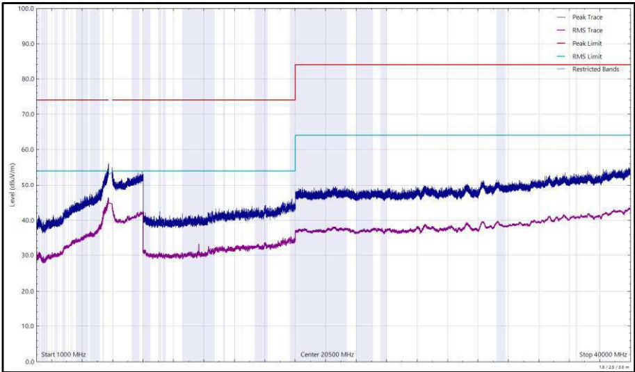
Figure 590 - U-NII-3 - 5825 MHz (CH165), VHT20, CDD, Core 0 + Core 1, 1 GHz to 40 GHz, Horizontal
