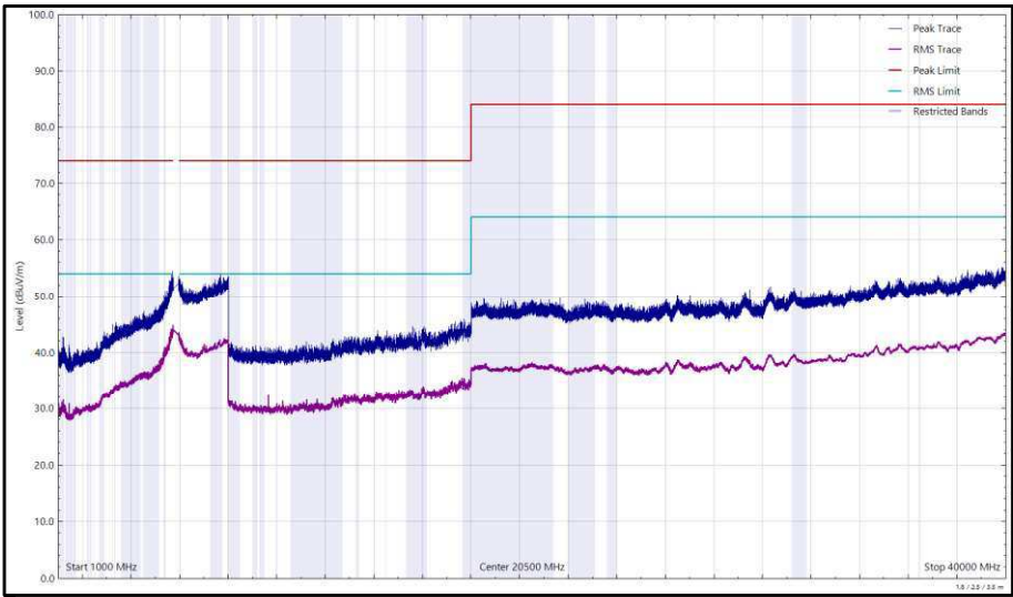
Figure 592 - U-NII-3 - 5825 MHz (CH165), VHT20, CDD, Core 0 + Core 1, 1 GHz to 40 GHz, Vertical
