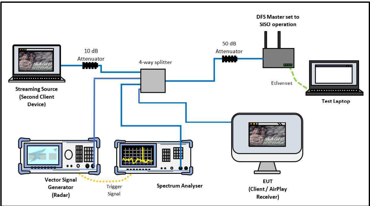
Figure 599 - Test Equipment Setup Diagram for Client without Radar Detection with Injection at the Master
