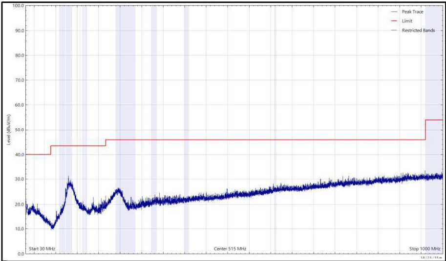
Figure 589 - U-NII-3 - 5825 MHz (CH165), VHT20, CDD, Core 0 + Core 1, 30 MHz to 1 GHz, Horizontal (Peak)
