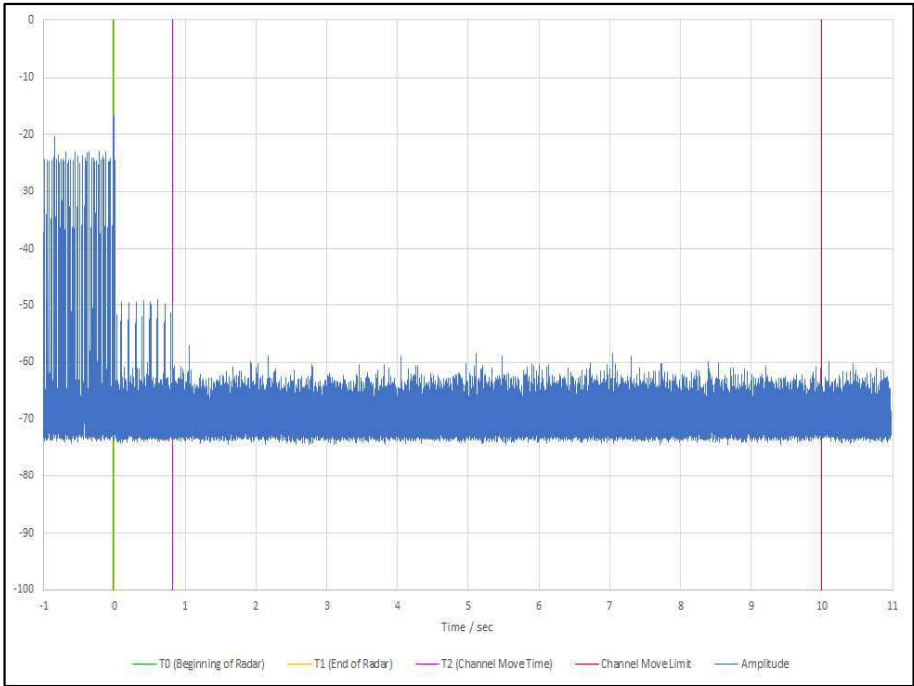
Figure 603 - First 12 s of Channel Shutdown Period
