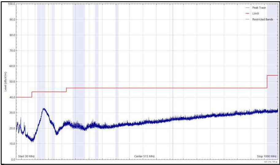
Figure 591 - U-NII-3 - 5825 MHz (CH165), VHT20, CDD, Core 0 + Core 1, 30 MHz to 1 GHz, Vertical (Peak)
