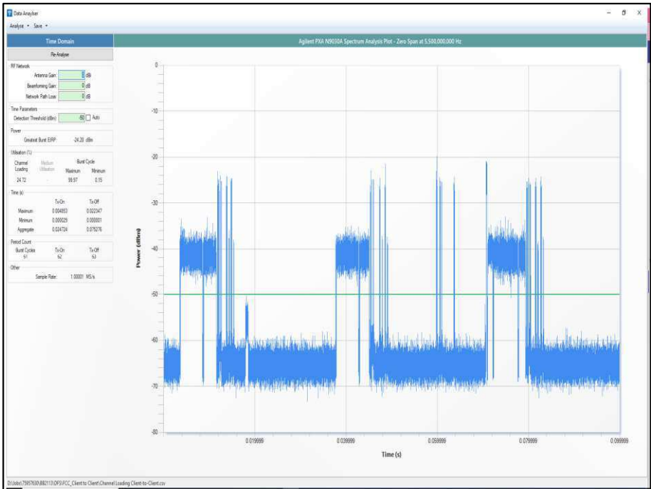
Figure 601 - Channel Loading
