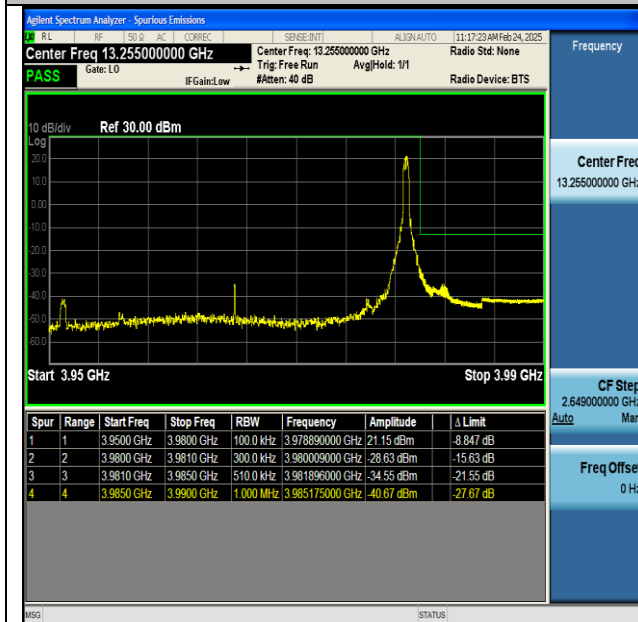
NTNV-n77(3700-3980)-PC2-30-30-H-CP-QPSK- Edge_1RB_Right-PASS
