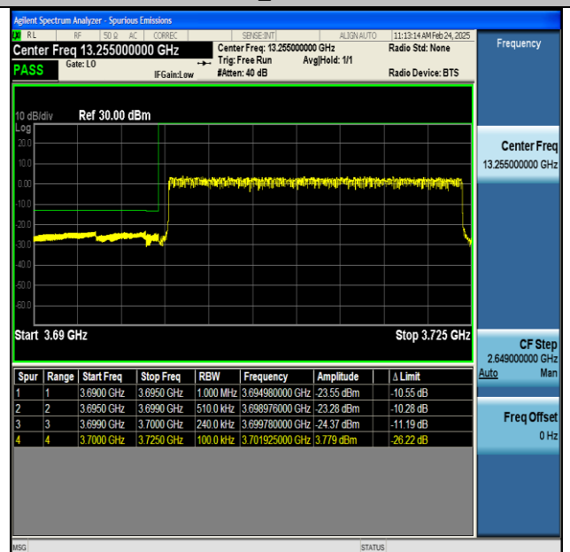
NTNV-n77(3700-3980)-PC2-30-25-L-CP-QPSK- Outer_Full-PASS
