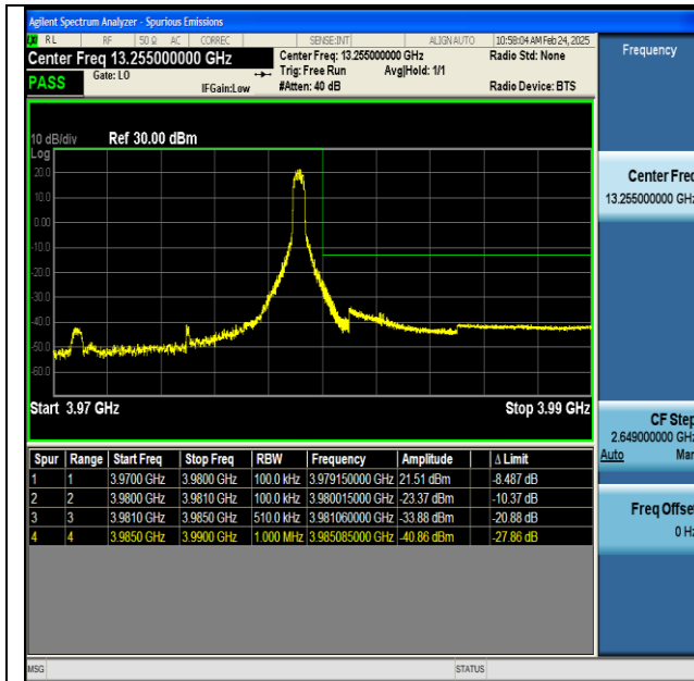
NTNV-n77(3700-3980)-PC2-30-10-H-DFT-BPSK- Edge_1RB_Right-PASS
