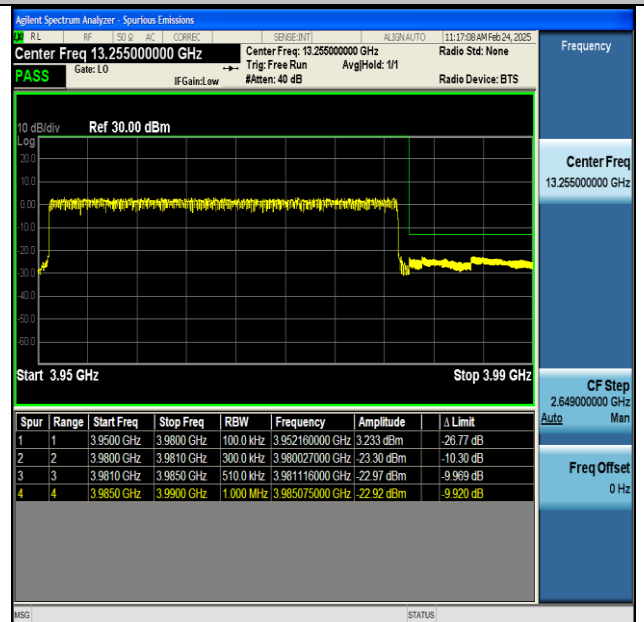
NTNV-n77(3700-3980)-PC2-30-30-H-CP-QPSK- Outer_Full-PASS
