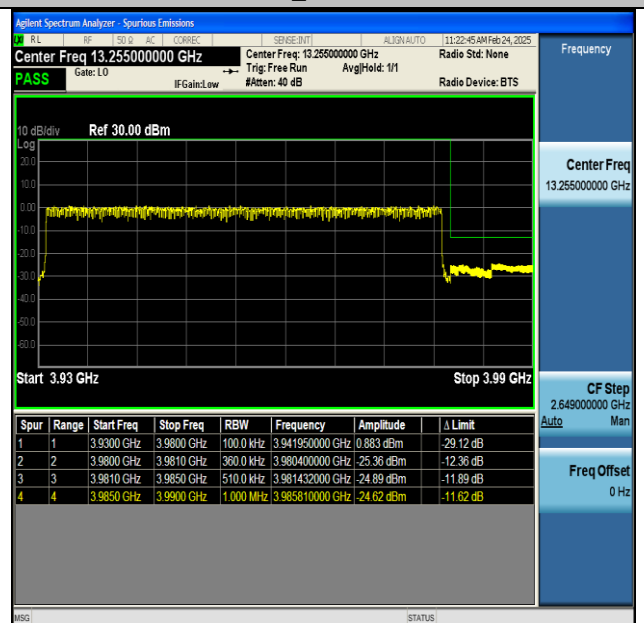
NTNV-n77(3700-3980)-PC2-30-50-H-CP-QPSK- Outer_Full-PASS
