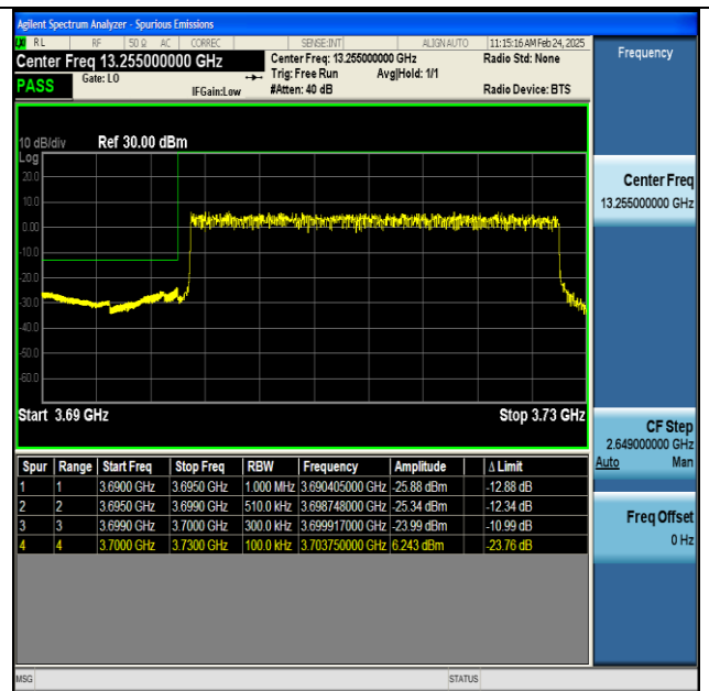
NTNV-n77(3700-3980)-PC2-30-30-L-DFT-BPSK- Outer_Full-PASS
