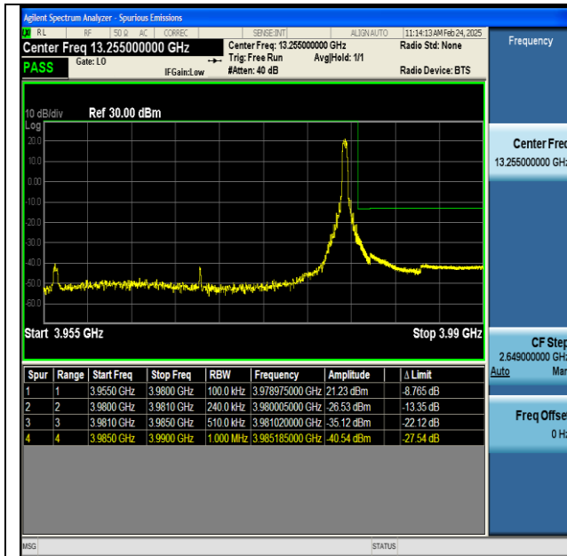
NTNV-n77(3700-3980)-PC2-30-25-H-DFT-BPSK- Edge_1RB_Right-PASS
