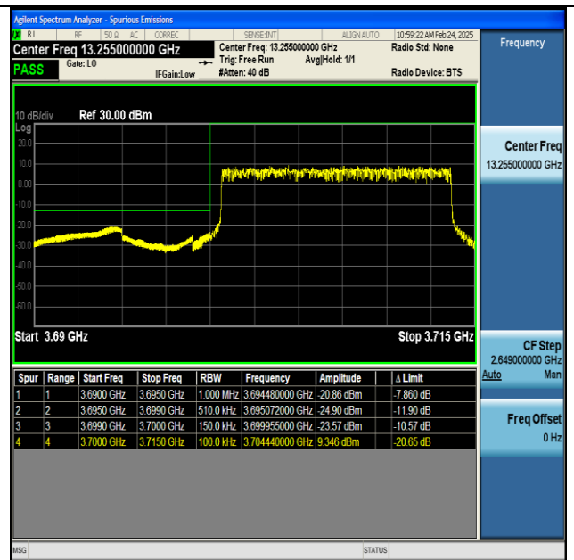
NTNV-n77(3700-3980)-PC2-30-15-L-DFT-BPSK- Outer_Full-PASS
