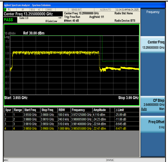
NTNV-n77(3700-3980)-PC2-30-25-H-CP-QPSK- Outer_Full-PASS
