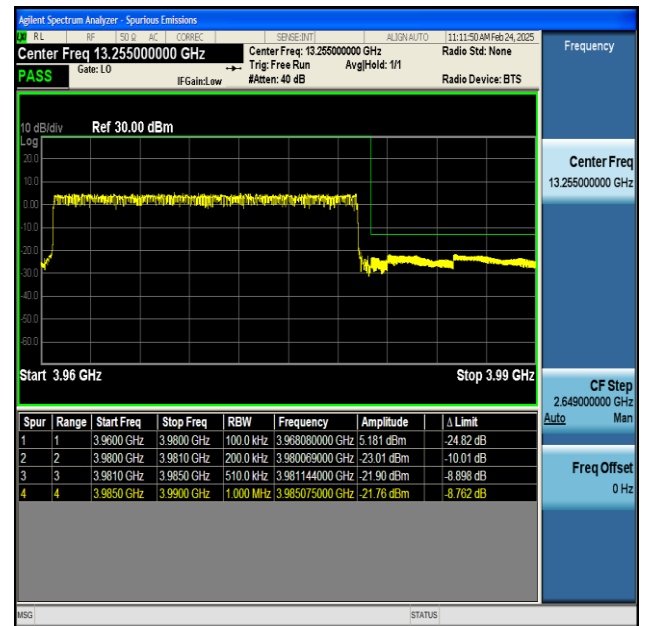
NTNV-n77(3700-3980)-PC2-30-20-H-CP-QPSK- Outer_Full-PASS
