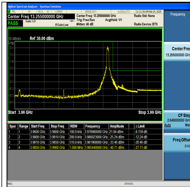
NTNV-n77(3700-3980)-PC2-30-20-H-DFT-BPSK- Edge_1RB_Right-PASS
