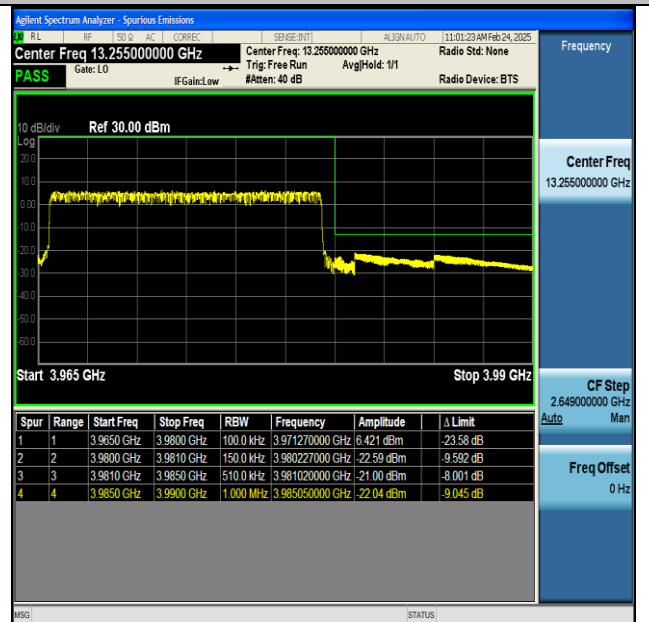
NTNV-n77(3700-3980)-PC2-30-15-H-CP-QPSK- Outer_Full-PASS
