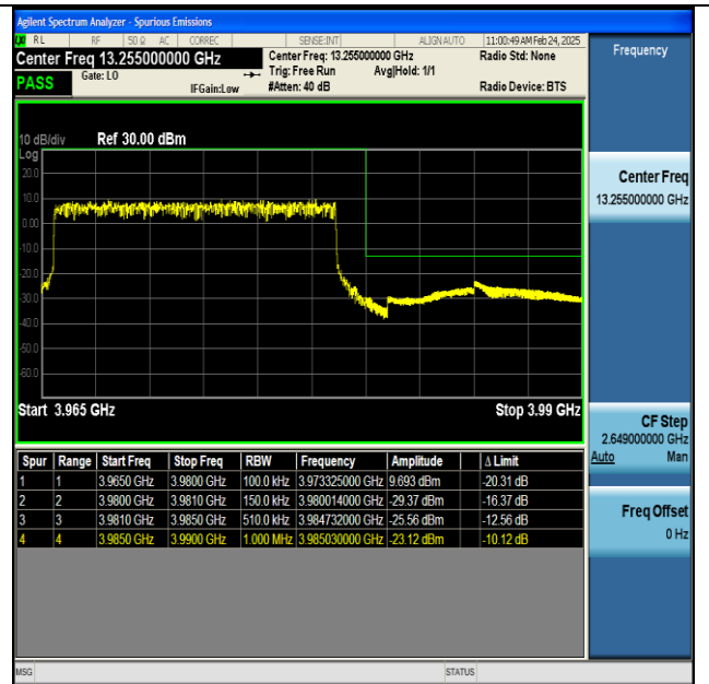
NTNV-n77(3700-3980)-PC2-30-15-H-DFT-BPSK- Outer_Full-PASS
