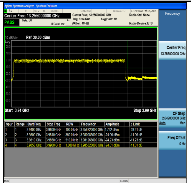
NTNV-n77(3700-3980)-PC2-30-40-H-CP-QPSK- Outer_Full-PASS
