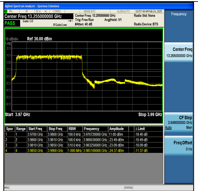
NTNV-n77(3700-3980)-PC2-30-10-H-DFT-BPSK- Outer_Full-PASS
