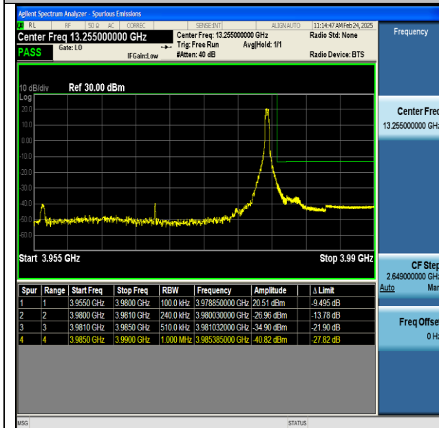
NTNV-n77(3700-3980)-PC2-30-25-H-CP-QPSK- Edge_1RB_Right-PASS
