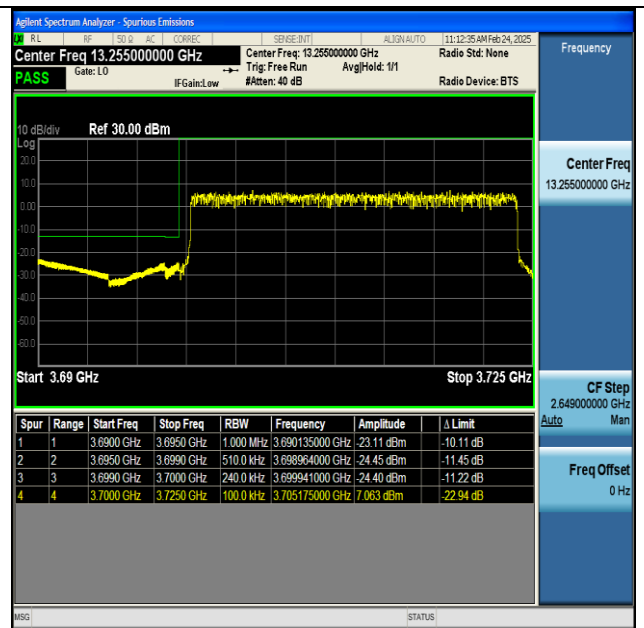
NTNV-n77(3700-3980)-PC2-30-25-L-DFT-BPSK- Outer_Full-PASS
