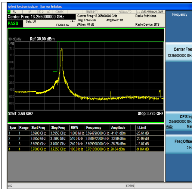
NTNV-n77(3700-3980)-PC2-30-25-L-DFT-BPSK- Edge_1RB_Left-PASS
