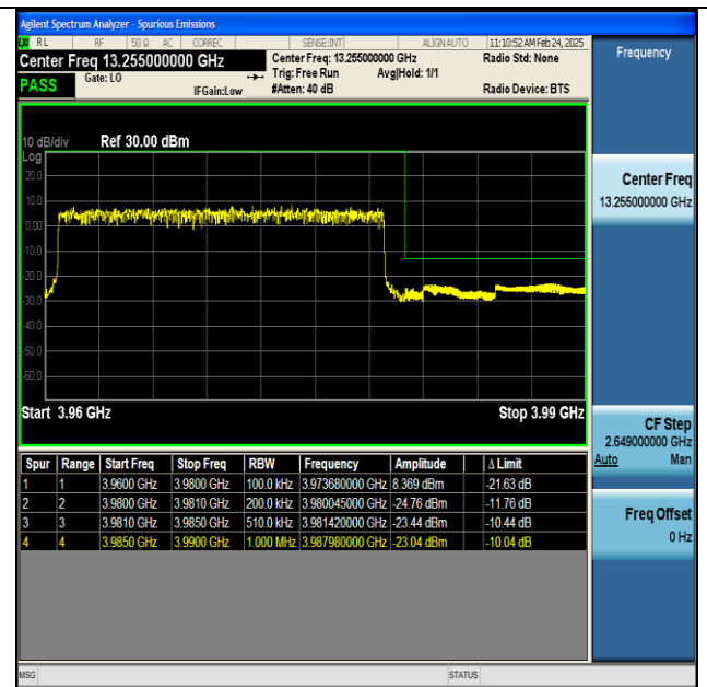
NTNV-n77(3700-3980)-PC2-30-20-H-DFT-BPSK- Outer_Full-PASS
