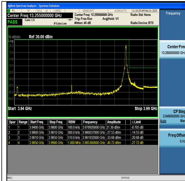
NTNV-n77(3700-3980)-PC2-30-40-H-DFT-BPSK- Edge_1RB_Right-PASS
