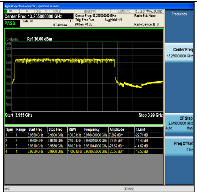
NTNV-n77(3700-3980)-PC2-30-25-H-DFT-BPSK- Outer_Full-PASS
