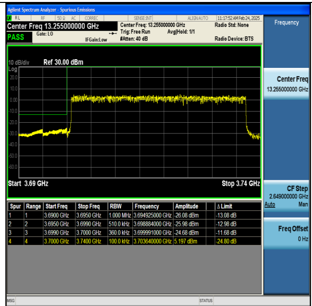
NTNV-n77(3700-3980)-PC2-30-40-L-DFT-BPSK- Outer_Full-PASS
