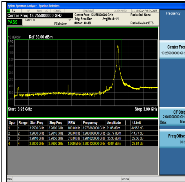
NTNV-n77(3700-3980)-PC2-30-30-H-DFT-BPSK- Edge_1RB_Right-PASS
