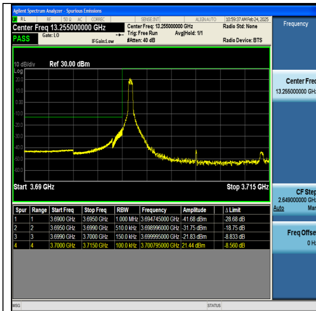
NTNV-n77(3700-3980)-PC2-30-15-L-DFT-BPSK- Edge_1RB_Left-PASS
