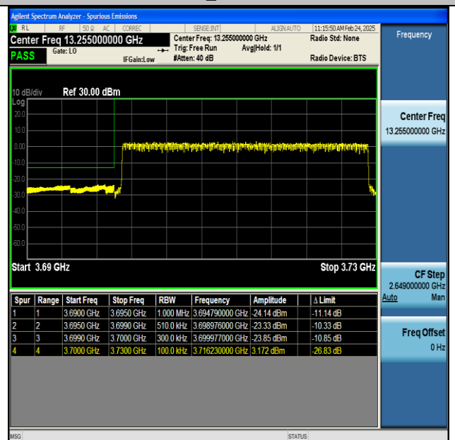
NTNV-n77(3700-3980)-PC2-30-30-L-CP-QPSK- Outer_Full-PASS
