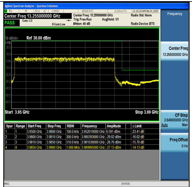
NTNV-n77(3700-3980)-PC2-30-30-H-DFT-BPSK- Outer_Full-PASS
