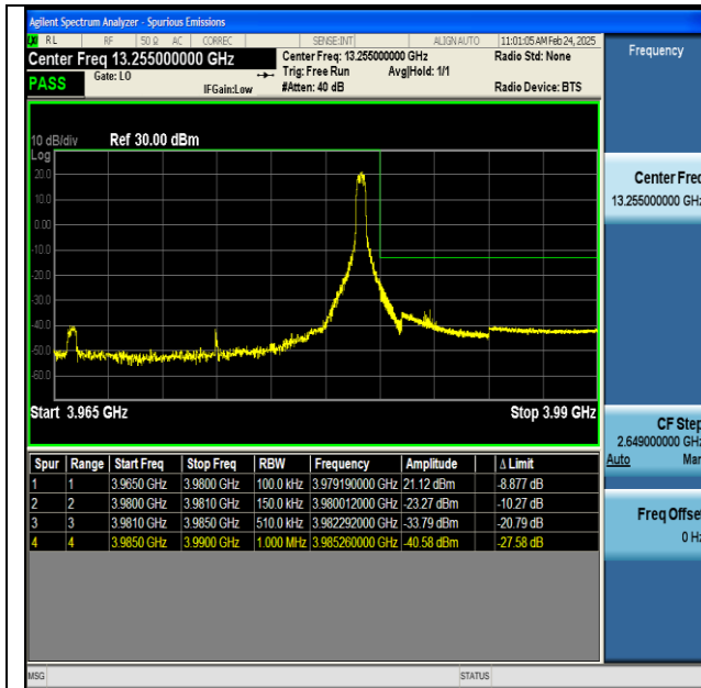
NTNV-n77(3700-3980)-PC2-30-15-H-DFT-BPSK- Edge_1RB_Right-PASS
