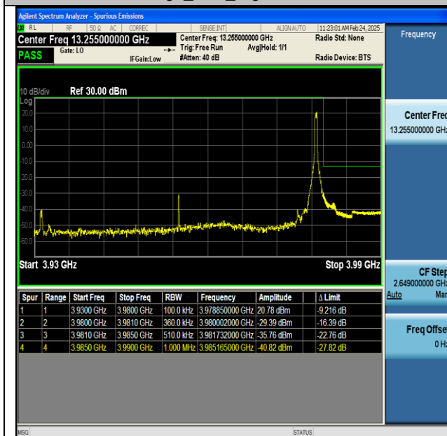
NTNV-n77(3700-3980)-PC2-30-50-H-CP-QPSK- Edge_1RB_Right-PASS
