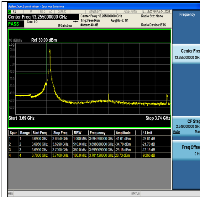
NTNV-n77(3700-3980)-PC2-30-40-L-DFT-BPSK- Edge_1RB_Left-PASS
