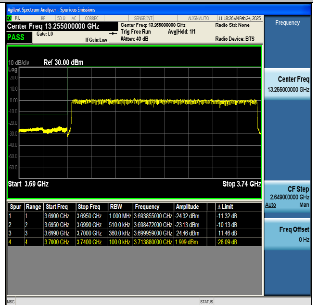
NTNV-n77(3700-3980)-PC2-30-40-L-CP-QPSK- Outer_Full-PASS
