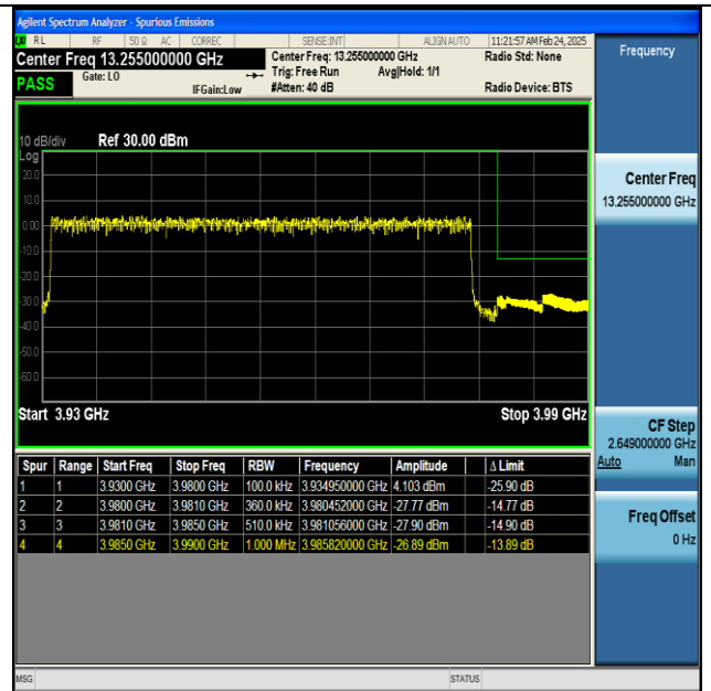
NTNV-n77(3700-3980)-PC2-30-50-H-DFT-BPSK- Outer_Full-PASS
