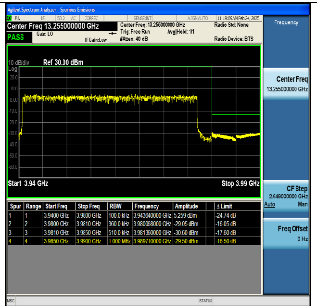
NTNV-n77(3700-3980)-PC2-30-40-H-DFT-BPSK- Outer_Full-PASS
