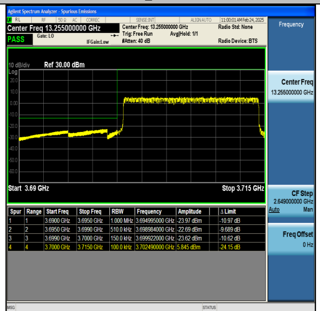
NTNV-n77(3700-3980)-PC2-30-15-L-CP-QPSK- Outer_Full-PASS
