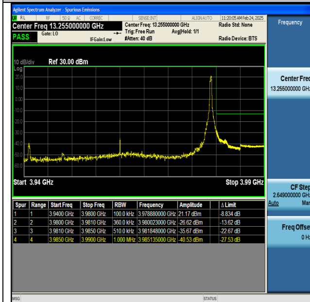
NTNV-n77(3700-3980)-PC2-30-40-H-CP-QPSK- Edge_1RB_Right-PASS
