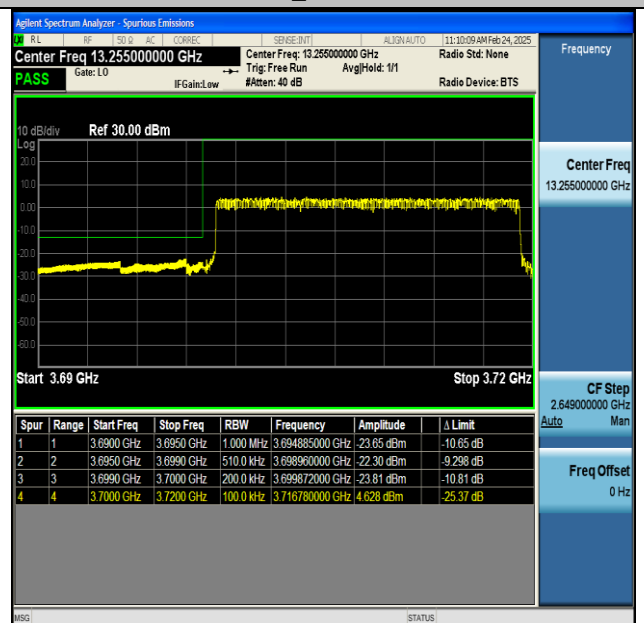
NTNV-n77(3700-3980)-PC2-30-20-L-CP-QPSK- Outer_Full-PASS
