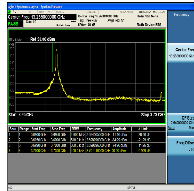
NTNV-n77(3700-3980)-PC2-30-30-L-DFT-BPSK- Edge_1RB_Left-PASS
