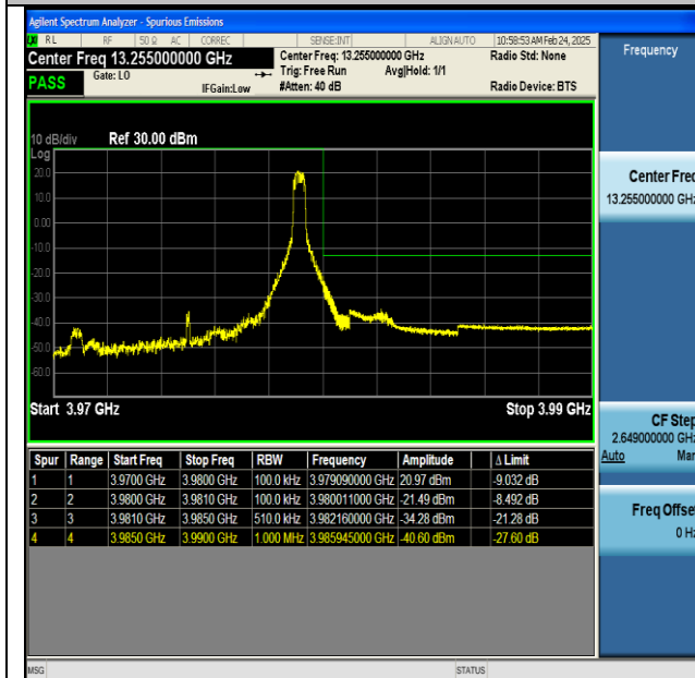
NTNV-n77(3700-3980)-PC2-30-10-H-CP-QPSK- Edge_1RB_Right-PASS
