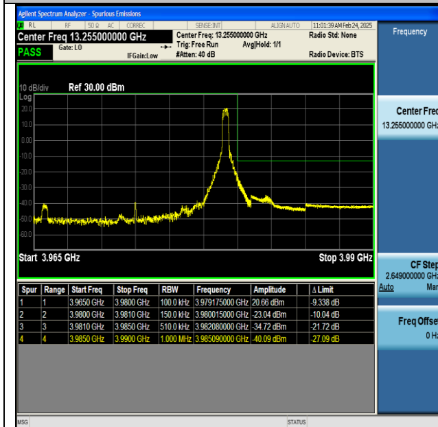
NTNV-n77(3700-3980)-PC2-30-15-H-CP-QPSK- Edge_1RB_Right-PASS
