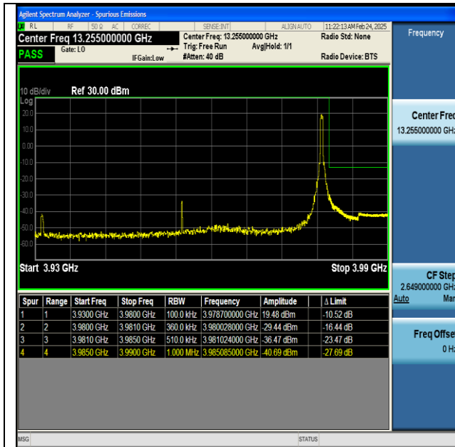
NTNV-n77(3700-3980)-PC2-30-50-H-DFT-BPSK- Edge_1RB_Right-PASS
