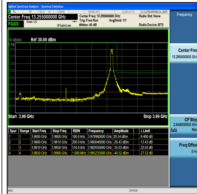
NTNV-n77(3700-3980)-PC2-30-20-H-CP-QPSK- Edge_1RB_Right-PASS
