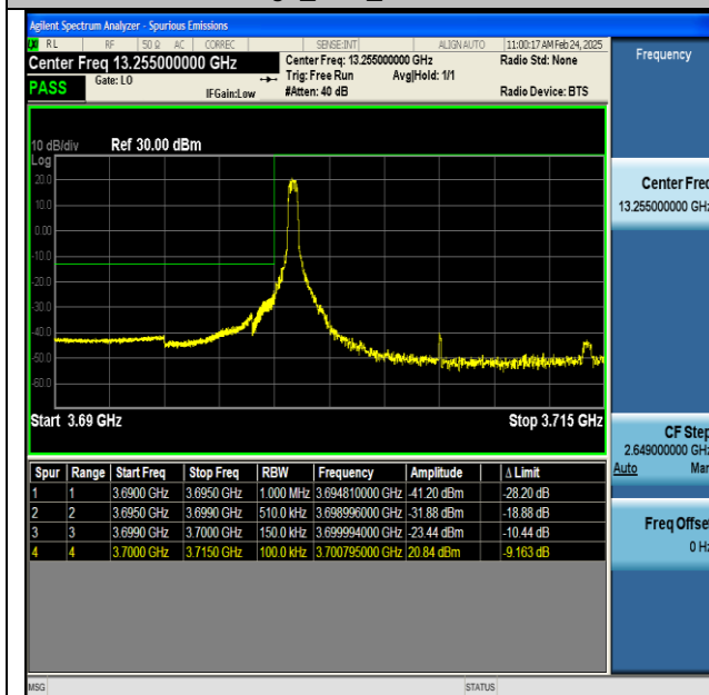
NTNV-n77(3700-3980)-PC2-30-15-L-CP-QPSK- Edge_1RB_Left-PASS
