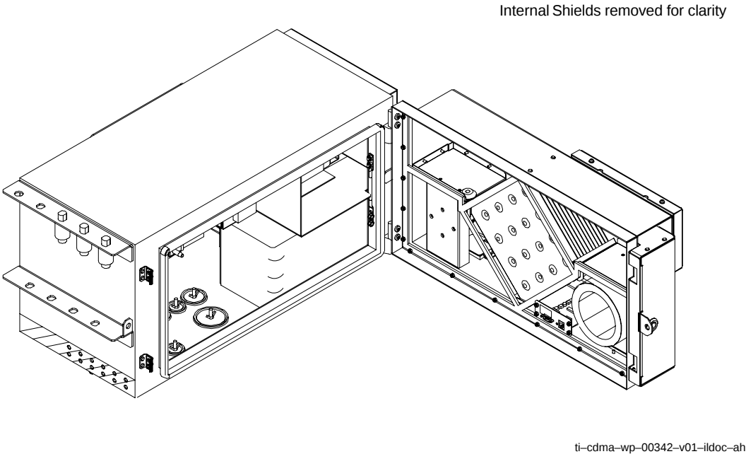
Figure 4-29: PDE and Heat Exchanger
