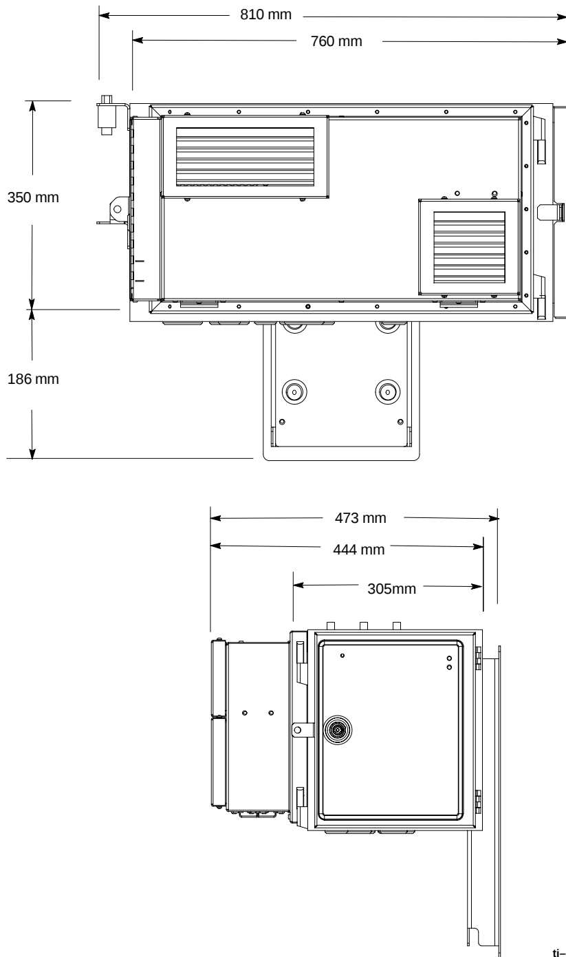
Figure 2-12: PDE Overall Dimensions
