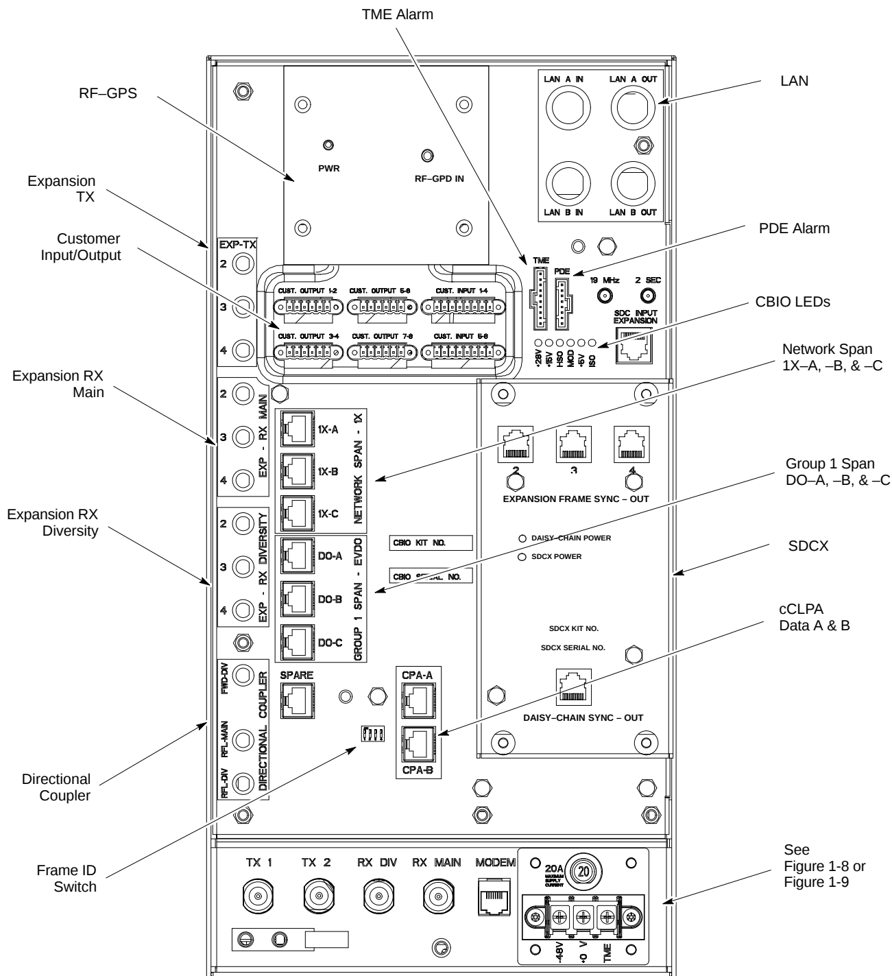
Figure 1-7: CBIO Board
