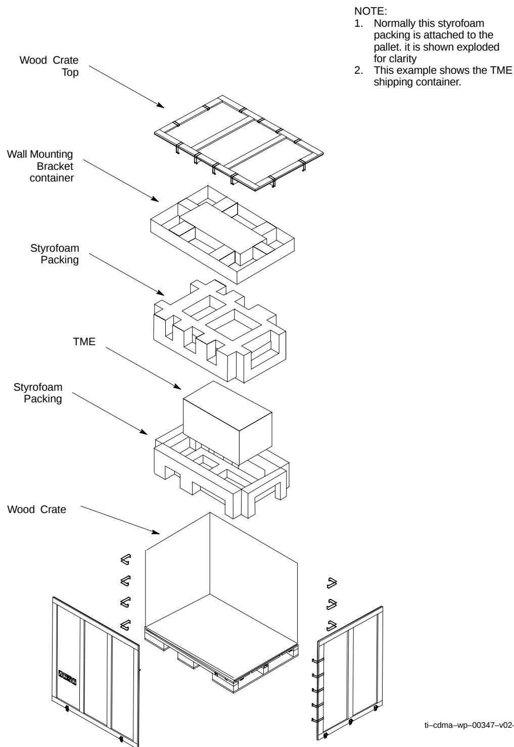
Figure 2-2: Wood Shipping Container
