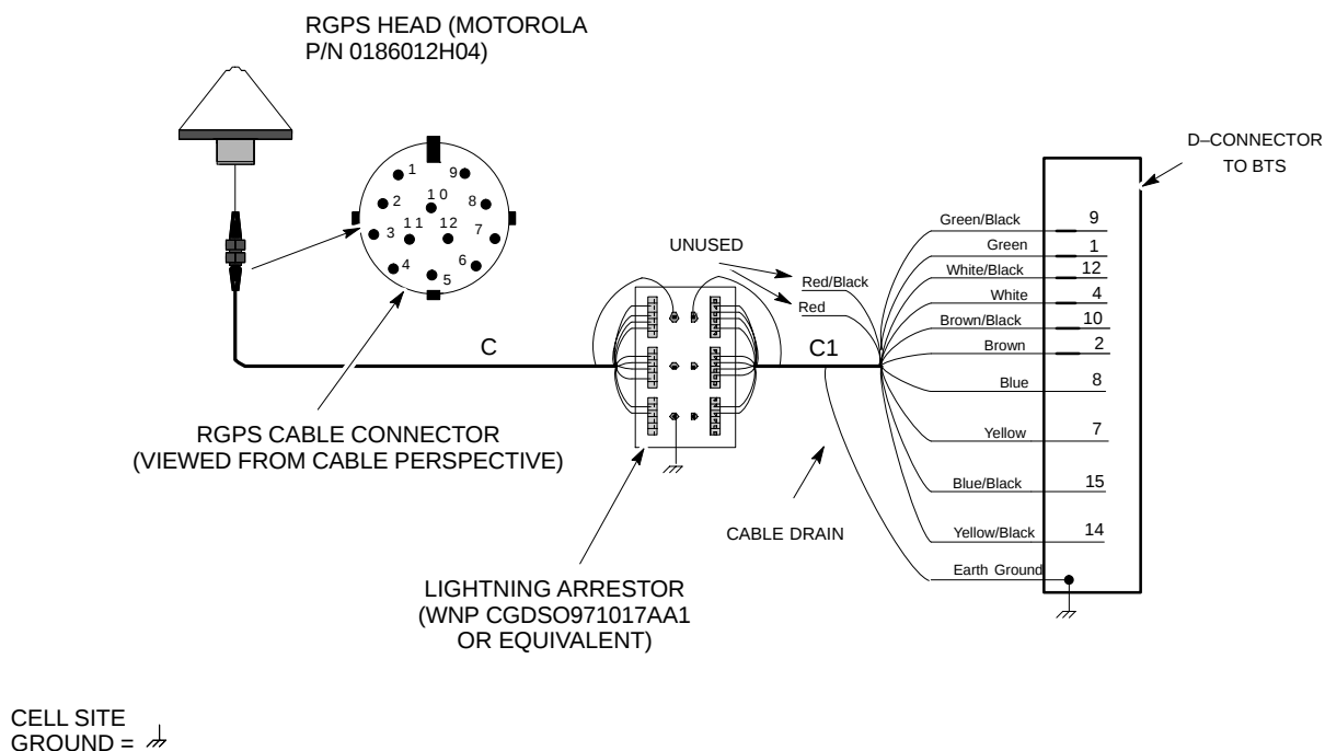
Figure 4-45: RGPS to SC480 Connection Diagram
