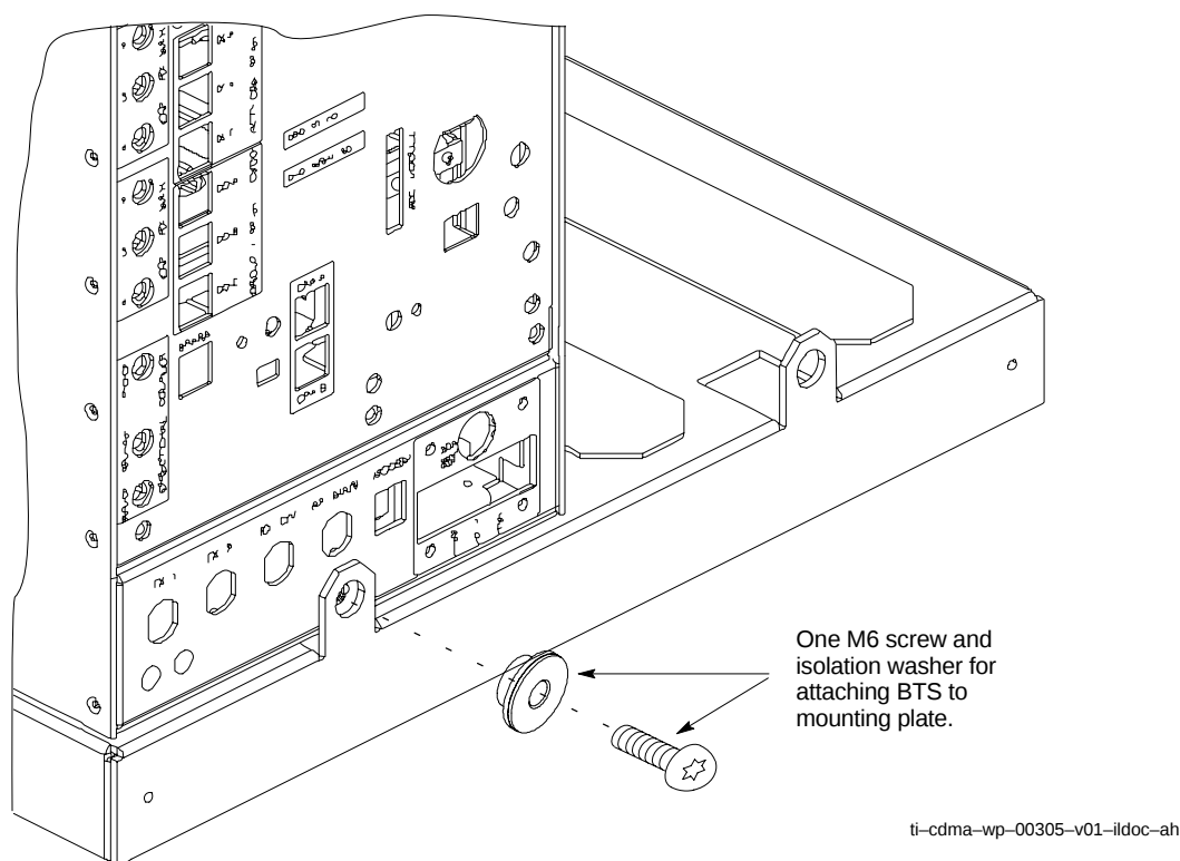
Figure 4-6: BTS Rear Attachment
