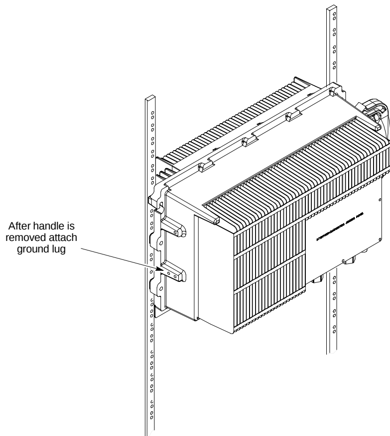
Figure 4-9: cCLPA Grounding
