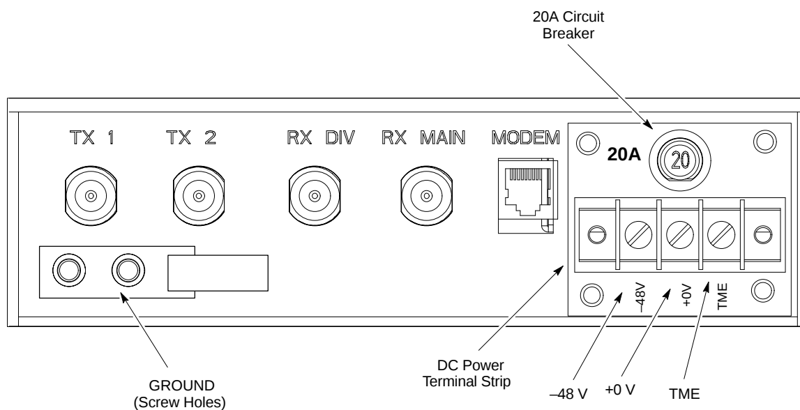
Figure 1-8: –48 VDC RF Connectors, Circuit Breaker, DC Power Terminal Strip, and Ground Studs
