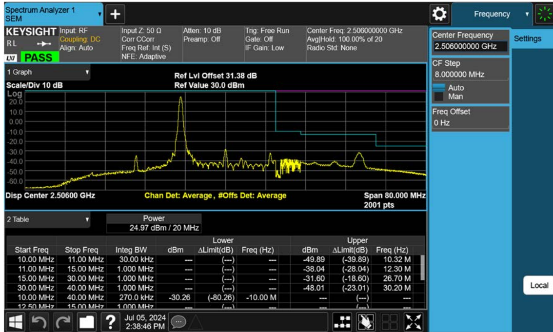
LTE B41_20 M_Channel Edge_Upper_Low_QPSK_1RB
