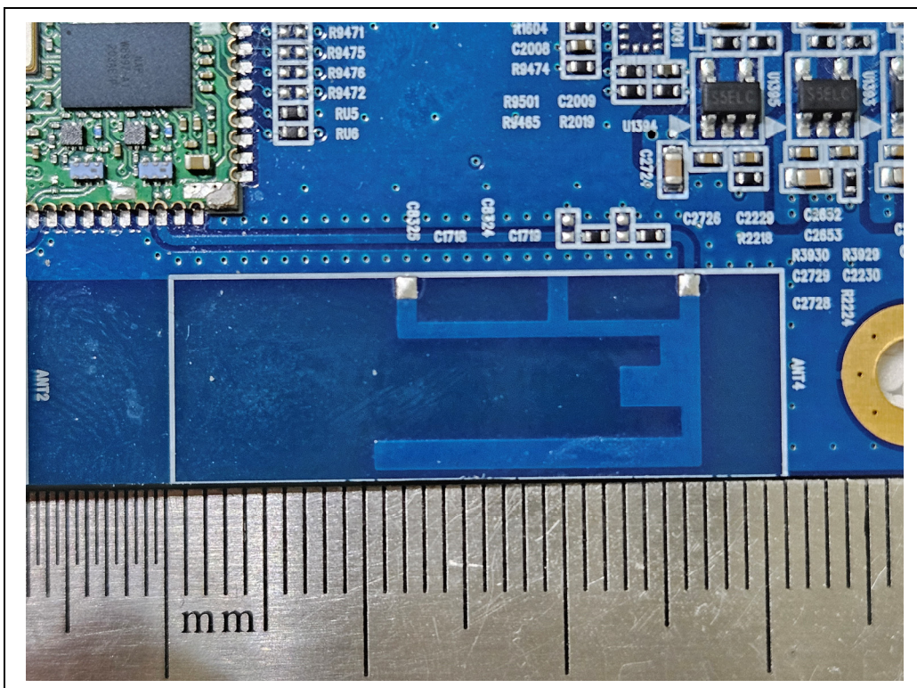
<WLAN Antenna 2>
