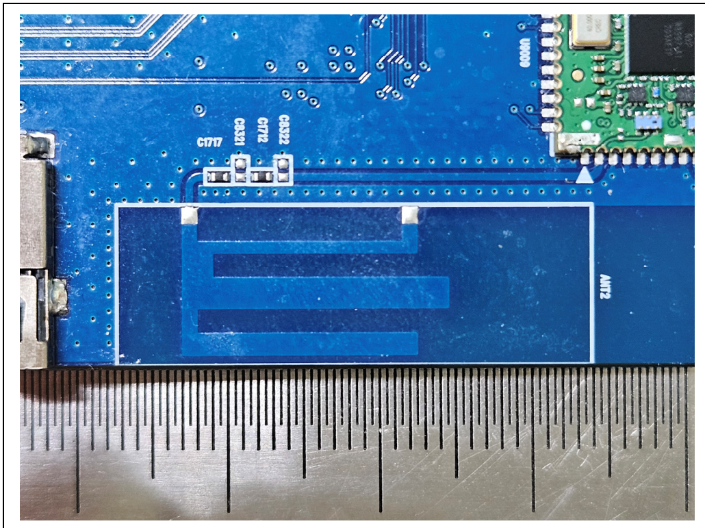
<WLAN Antenna 1>
