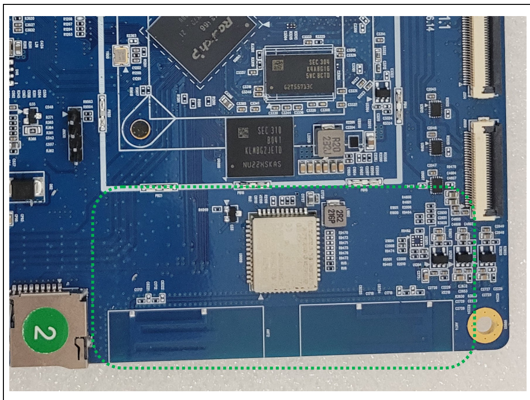
<WLAN Module and antennas>
