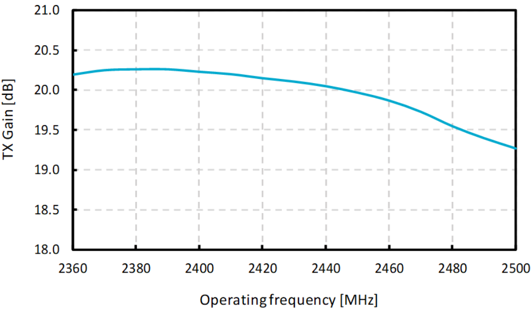
Figure 10: TX gain over operating frequency
