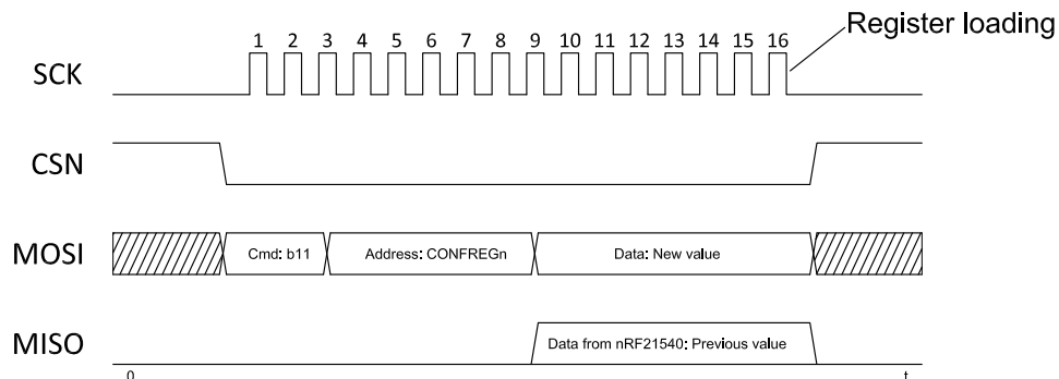
Figure 7: SPI write configuration example
