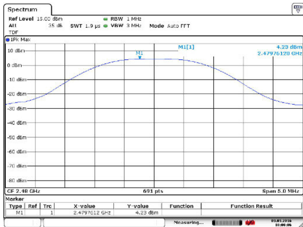
Figure 4. Maximum peak output power channel high.
