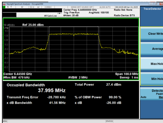
Plot 7-70. 26dB & 99% Bandwidth Plot Antenna WF2a (40MHz 802.11ax RU484 (UNII Band 6) – Ch. 99)
