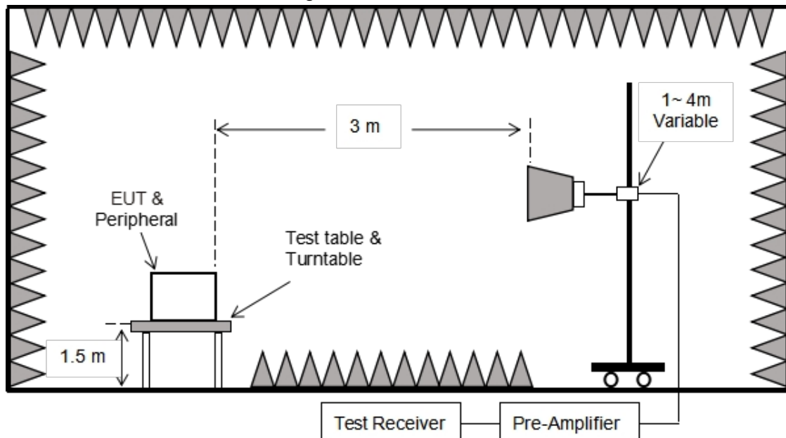
Figure 3. Above 1 GHz
