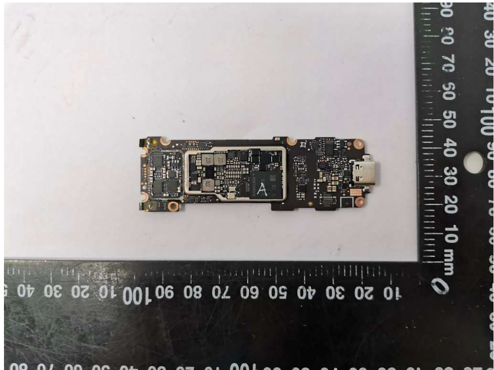
Fig.9 Mainboard view-02
