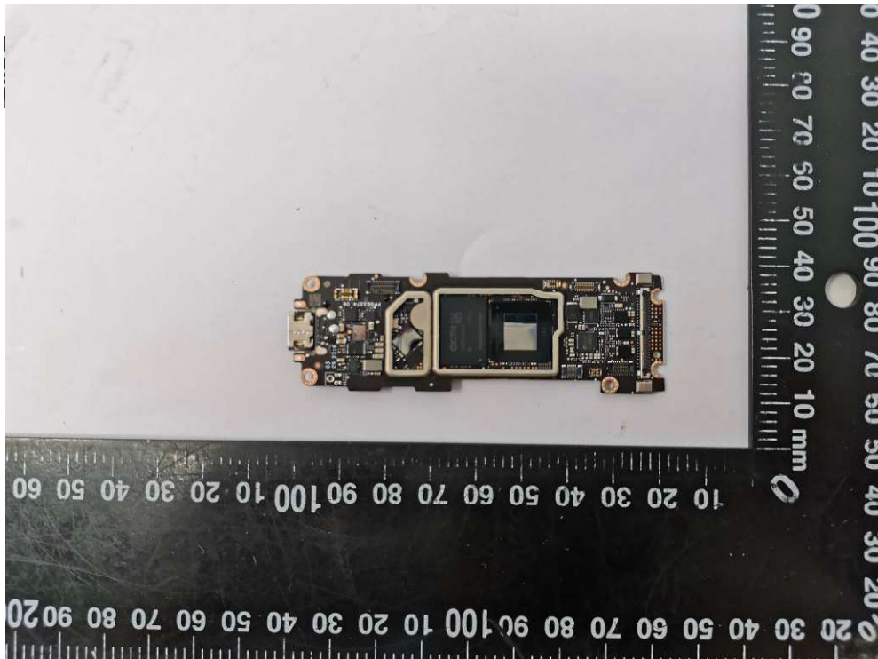
Fig.8 Mainboard view-01
