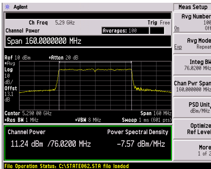
Antenna C
