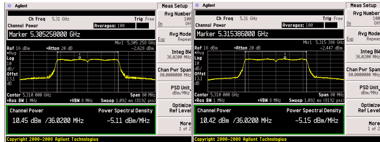
Antenna C
