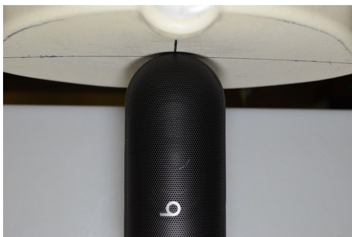
SAR Test Setup Photo 5: Body. Right Edge SAR at 0.0 cm
