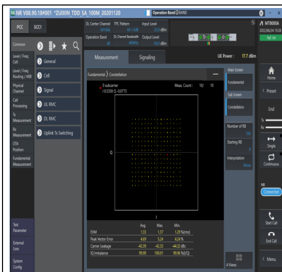
1-N48-PC3-30-40-M-9-CP-256QAM-Outer_Full-106@0-Ant1-see graph-PASS
