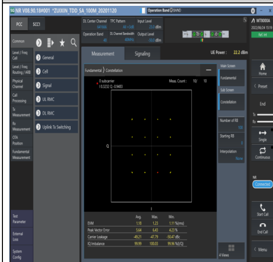
1-N48-PC3-30-40-M-3-DFT-16QAM-Outer_Full-100@0-Ant1-see graph-PASS
