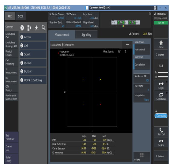
1-N48-PC3-30-40-M-2-DFT-QPSK-Outer_Full-100@0-Ant1-see graph-PASS
