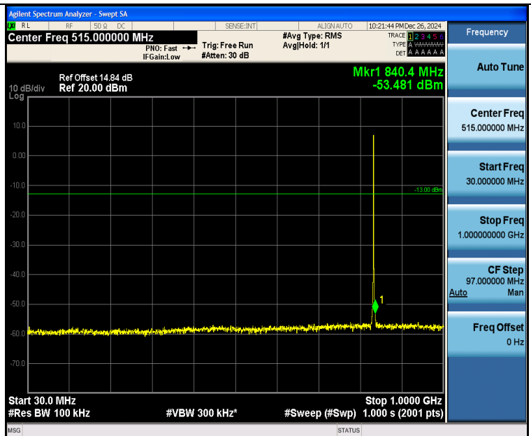
Band26 1.4MHz 16QAM 26915 6RB#0 30~1000 30~1000
