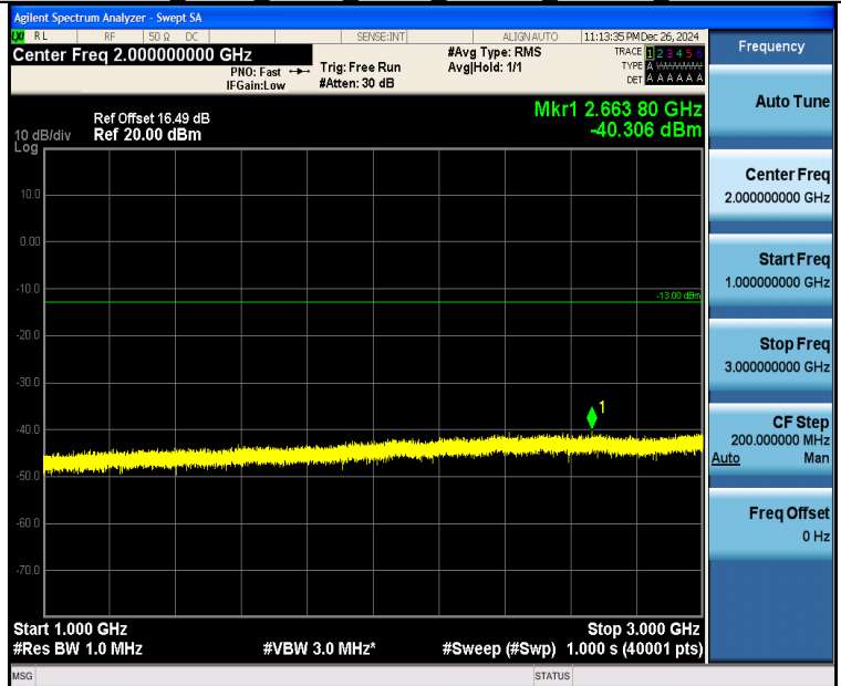
Band26_3MHz_QPSK_26915_1RB#14_1000~3000_1000~3000
