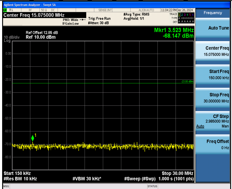
Band26_3MHz_QPSK_26805_1RB#0_0.15~30_0.15~30
