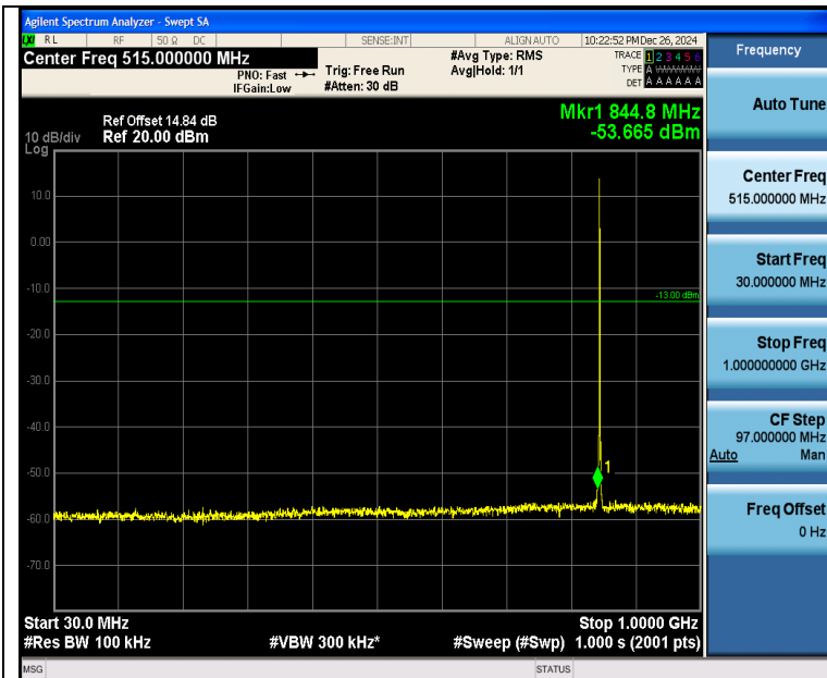
Band26 1.4MHz QPSK 27033 1RB#0 30~1000 30~1000
