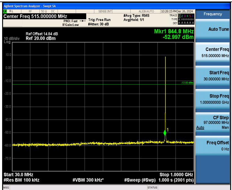
Band26 1.4MHz 16QAM 27033 6RB#0 30~1000 30~1000
