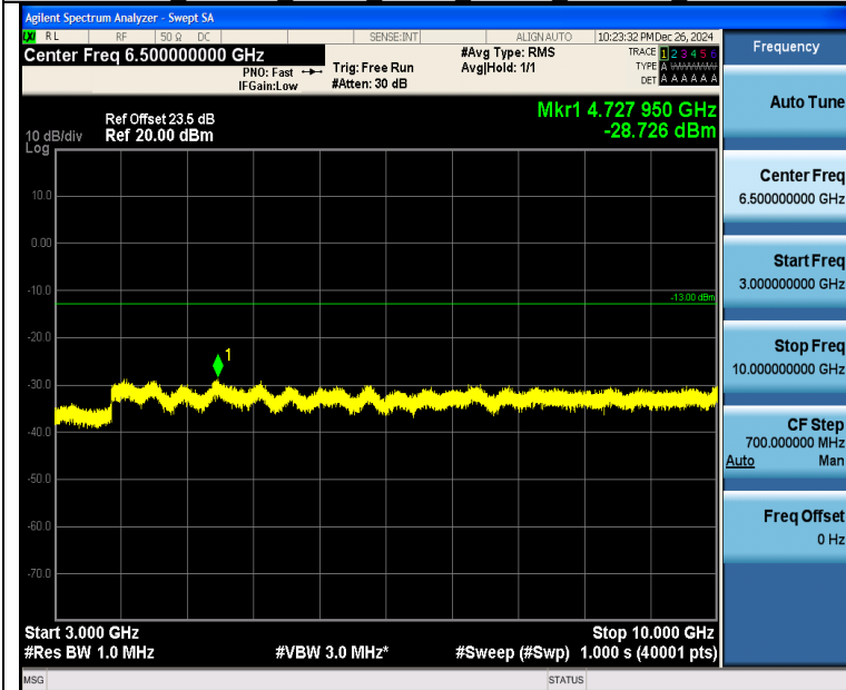
Band26 1.4MHz QPSK 27033 1RB#0 3000~10000 3000~10000
