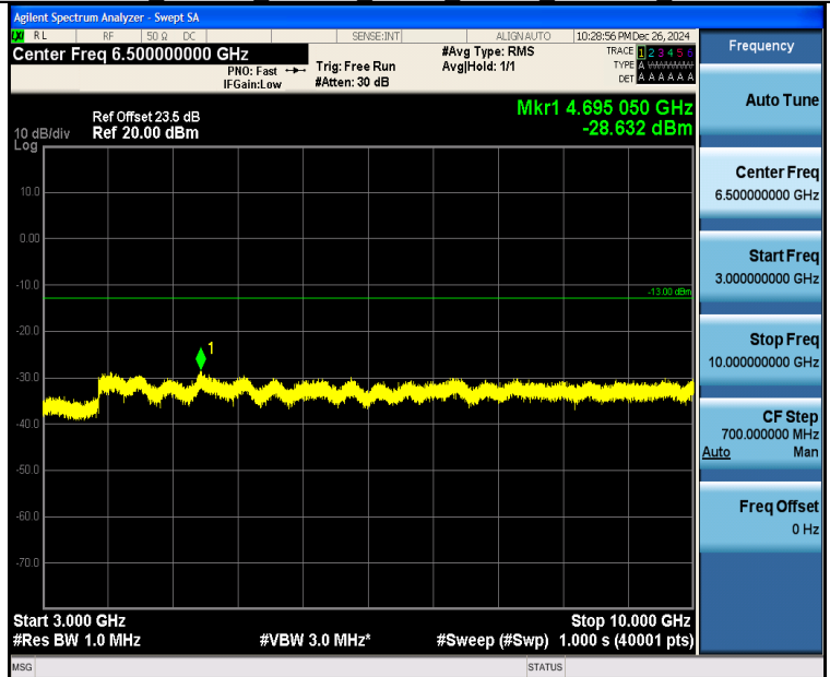
Band26 1.4MHz 16QAM 27033 6RB#0 3000~10000 3000~10000
