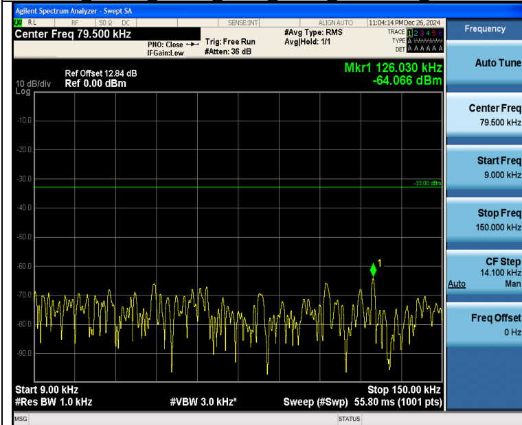
Band26_3MHz_QPSK_26805_1RB#0_0.009~0.15_0.009~0.15
