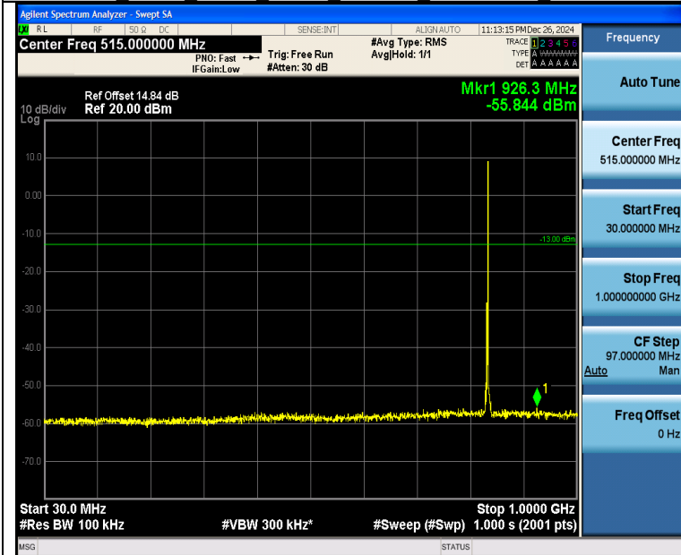
Band26_3MHz_QPSK_26915_1RB#14_30~1000_30~1000
