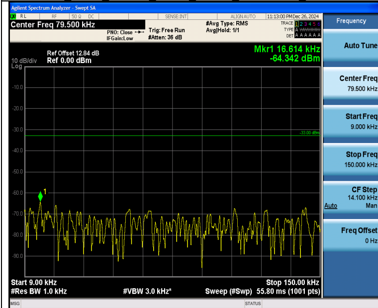
Band26 3MHz QPSK 26915 1RB#14 0.009~0.15 0.009~0.15
