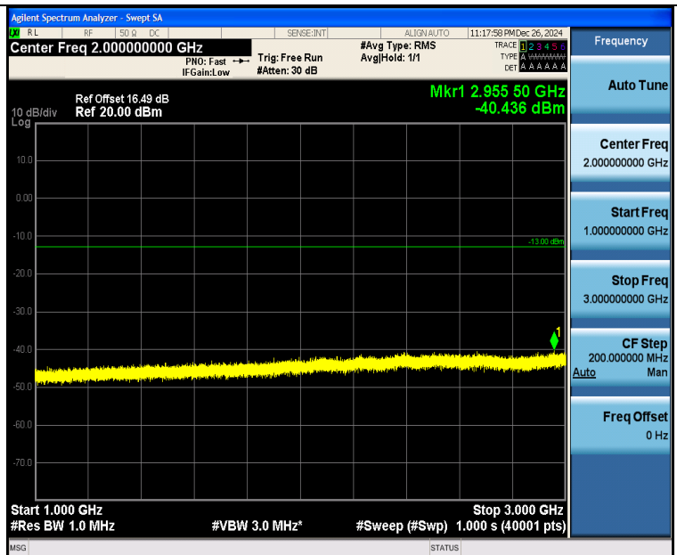
Band26 3MHz QPSK 27025 1RB#0 1000~3000 1000~3000
