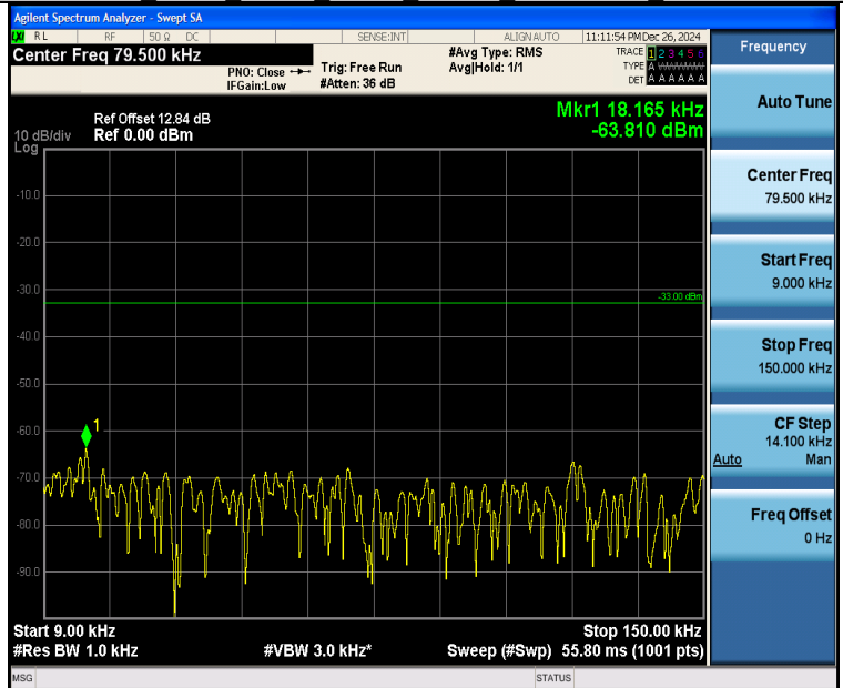
Band26 3MHz 16QAM 26915 1RB#0 0.009~0.15 0.009~0.15
