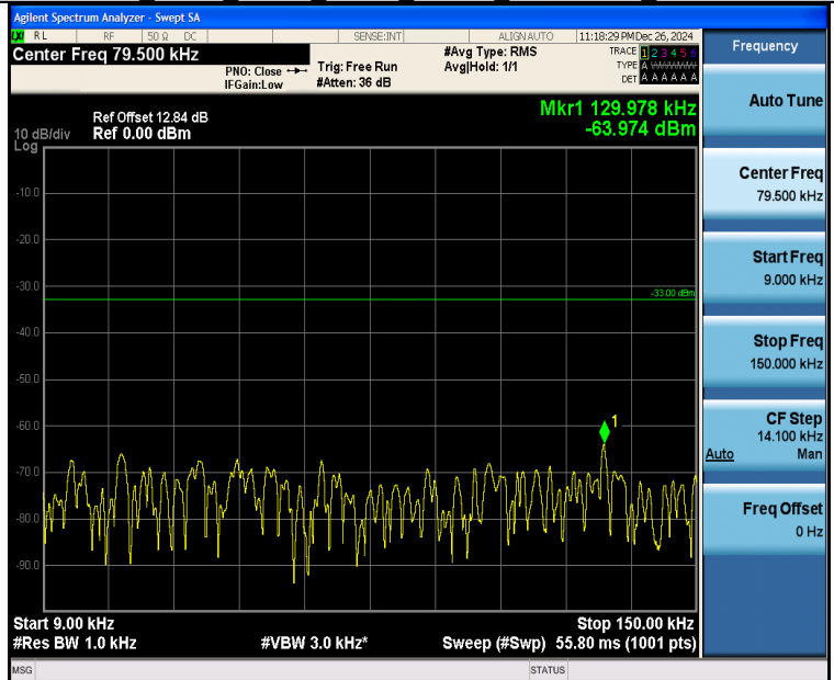
Band26 3MHz 16QAM 27025 1RB#0 0.009~0.15 0.009~0.15
