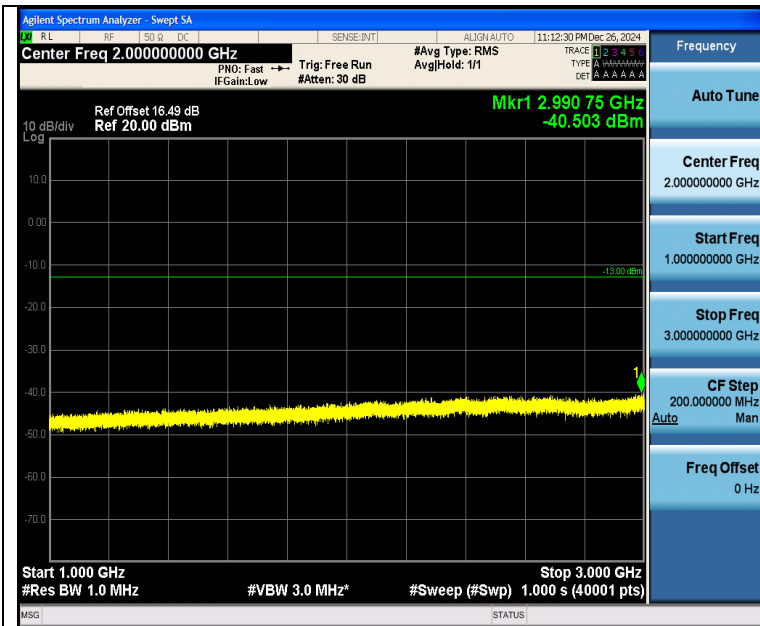
Band26 3MHz 16QAM 26915 1RB#0 1000~3000 1000~3000
