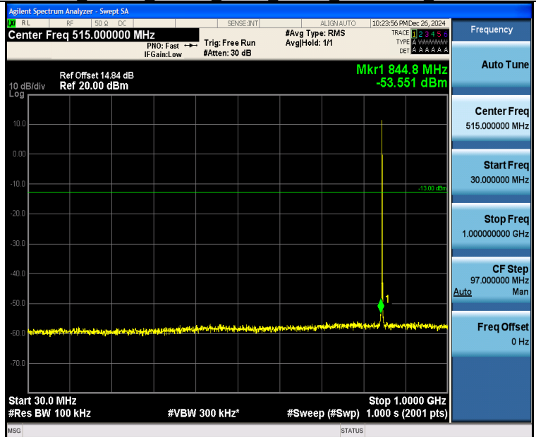
Band26 1.4MHz 16QAM 27033 1RB#0 30~1000 30~1000
