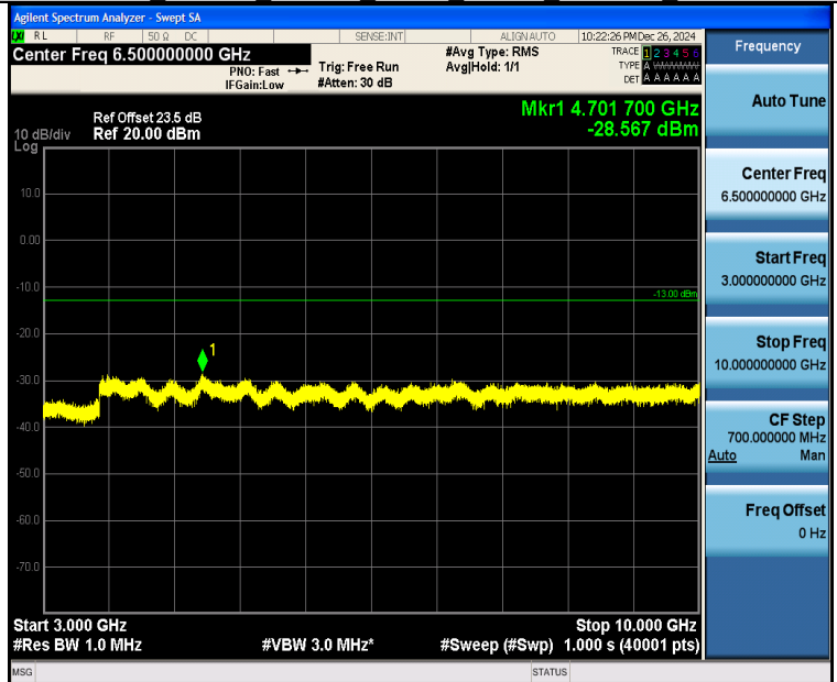
Band26 1.4MHz 16QAM 26915 6RB#0 3000~10000 3000~10000
