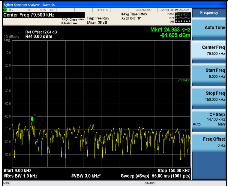
Band26 1.4MHz 16QAM 27033 1RB#0 0.009~0.15 0.009~0.15
