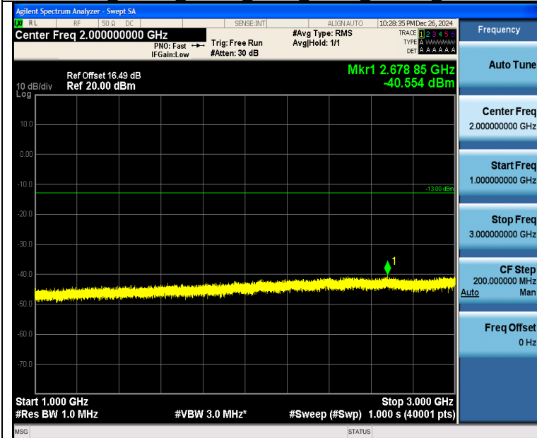
Band26 1.4MHz 16QAM 27033 6RB#0 1000~3000 1000~3000
