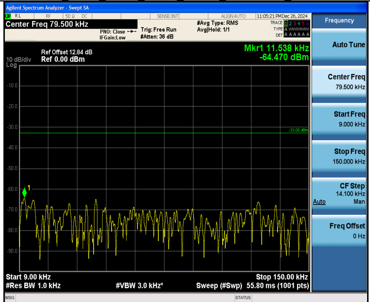
Band26 3MHz 16QAM 26805 1RB#0 0.009~0.15 0.009~0.15
