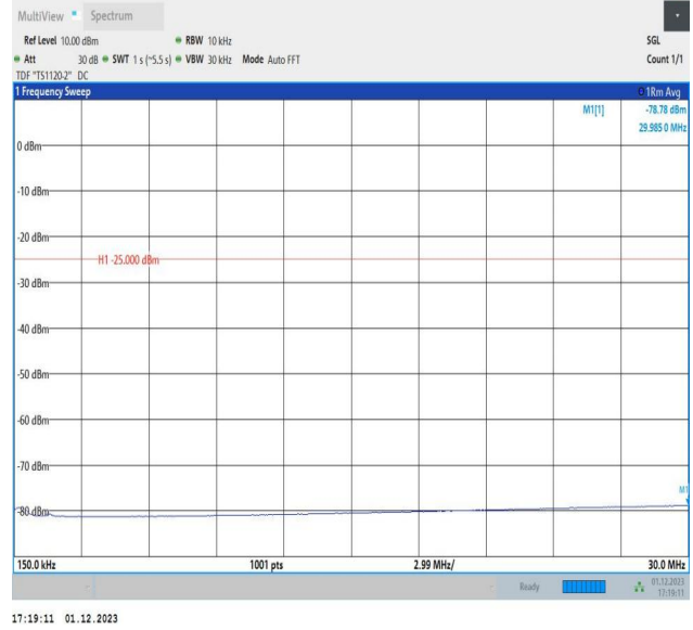
7-7-15MHz-20MHz-64QAM-64QAM-21003-21174-1RB#0-1RB #99-0.15~30MHz-PASS
