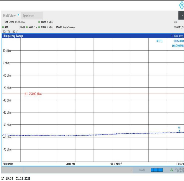
7-7-15MHz-20MHz-64QAM-64QAM-21003-21174-1RB#0-1RB #99-30~1000MHz-PASS
