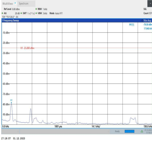
7-7-15MHz-20MHz-64QAM-64QAM-21003-21174-1RB#0-1RB #99-0.009~0.15MHz-PASS
