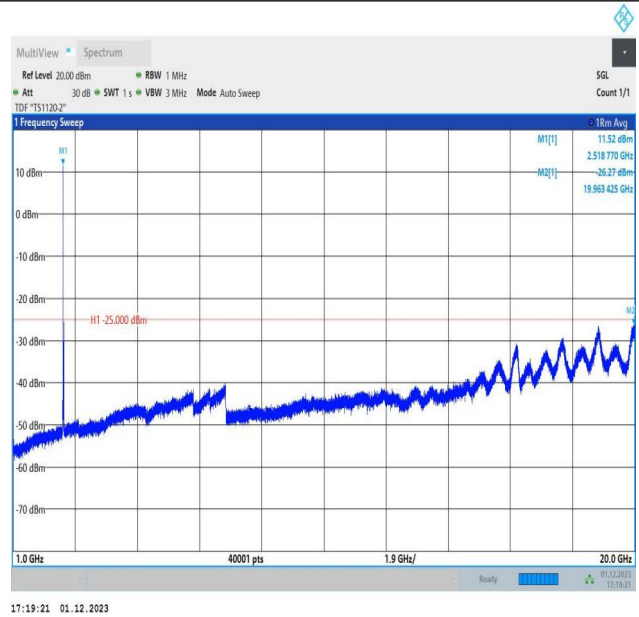
7-7-15MHz-20MHz-64QAM-64QAM-21003-21174-1RB#0-1RB #99-1000~20000MHz-PASS
