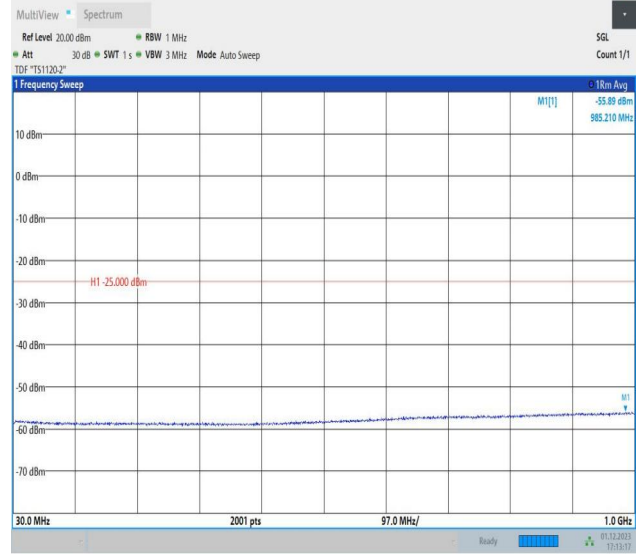
7-7-15MHz-20MHz-64QAM-64QAM-20828-20999-75RB#0-10 ORB#0-30~1000MHz-PASS
