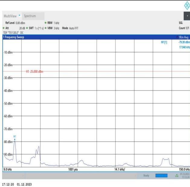
7-7-15MHz-20MHz-16QAM-16QAM-20828-20999-75RB#0-10 ORB#0-0.009~0.15MHz-PASS
