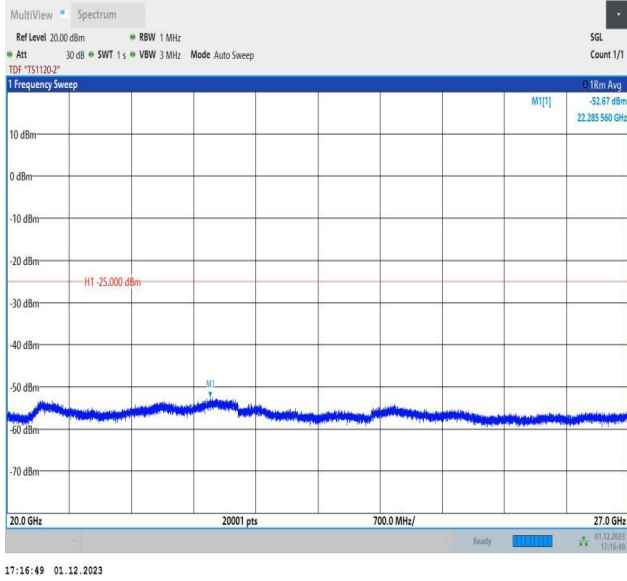
7-7-15MHz-20MHz-16QAM-16QAM-21003-21174-1RB#74-0R B#0-20000~27000MHz-PASS
