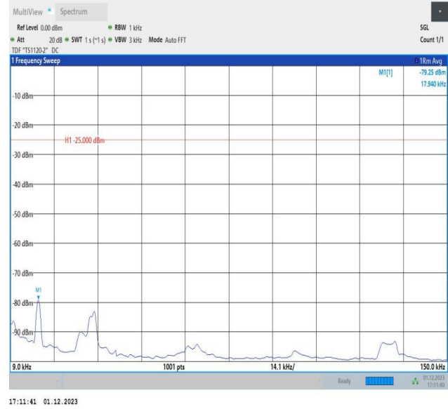
7-7-15MHz-20MHz-QPSK-QPSK-20828-20999-75RB#0-100R B#0-0.009~0.15MHz-PASS
