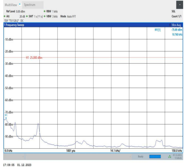
7-7-15MHz-20MHz-64QAM-64QAM-20828-20999-1RB#74-0R B#0-0.009~0.15MHz-PASS
