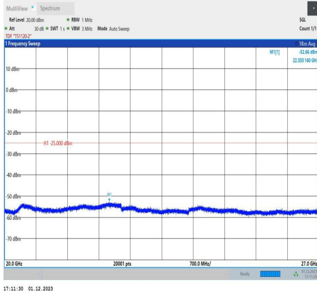
7-7-15MHz-20MHz-64QAM-64QAM-20828-20999-1RB#0-1RB #99-20000~27000MHz-PASS
