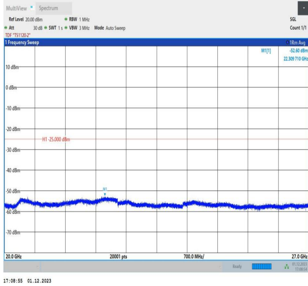
7-7-15MHz-20MHz-16QAM-16QAM-20828-20999-1RB#74-0R B#0-20000~27000MHz-PASS
