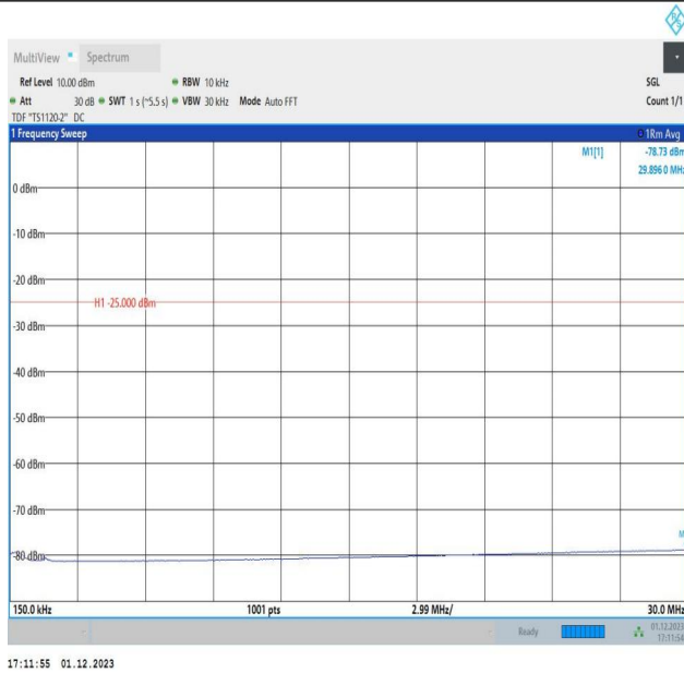
7-7-15MHz-20MHz-QPSK-QPSK-20828-20999-75RB#0-100R B#0-0.15~30MHz-PASS
