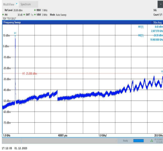
7-7-15MHz-20MHz-QPSK-QPSK-20828-20999-75RB#0-100R B#0-1000~20000MHz-PASS
