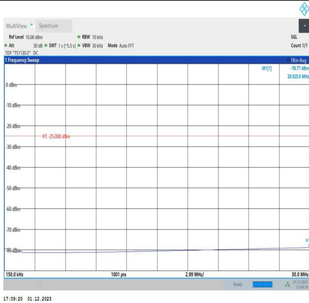
7-7-15MHz-20MHz-64QAM-64QAM-20828-20999-1RB#74-0R B#0-0.15~30MHz-PASS
