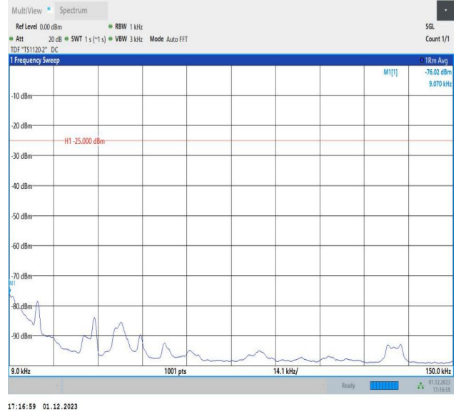
7-7-15MHz-20MHz-64QAM-64QAM-21003-21174-1RB#74-0R B#0-0.009~0.15MHz-PASS
