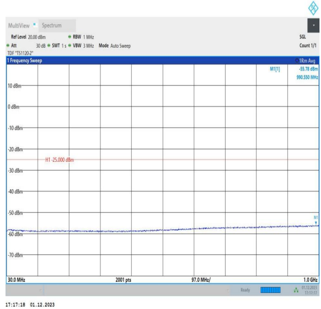
7-7-15MHz-20MHz-64QAM-64QAM-21003-21174-1RB#74-0R B#0-30~1000MHz-PASS
