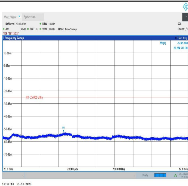
7-7-15MHz-20MHz-QPSK-QPSK-20828-20999-1RB#0-1RB#9 9-20000~27000MHz-PASS
