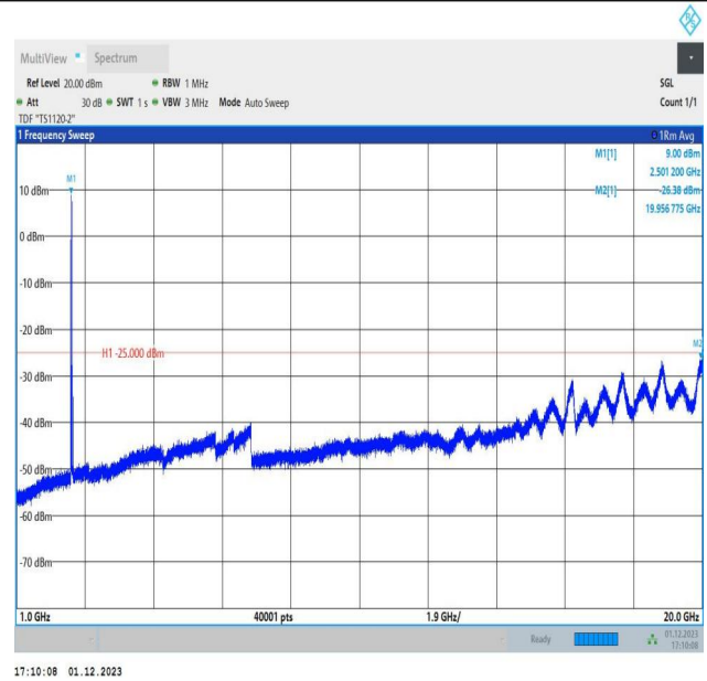
7-7-15MHz-20MHz-QPSK-QPSK-20828-20999-1RB#0-1RB#9 9-1000~20000MHz-PASS
