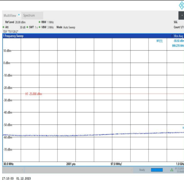
7-7-15MHz-20MHz-QPSK-QPSK-20828-20999-1RB#0-1RB#9 9-30~1000MHz-PASS
