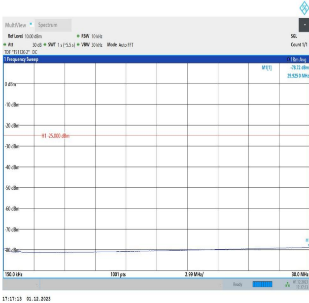
7-7-15MHz-20MHz-64QAM-64QAM-21003-21174-1RB#74-0R B#0-0.15~30MHz-PASS
