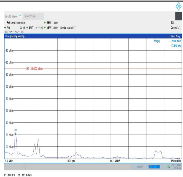
7-7-15MHz-20MHz-16QAM-16QAM-20828-20999-1RB#0-1RB #99-0.009~0.15MHz-PASS
