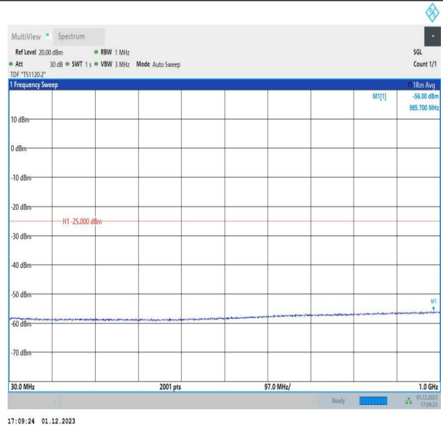
7-7-15MHz-20MHz-64QAM-64QAM-20828-20999-1RB#74-0R B#0-30~1000MHz-PASS
