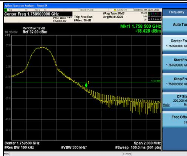
Band4_10MHz_16QAM_20385_1RB#49
