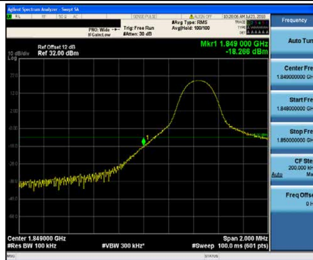
Band2_5MHz_QPSK_18615_1RB#0
