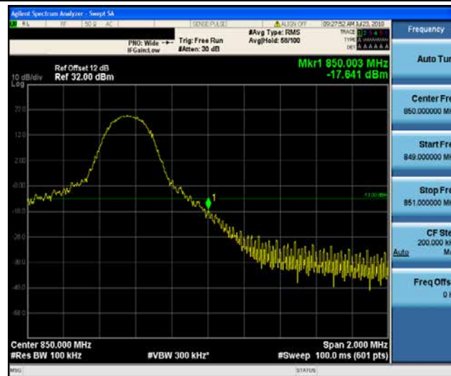
Band5_5MHz_QPSK_20635_1RB#24
