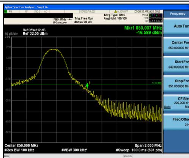
Band5_5MHz_16QAM_20635_1RB#24
