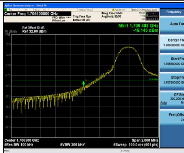
Band4_10MHz_16QAM_19965_1RB#0
