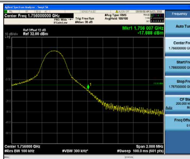
Band4_5MHz_16QAM_20385_1RB#24
