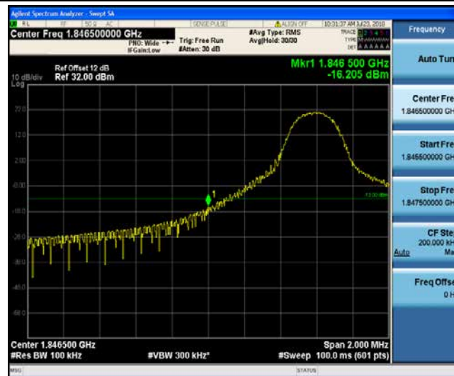
Band2_10MHz_16QAM_18615_1RB#0
