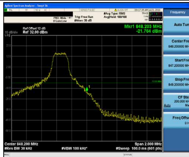
Band5_1.4MHz_16QAM_20635_1RB#5
