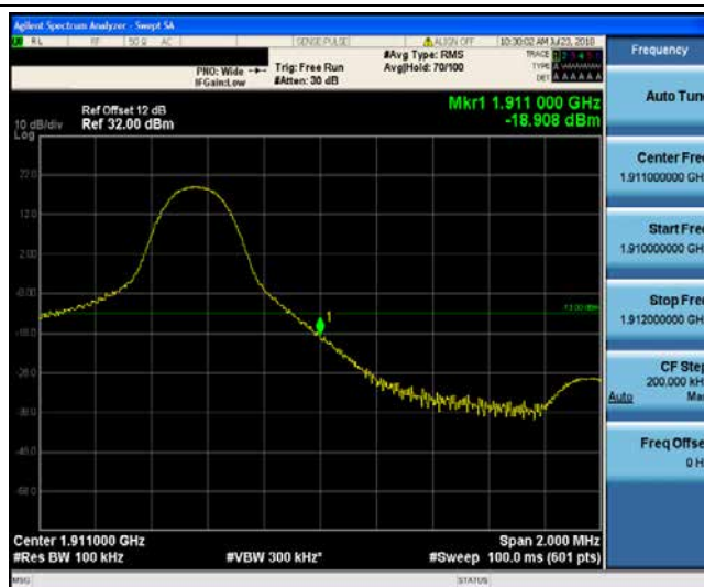
Band2_5MHz_QPSK_19185_1RB#24
