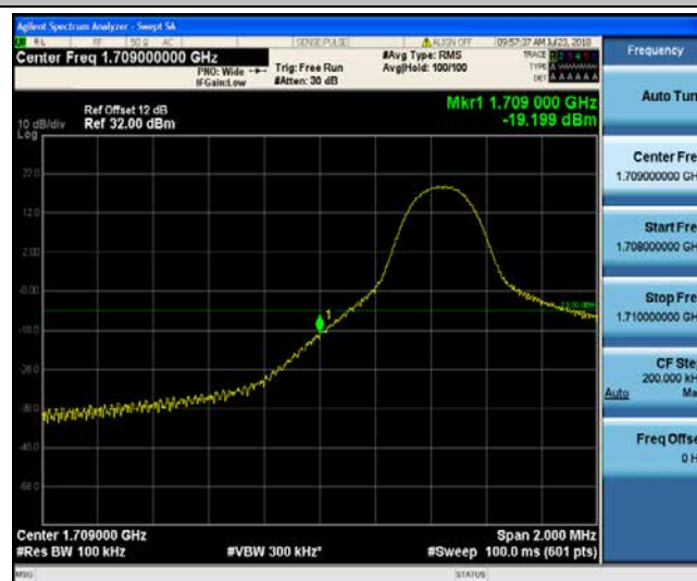
Band4_5MHz_16QAM_19965_1RB#0
