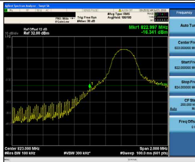
Band5_5MHz_QPSK_20415_1RB#0
