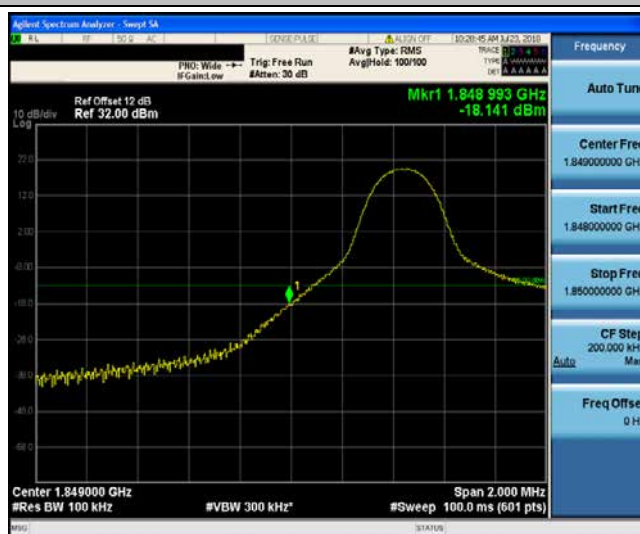
Band2_5MHz_16QAM_18615_1RB#0
