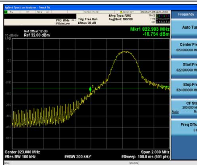
Band5_5MHz_16QAM_20415_1RB#0
