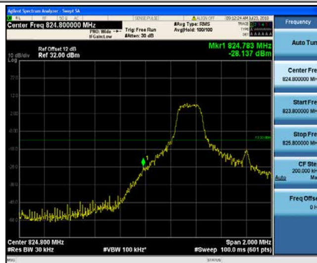
Band5_1.4MHz_QPSK_20415_1RB#0
