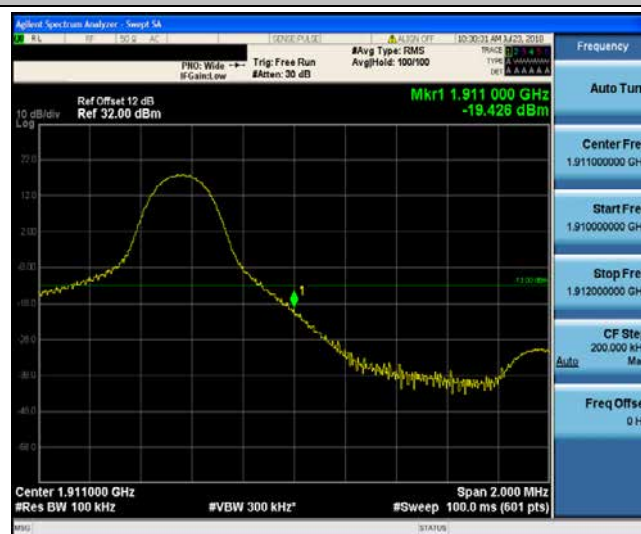
Band2_5MHz_16QAM_19185_1RB#24
