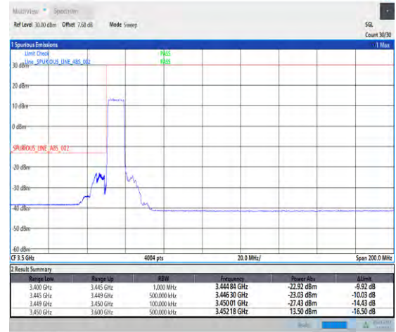
1-N78-3450-3550-30-10-L-3-DFT-PI2BPSK-Outer _Full-24@0-Ant1-1--PASS-see graph
