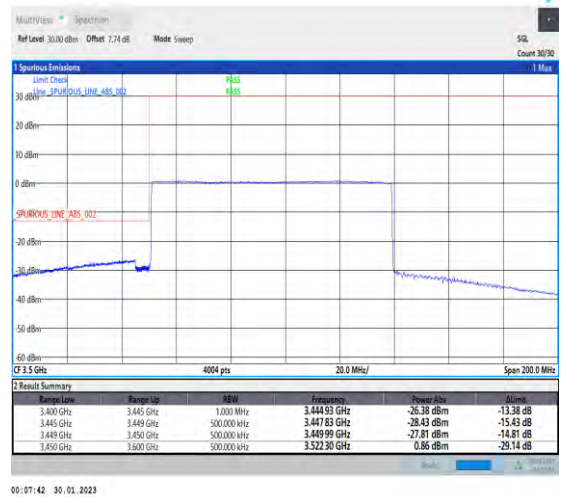
1-N78-3450-3550-30-90-L-6-CP-QPSK-Outer_Full -245@0-Ant1-1--PASS-see graph
