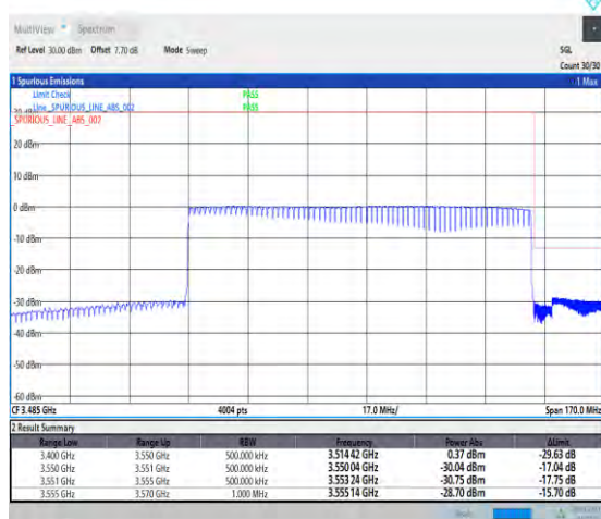
1-N78-3450-3550-30-100-H-6-CP-QPSK-Outer_Full-273@0-Ant1-1--PASS-see graph
