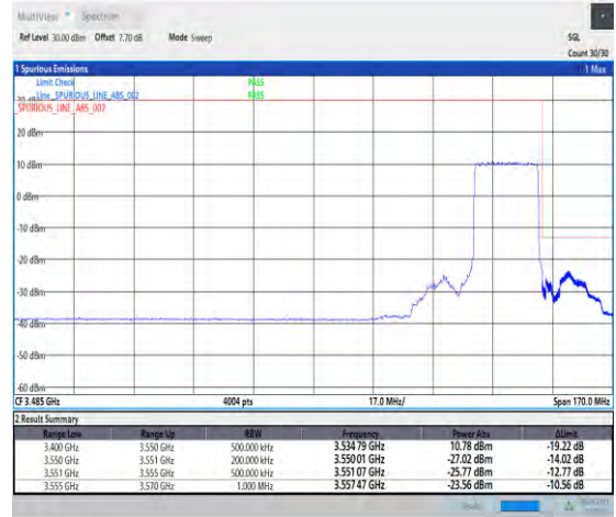
1-N78-3450-3550-30-20-H-3-DFT-PI2BPSK-Outer _Full-50@0-Ant1-1--PASS-see graph
