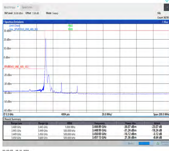
1-N78-3450-3550-30-40-L-1-DFT-PI2BPSK-Edge_1RB _Left-1@0-Ant1-1--PASS-see graph
