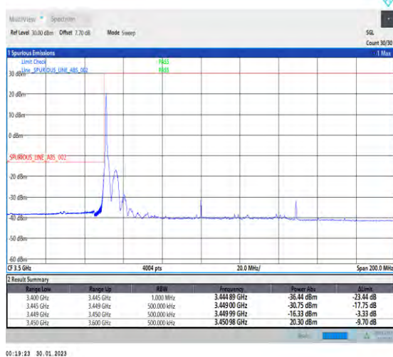
1-N78-3450-3550-30-100-L-4-CP-QPSK-Edge_1RB_Left-1@0-Ant1-1--PASS-see graph
