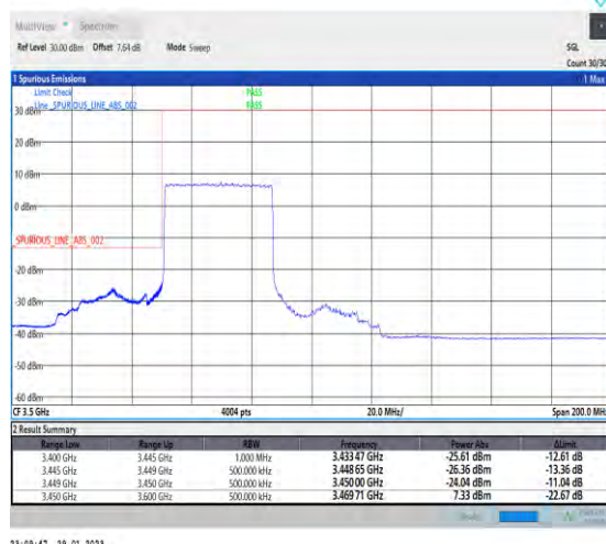
1-N78-3450-3550-30-40-L-3-DFT-PI2BPSK-Outer _Full-100@0-Ant1-1--PASS-see graph
