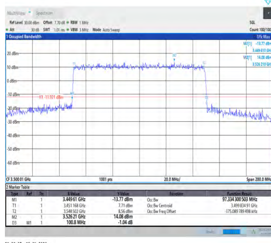
1-N78-3450-3550-30-100-M-7-CP-16QAM-Outer_Full-273@0-Ant1-97.334-100.800-≤100-PASS
