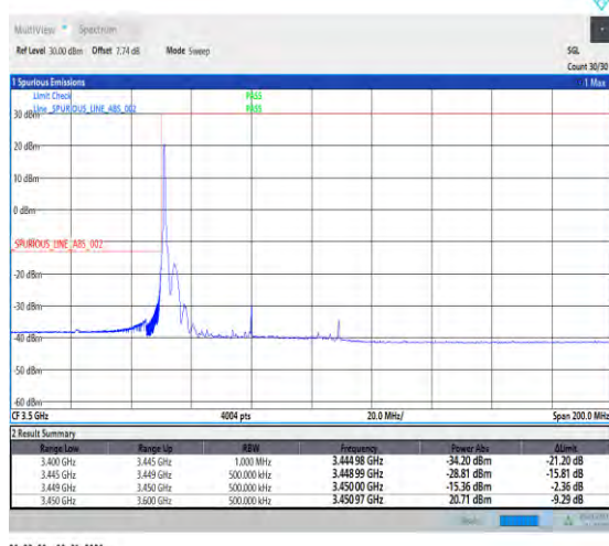
1-N78-3450-3550-30-60-L-4-CP-QPSK-Edge_1RB_Lef t-1@0-Ant1-1--PASS-see graph
