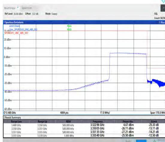
1-N78-3450-3550-30-40-H-6-CP-QPSK-Outer_Full -106@0-Ant1-1--PASS-see graph
