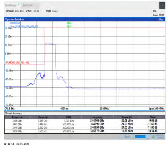
1-N78-3450-3550-30-15-L-3-DFT-PI2BPSK-Outer _Full-36@0-Ant1-1--PASS-see graph
