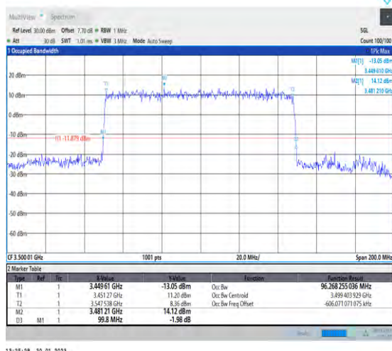
1-N78-3450-3550-30-100-M-4-DFT-64QAM-Outer_Full-270@0-Ant1-96.268-99.800-≤100-PASS
