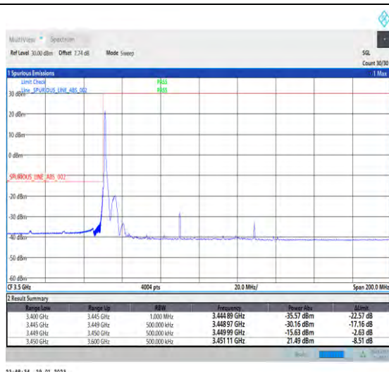
1-N78-3450-3550-30-80-L-1-DFT-PI2BPSK-Edge_1RB _Left-1@0-Ant1-1--PASS-see graph
