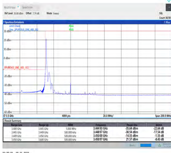
1-N78-3450-3550-30-60-L-1-DFT-PI2BPSK-Edge_1RB _Left-1@0-Ant1-1--PASS-see graph
