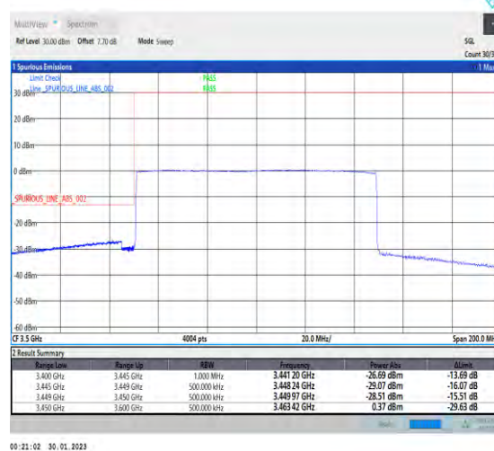
1-N78-3450-3550-30-100-L-6-CP-QPSK-Outer_Full-273@0-Ant1-1--PASS-see graph
