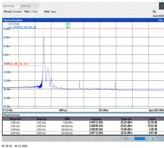
1-N78-3450-3550-30-90-L-4-CP-QPSK-Edge_1RB_Lef t-1@0-Ant1-1--PASS-see graph
