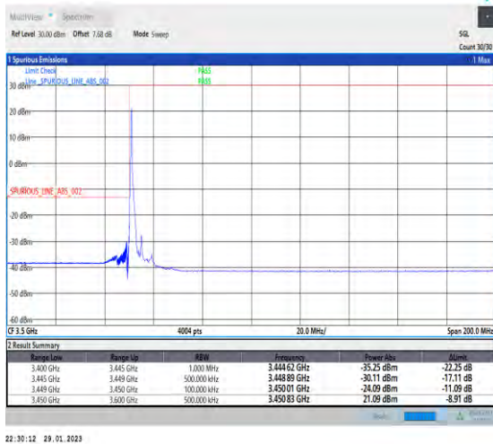
1-N78-3450-3550-30-10-L-4-CP-QPSK-Edge_1RB_Lef t-1@0-Ant1-1--PASS-see graph
