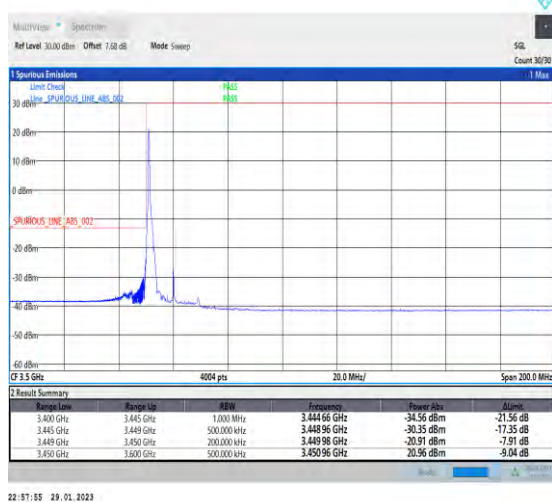
1-N78-3450-3550-30-20-L-4-CP-QPSK-Edge_1RB_Lef t-1@0-Ant1-1--PASS-see graph
