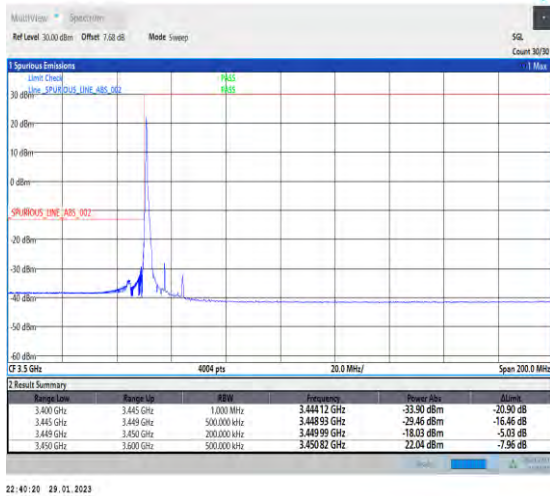
1-N78-3450-3550-30-15-L-1-DFT-PI2BPSK-Edge_1RB _Left-1@0-Ant1-1--PASS-see graph
