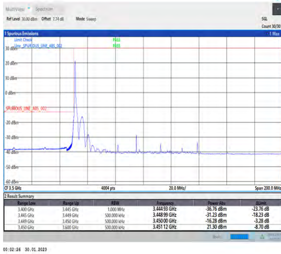
1-N78-3450-3550-30-90-L-1-DFT-PI2BPSK-Edge_1RB _Left-1@0-Ant1-1--PASS-see graph
