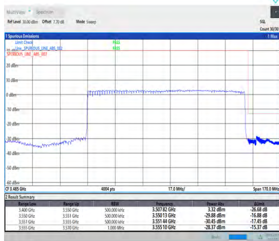
1-N78-3450-3550-30-100-H-3-DFT-PI2BPSK-Oute_r_Full-270@0-Ant1-1--PASS-see graph
