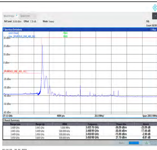
1-N78-3450-3550-30-100-L-1-DFT-PI2BPSK-Edge_1R_B_Left-1@0-Ant1-1--PASS-see graph
