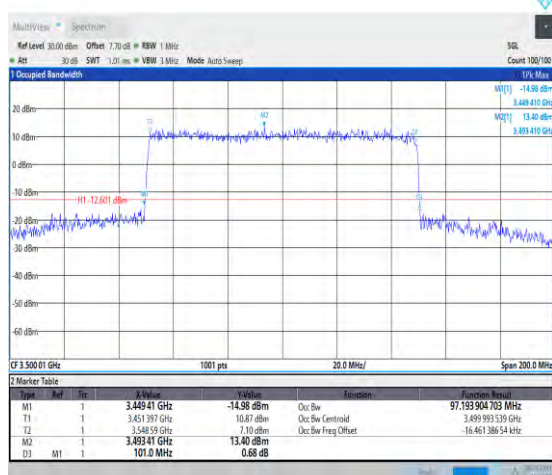
1-N78-3450-3550-30-100-L-7-CP-16QAM-Out-er_Full-273@0-Ant1-97.194-101.000-≤100-PASS
