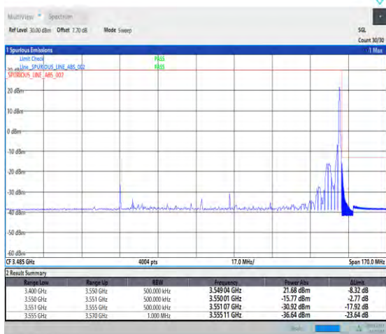
1-N78-3450-3550-30-100-H-2-DFT-PI2BPSK-Edge_1R_B_Right-1@272-Ant1-1--PASS-see graph
