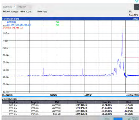
1-N78-3450-3550-30-100-H-5-CP-QPSK-Edge_1RB_Right-1@272-Ant1-1--PASS-see graph
