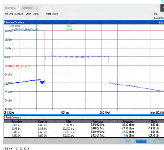
1-N78-3450-3550-30-80-L-6-CP-QPSK-Outer_Full -217@0-Ant1-1--PASS-see graph
