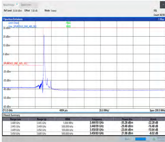
1-N78-3450-3550-30-10-L-1-DFT-PI2BPSK-Edge_1RB _Left-1@0-Ant1-1--PASS-see graph
