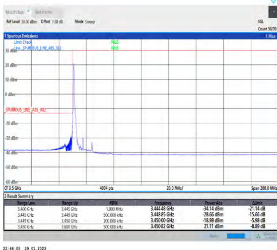
1-N78-3450-3550-30-15-L-4-CP-QPSK-Edge_1RB_Lef t-1@0-Ant1-1--PASS-see graph
