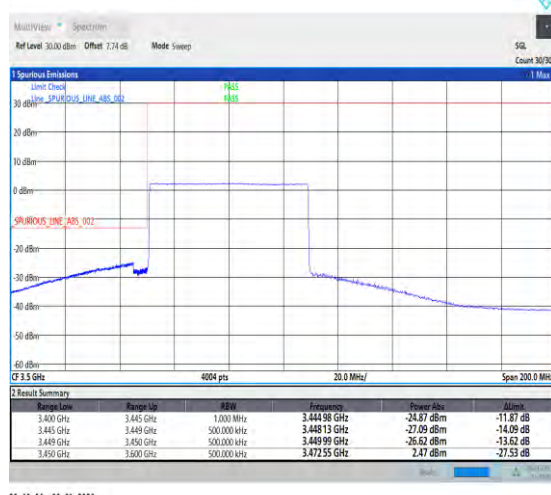
1-N78-3450-3550-30-60-L-6-CP-QPSK-Outer_Full -162@0-Ant1-1--PASS-see graph
