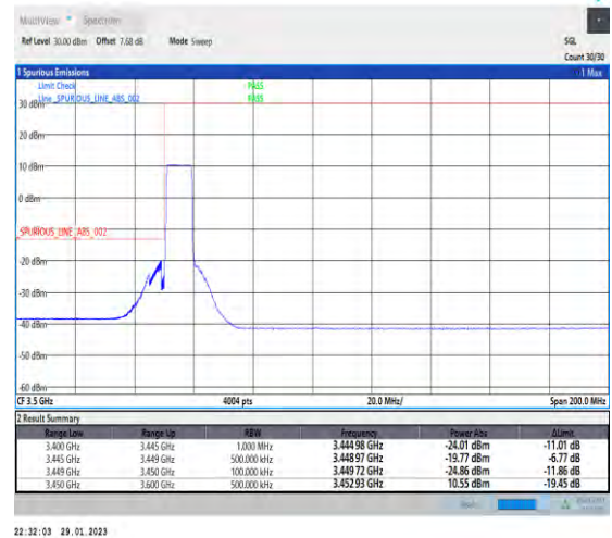
1-N78-3450-3550-30-10-L-6-CP-QPSK-Outer_Full -24@0-Ant1-1--PASS-see graph
