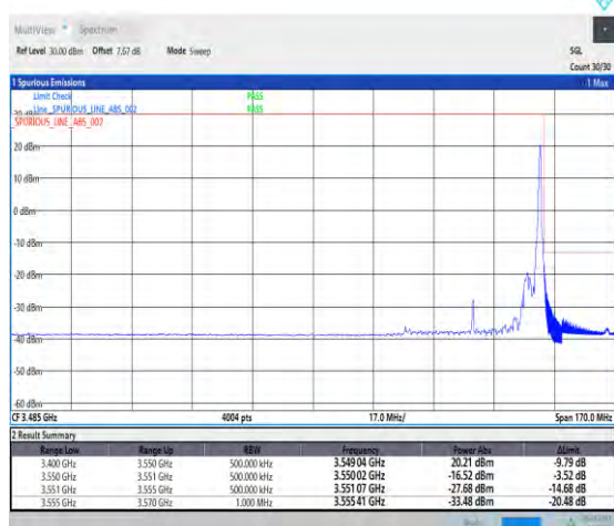
1-N78-3450-3550-30-40-H-5-CP-QPSK-Edge_1RB_Ri ght-1@105-Ant1-1--PASS-see graph
