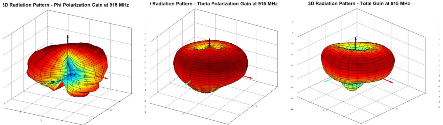
Figure 8: Phi polarization, Theta polarization and, and total gain plots – 915 MHz
