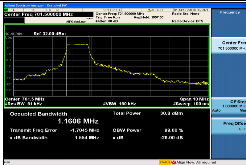
Band12-5MHz-QPSK-23035-6RB#0-1.1606
