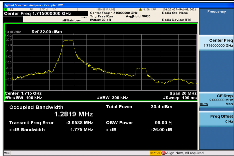
Band4-10MHz-QPSK-20000-6RB#0-1.2819
