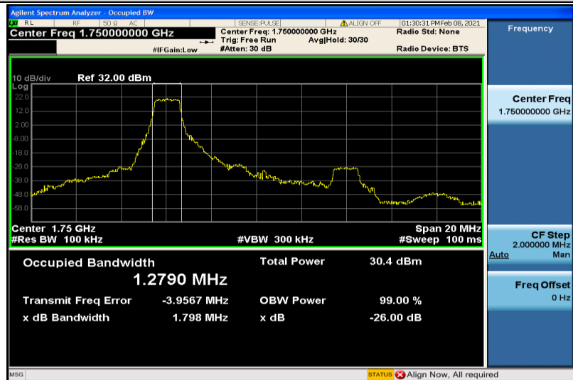
Band4-10MHz-QPSK-20350-6RB#0-1.2790
