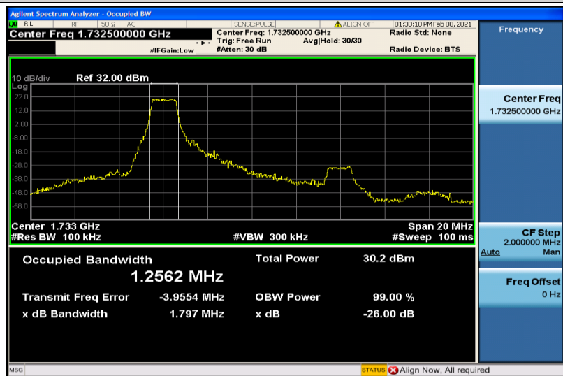
Band4-10MHz-QPSK-20175-6RB#0-1.2562
