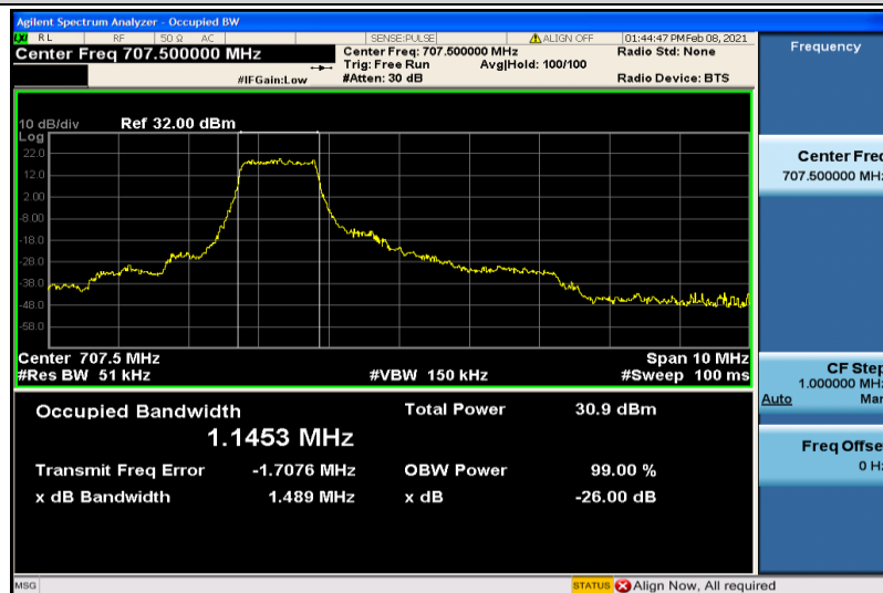
Band12-5MHz-QPSK-23095-6RB#0-1.1453
