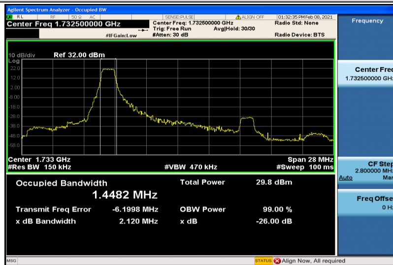
Band4-15MHz-QPSK-20175-6RB#0-1.4482
