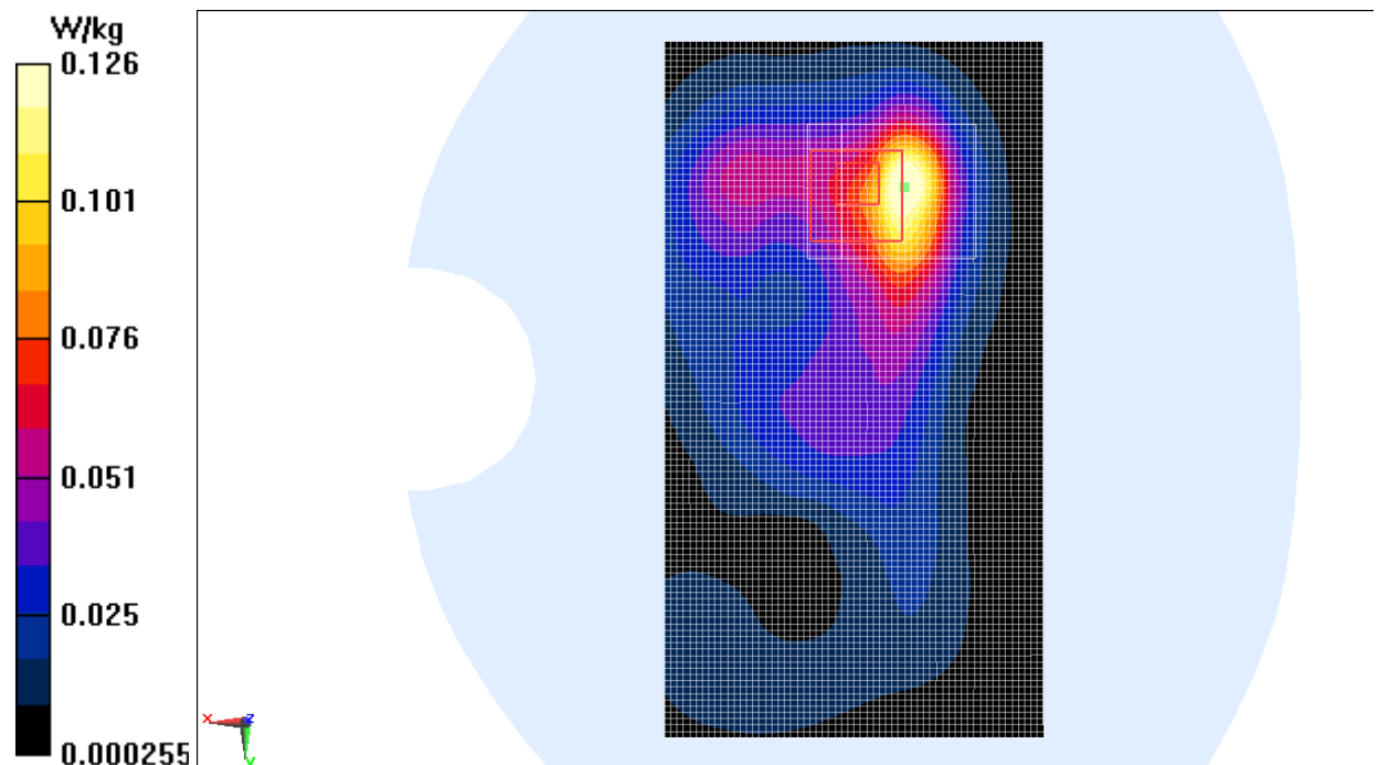
Fig.10 2450 MHz CH11
