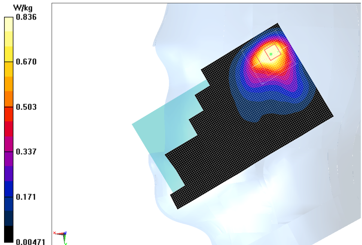
Fig.9 2450 MHz CH11
