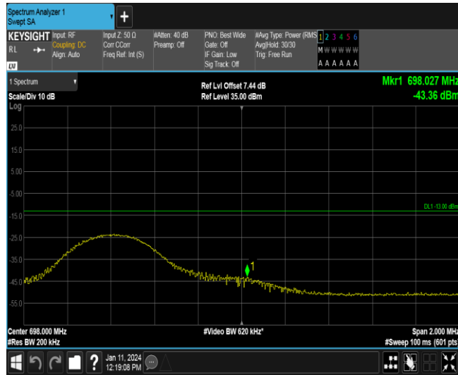
Band71-10MHz-16QAM-133422-1RB#49
