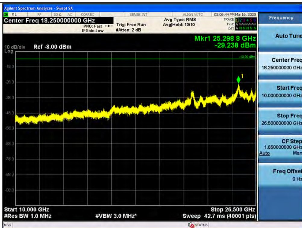
Spurious / PCS / Downlink / CDMA / Middle / 10 GHz ~ 26.5 GHz
