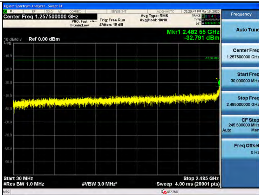
Spurious / BRS/EBS / Downlink / LTE 20 MHz / Low / 30 MHz ~ Low Edge - 1.1 MHz
