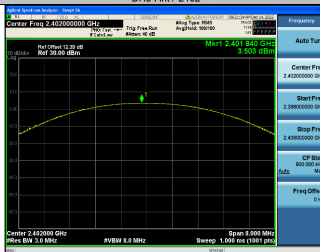
2DH5-Ant1-2402
