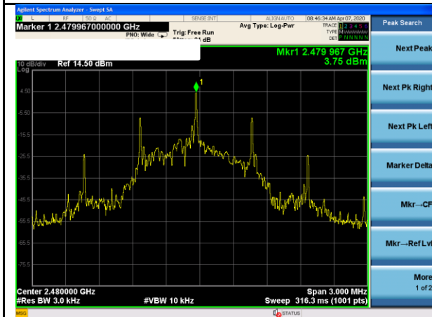
BLE-PSD-High
