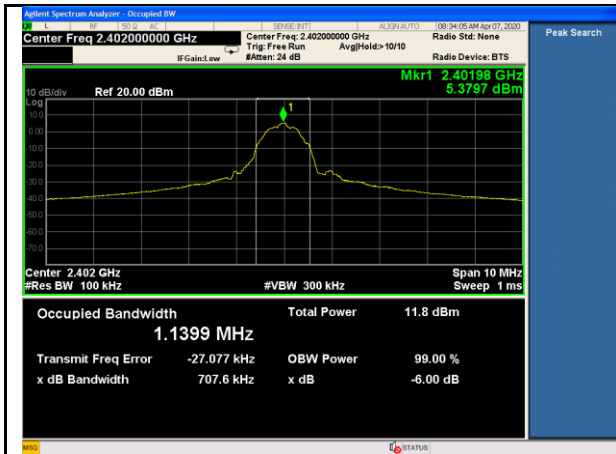
BLE-DTS BW-Low
