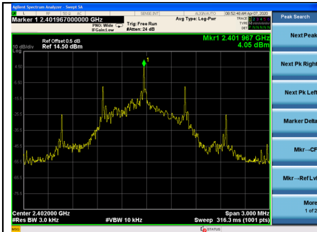
BLE-PSD-Low
