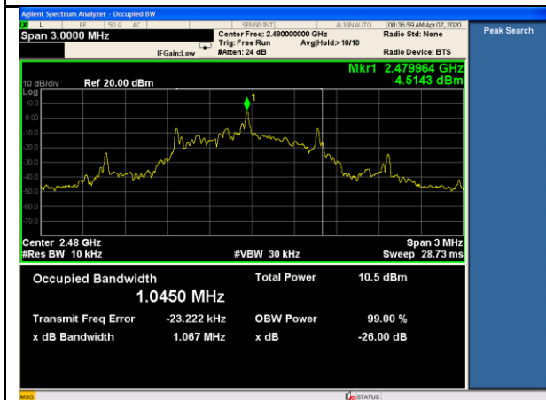
BLE-OBW-High
