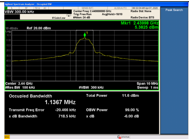
BLE-DTS BW-Mid
