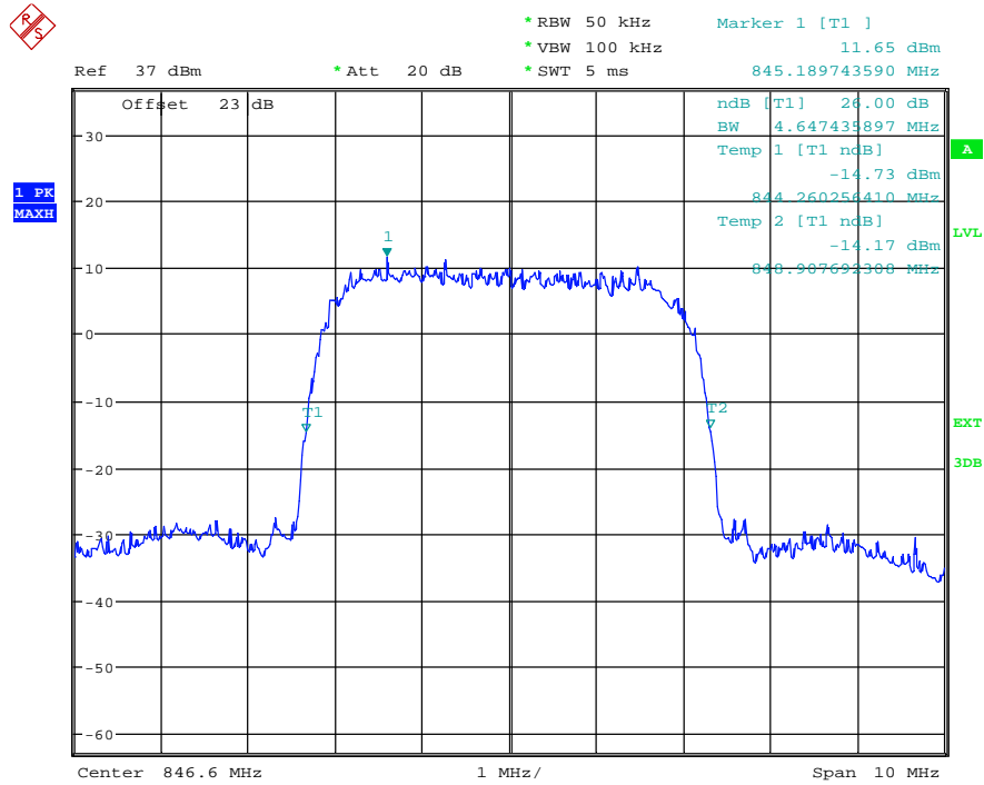
(Plot 4.4.2 C: Channel 4233:846.6MHz @ WCDMA Band V)
