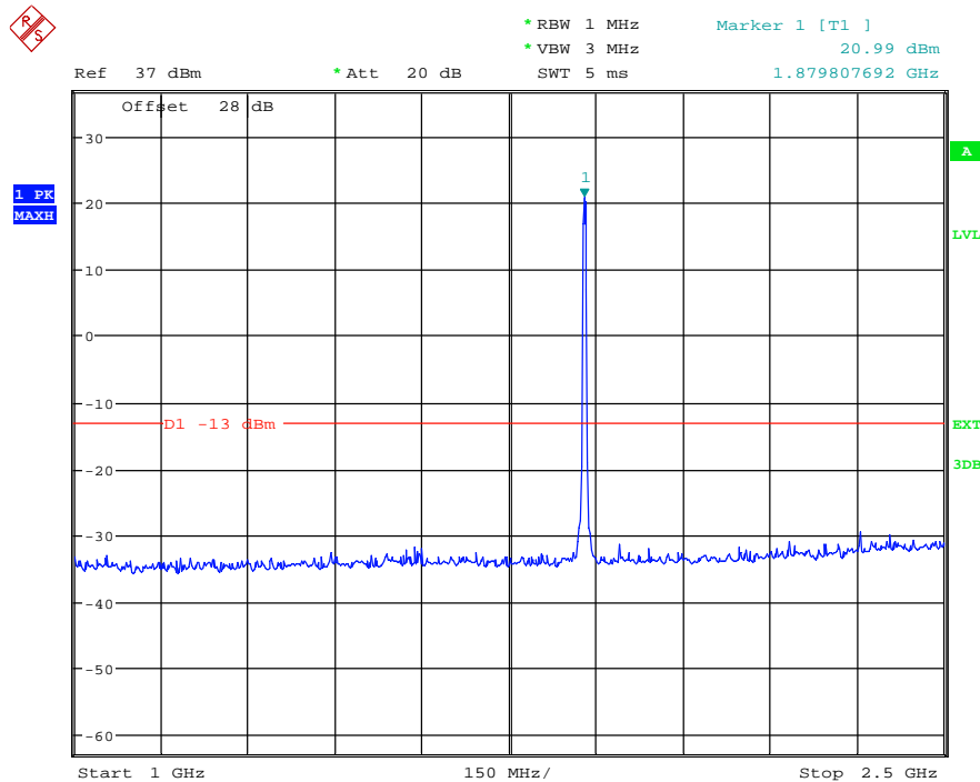
(Plot 4.6.1 B3: Channel 9400: 1880.0MHz @ Traffic WCDMA Band II)
