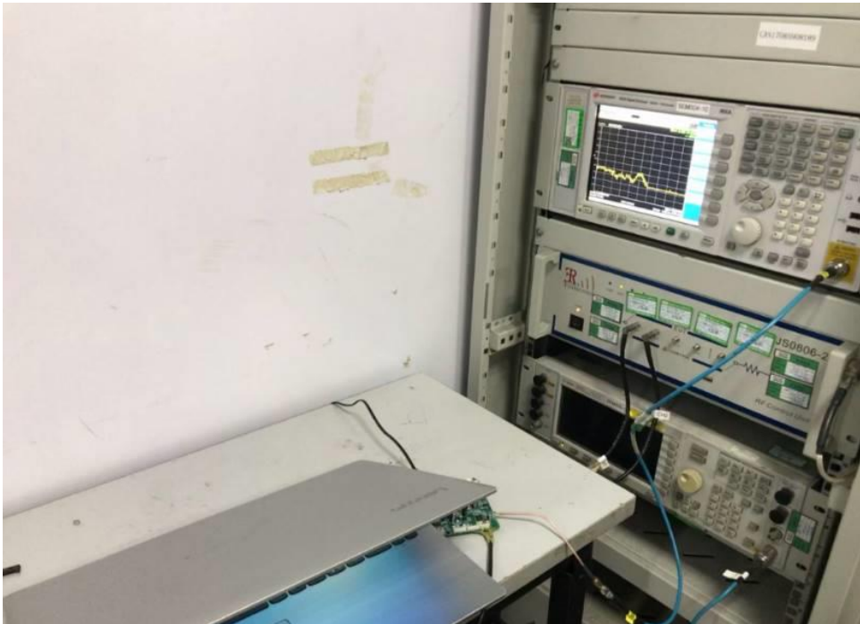
Conducted Emissions at AC Power Line (150kHz-30MHz)
