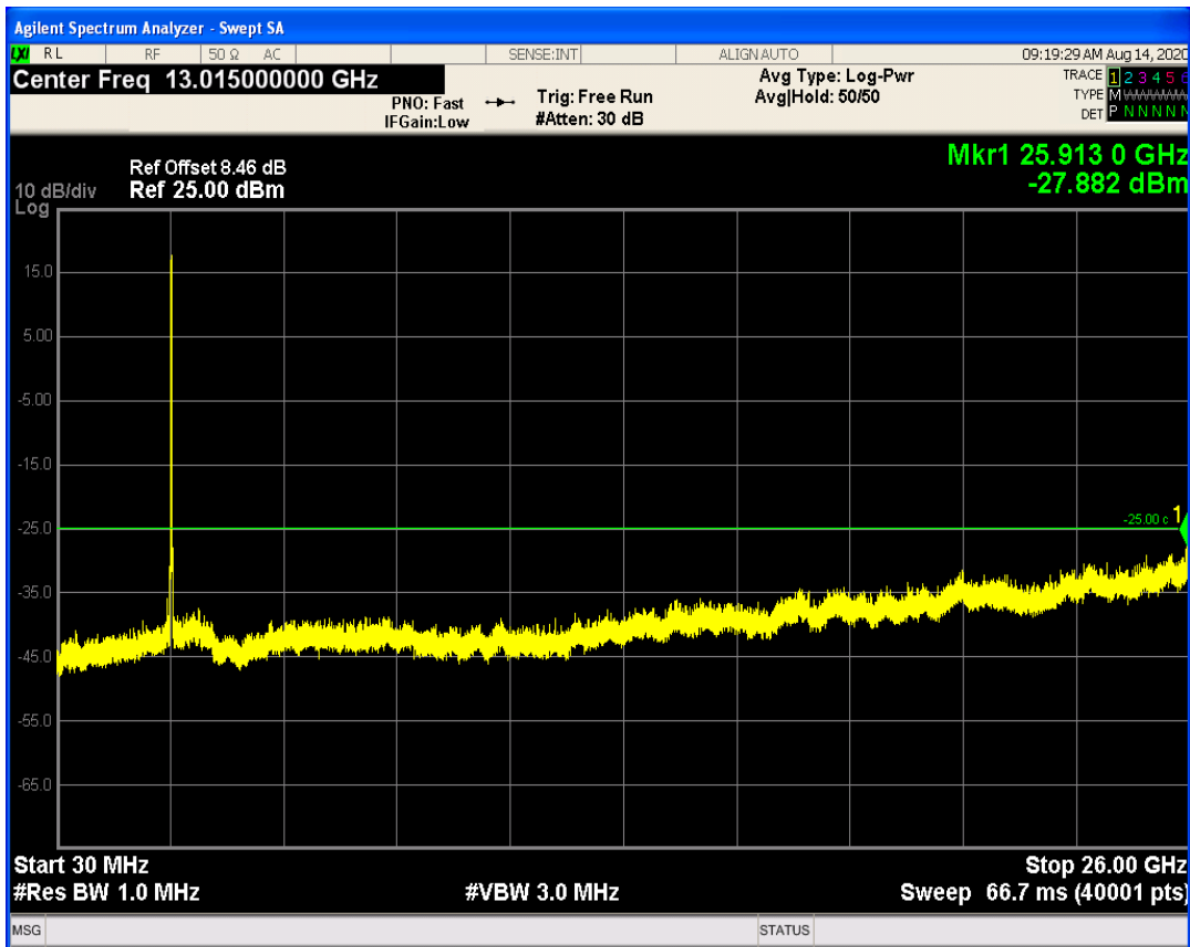
LTE Band41 QPSK BW=20MHz Channel=40340 RB Size=1 Position=#0
