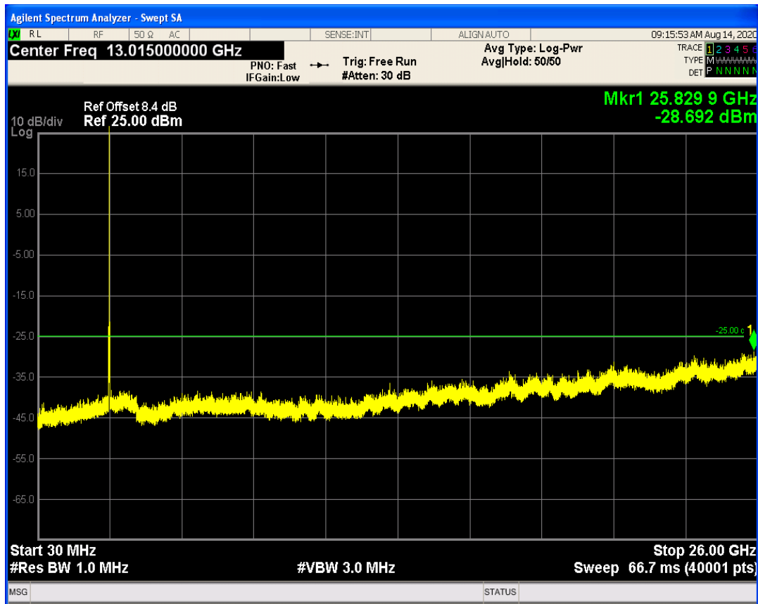
LTE Band41 QPSK BW=15MHz Channel=40740 RB Size=75 Position=#0
