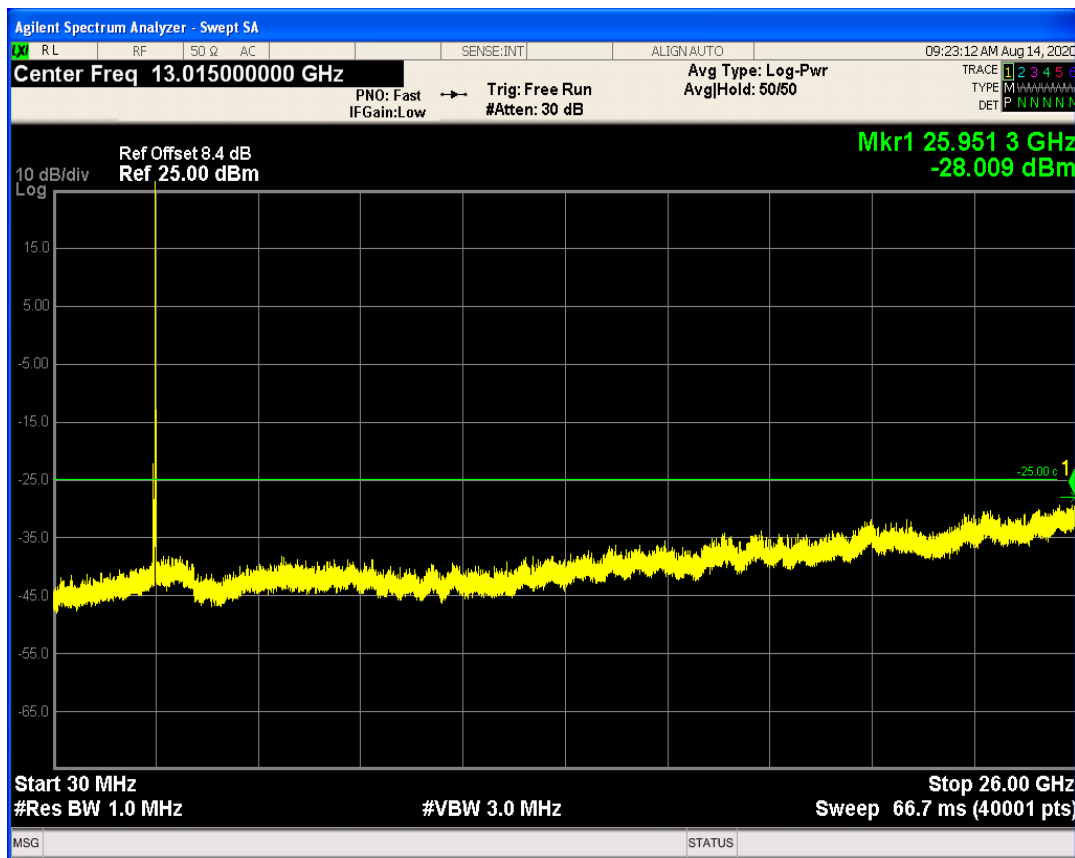
LTE Band41 QPSK BW=20MHz Channel=40740 RB Size=100 Position=#0
