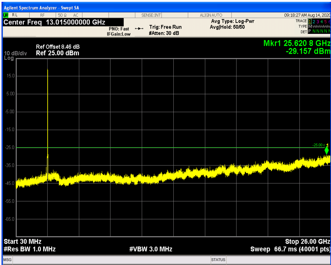
LTE Band41 QPSK BW=15MHz Channel=41165 RB Size=1 Position=#0
