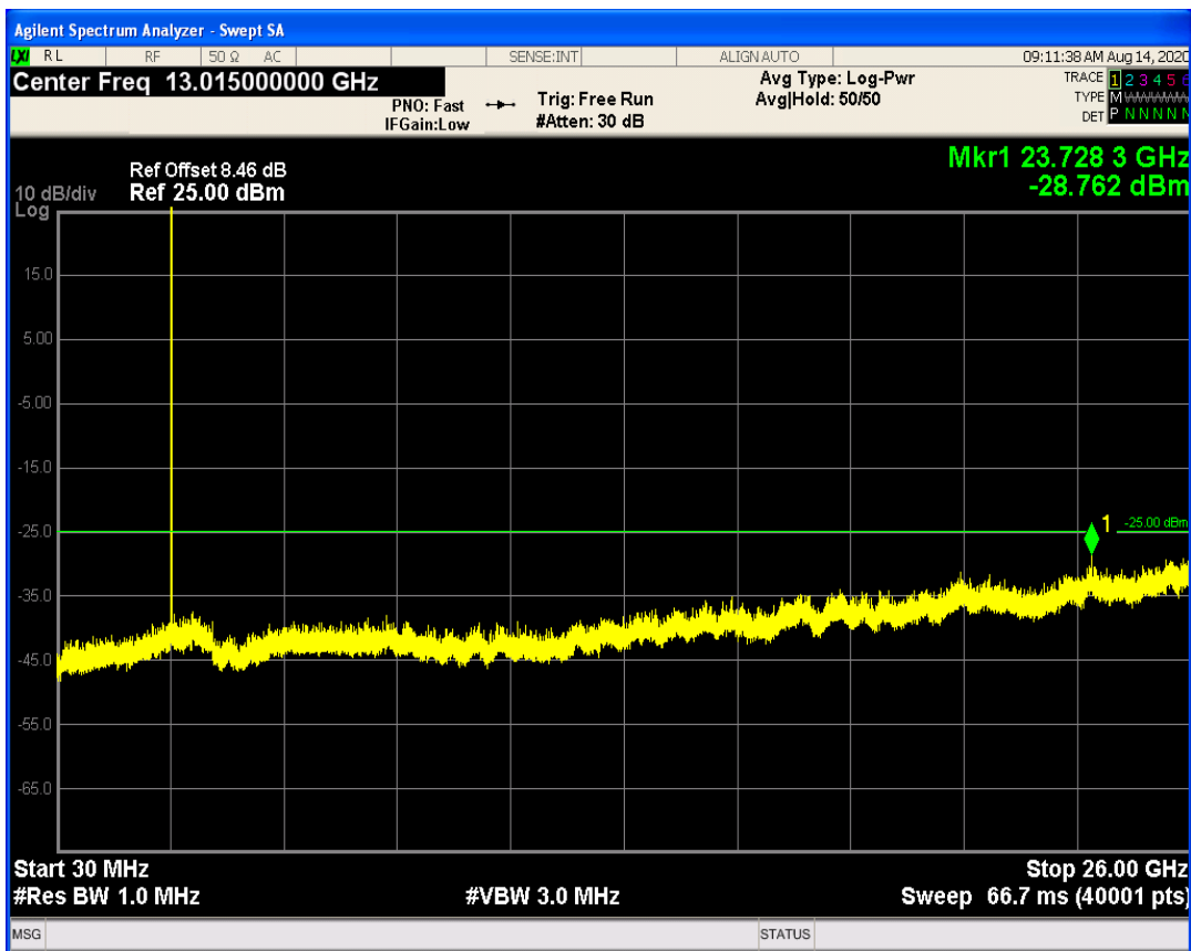
LTE Band41 QAM16 BW=10MHz Channel=41190 RB Size=1 Position=#0
