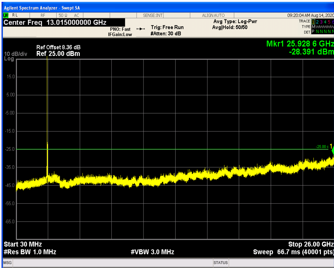
LTE Band41 QAM16 BW=20MHz Channel=40340 RB Size=1 Position=#0
