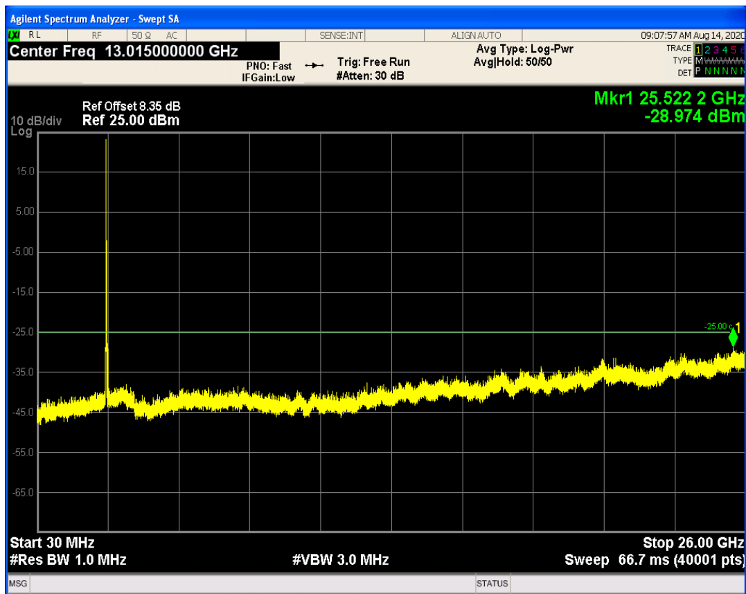
LTE Band41 QAM16 BW=10MHz Channel=40290 RB Size=1 Position=#0
