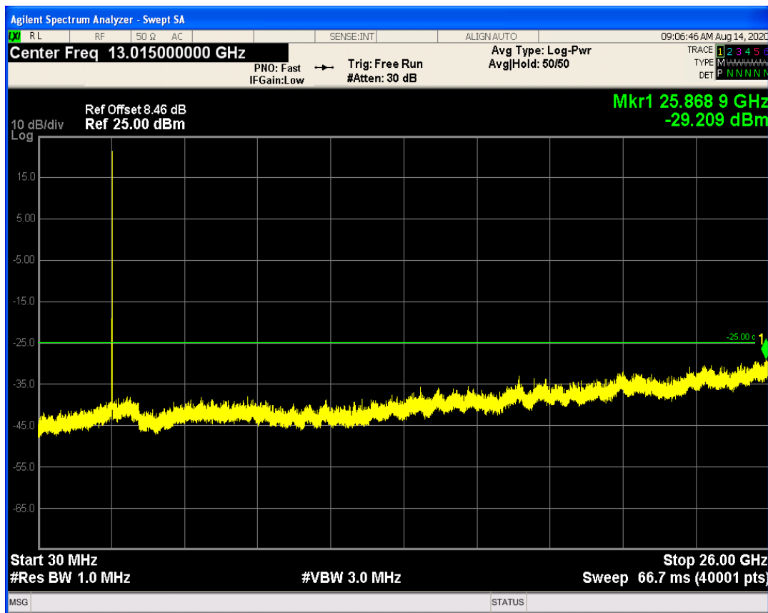
LTE Band41 QPSK BW=10MHz Channel=40290 RB Size=1 Position=#0
