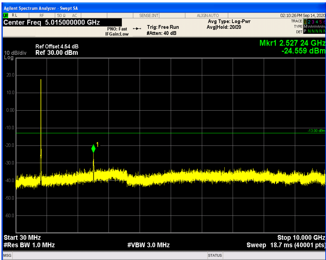
LTE Band41 QPSK BW=5MHz Channel=40265 RB Size=1 Position=#0
