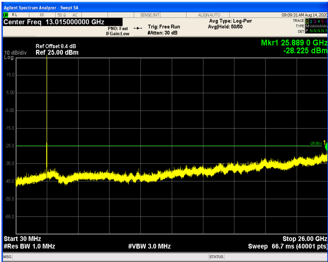
LTE Band41 QPSK BW=10MHz Channel=40740 RB Size=50 Position=#0
