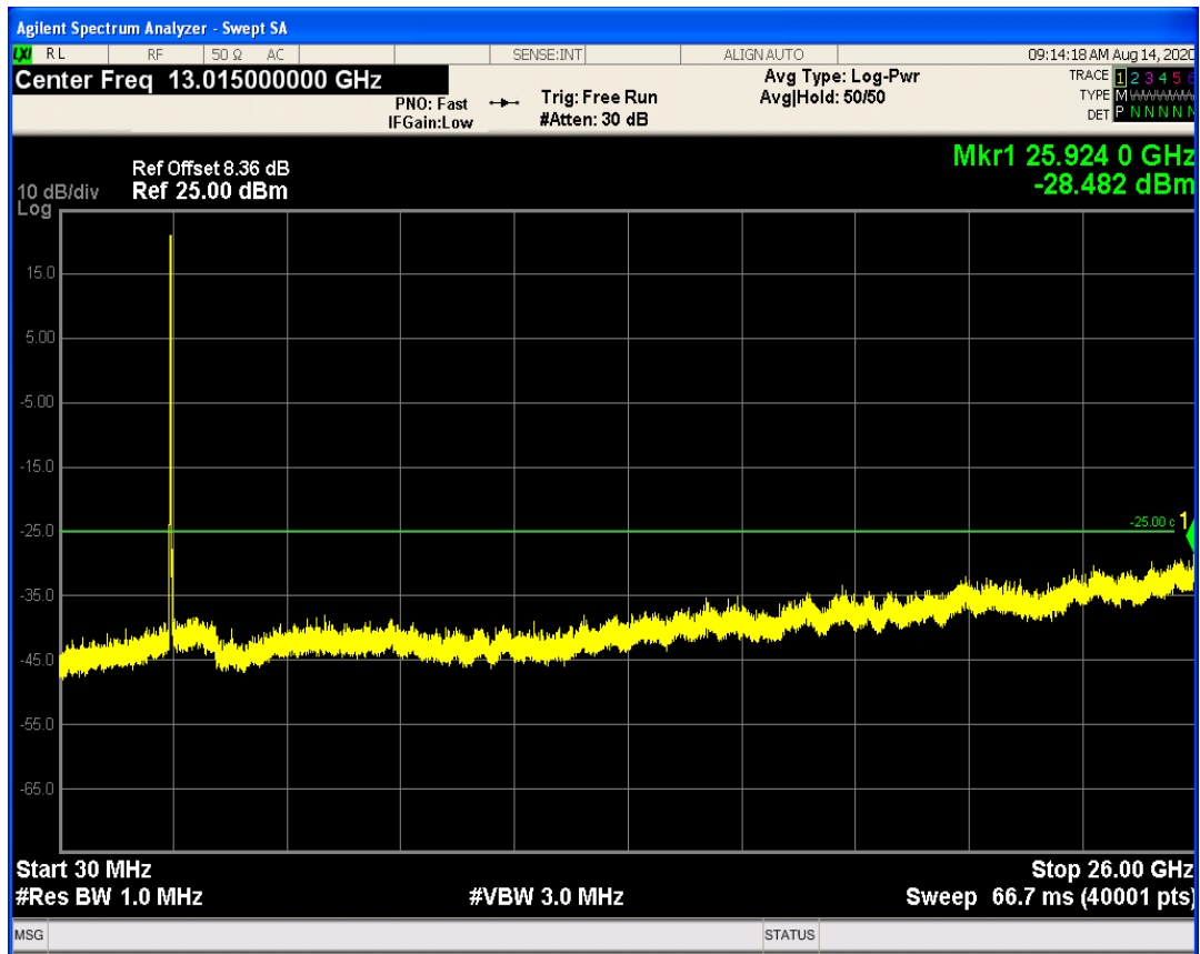
LTE Band41 QPSK BW=15MHz Channel=40315 RB Size=1 Position=#0
