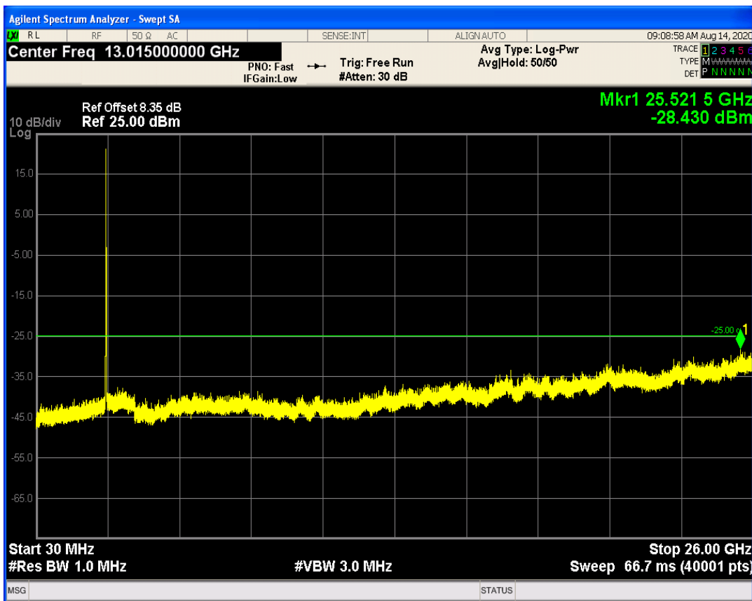
LTE Band41 QPSK BW=10MHz Channel=40740 RB Size=1 Position=#0
