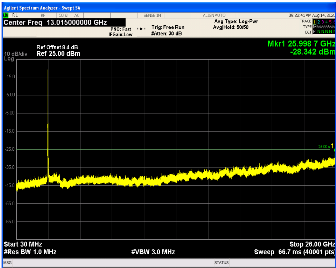
LTE Band41 QAM16 BW=20MHz Channel=40740 RB Size=100 Position=#0
