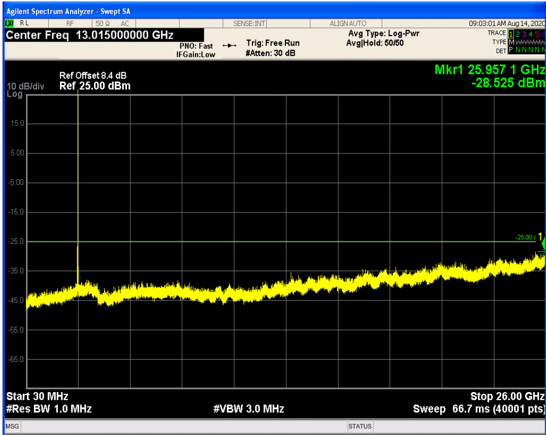
LTE Band41 QPSK BW=5MHz Channel=40740 RB Size=25 Position=#0
