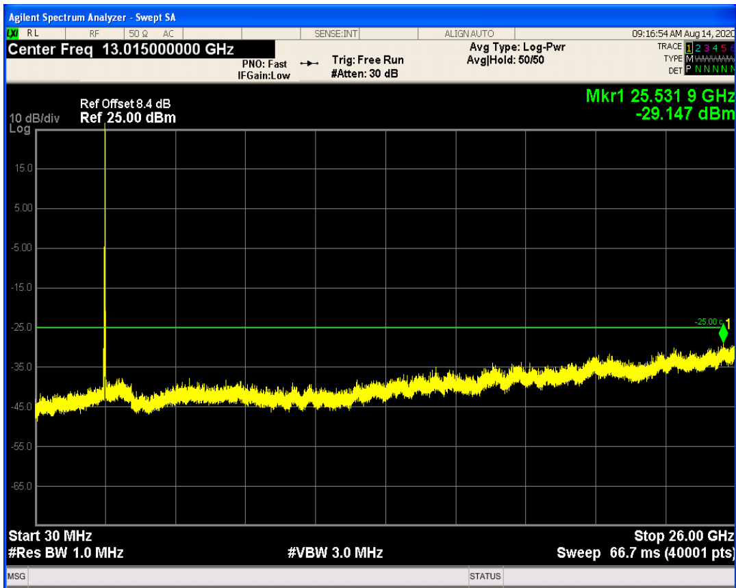
LTE Band41 QAM16 BW=15MHz Channel=40740 RB Size=75 Position=#0
