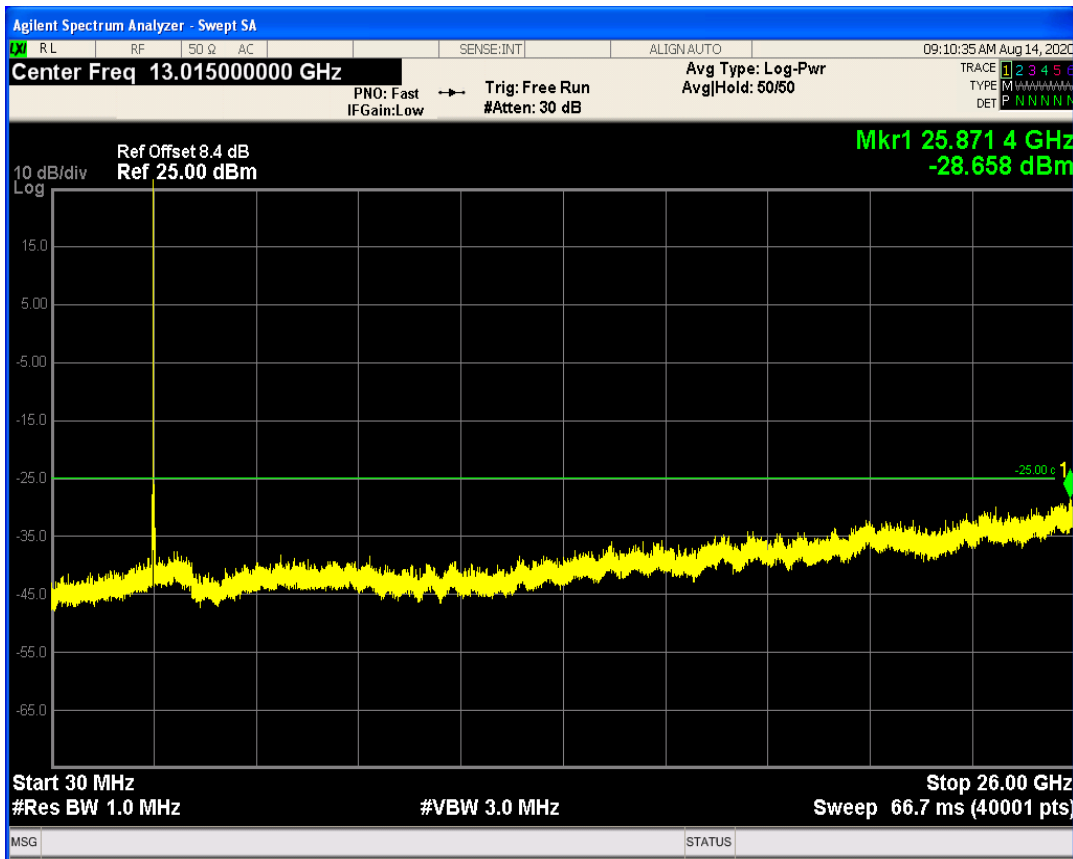
LTE Band41 QAM16 BW=10MHz Channel=40740 RB Size=50 Position=#0
