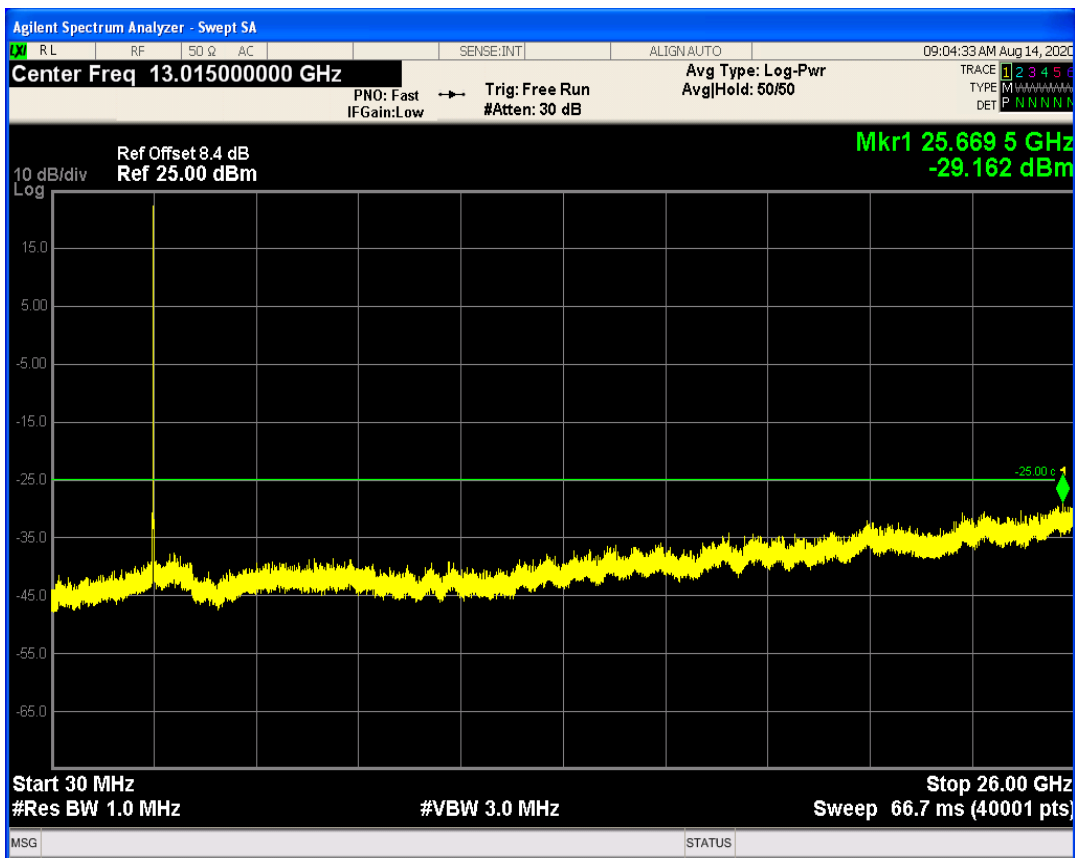
LTE Band41 QPSK BW=5MHz Channel=41215 RB Size=1 Position=#0
