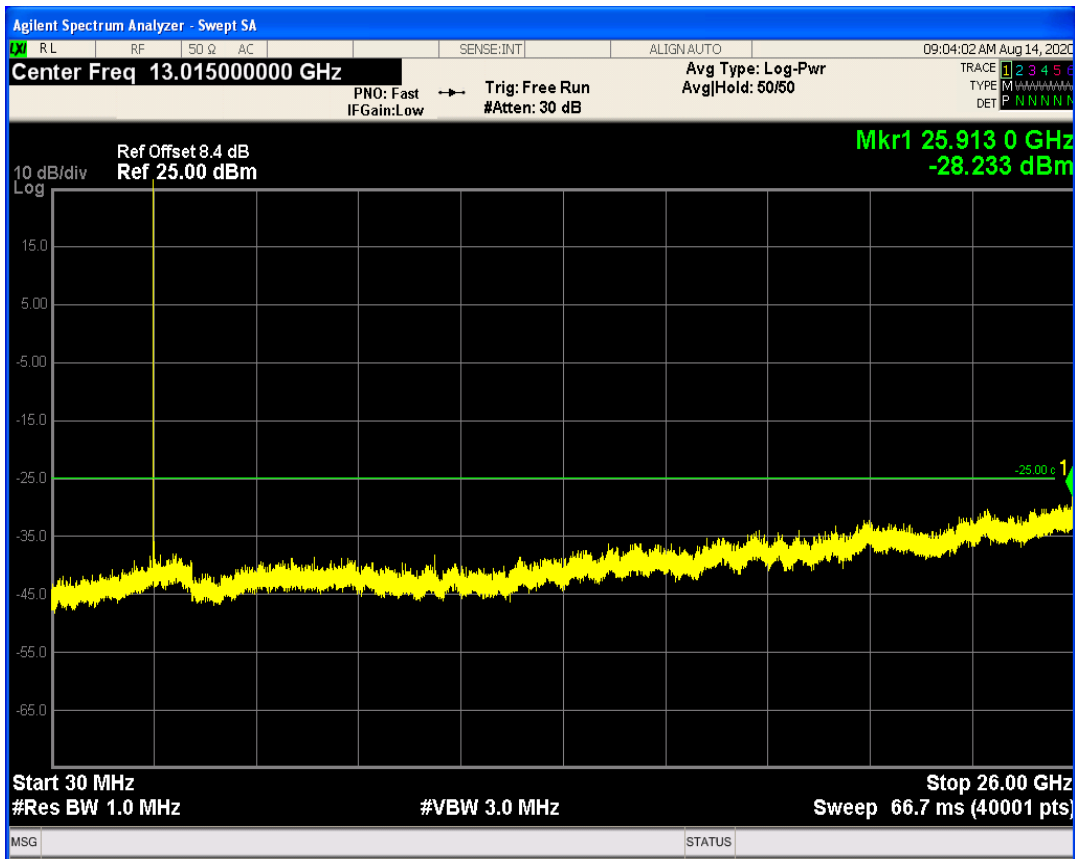
LTE Band41 QAM16 BW=5MHz Channel=40740 RB Size=25 Position=#0
