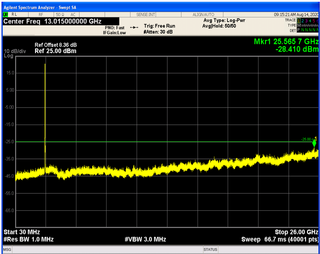
LTE Band41 QPSK BW=15MHz Channel=40740 RB Size=1 Position=#0
