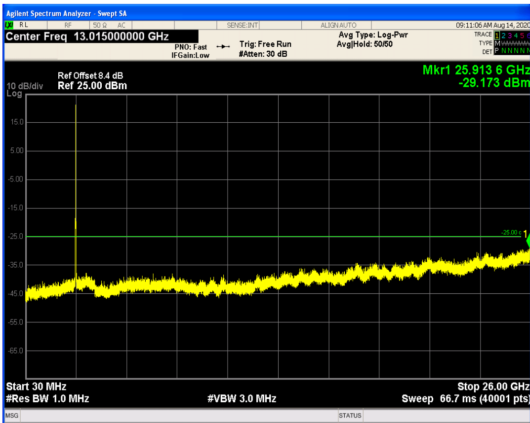
LTE Band41 QPSK BW=10MHz Channel=41190 RB Size=50 Position=#0
