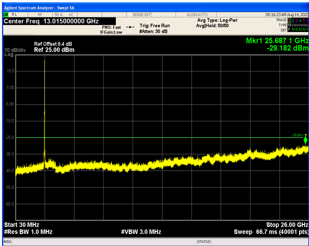
LTE Band41 QAM16 BW=15MHz Channel=40740 RB Size=1 Position=#0
