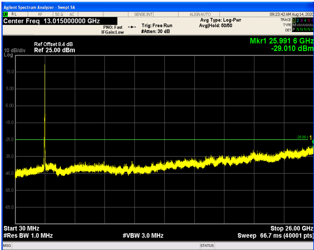
LTE Band41 QPSK BW=20MHz Channel=41140 RB Size=1 Position=#0
