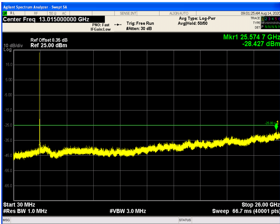
LTE Band41 QAM16 BW=5MHz Channel=40265 RB Size=1 Position=#0
