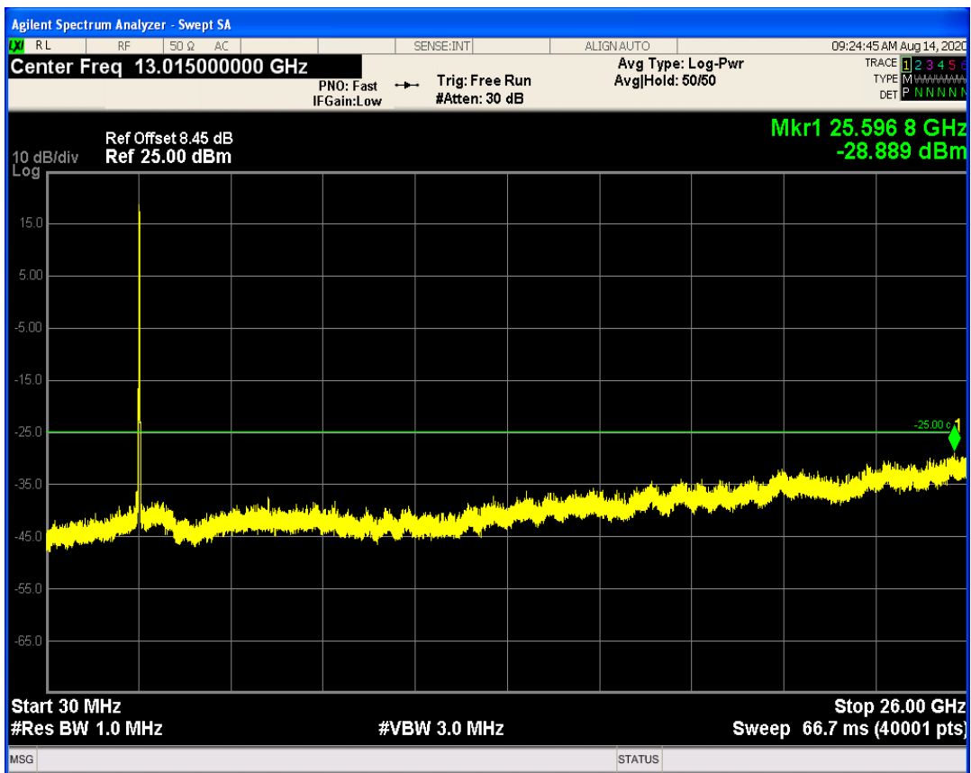
LTE Band41 QAM16 BW=20MHz Channel=41140 RB Size=1 Position=#0
