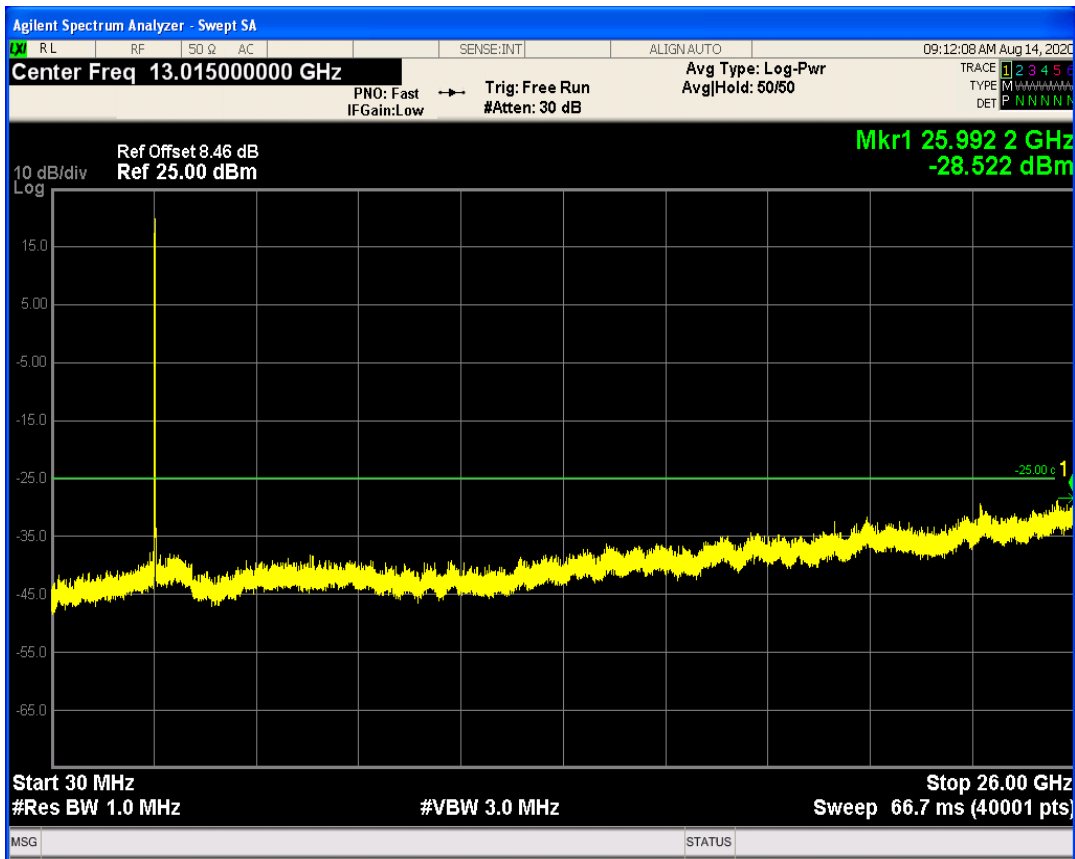
LTE Band41 QPSK BW=10MHz Channel=41190 RB Size=1 Position=#0
