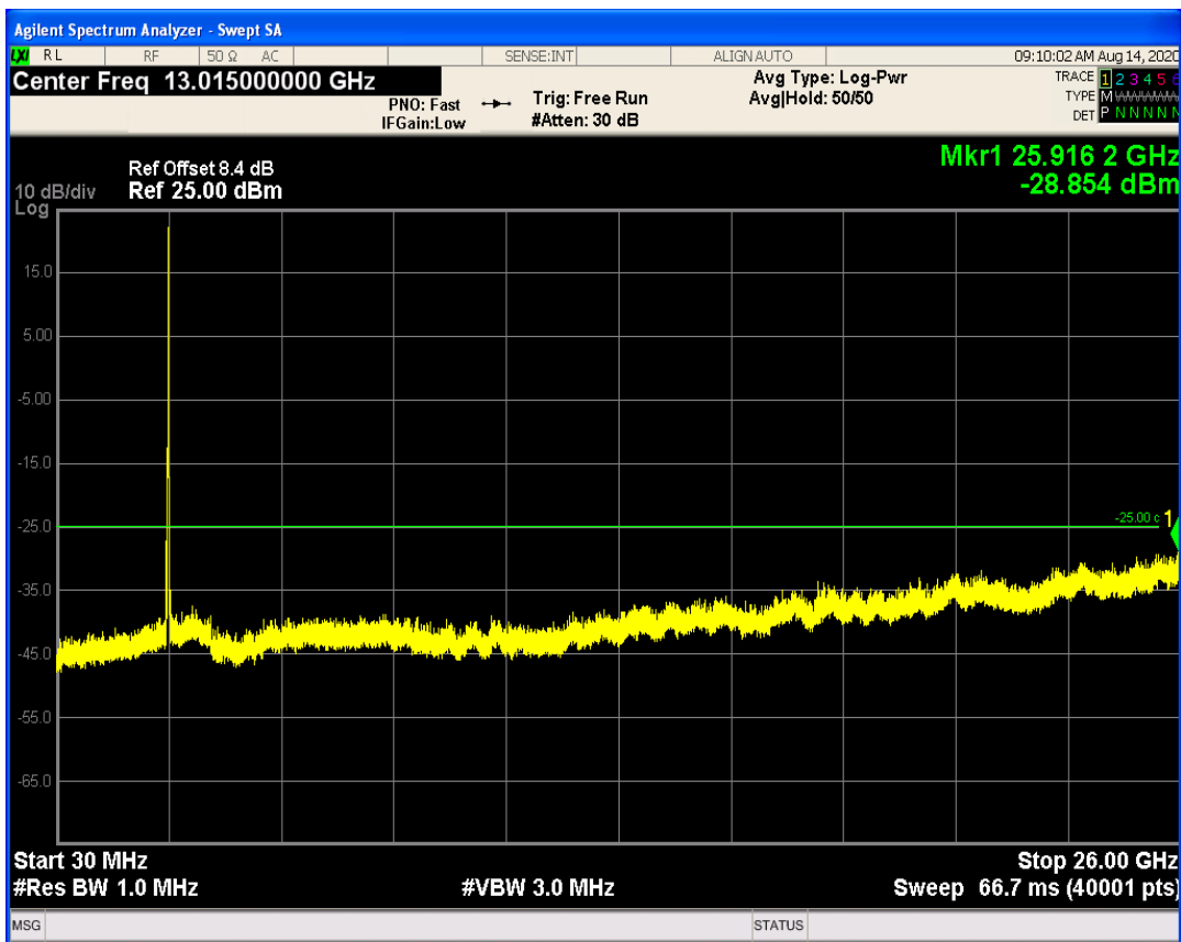
LTE Band41 QAM16 BW=10MHz Channel=40740 RB Size=1 Position=#0
