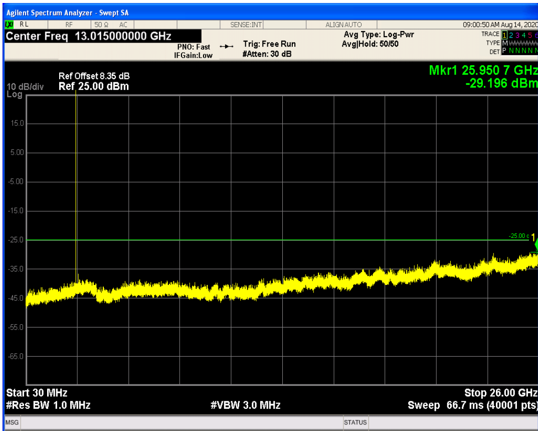
LTE Band41 QPSK BW=5MHz Channel=40265 RB Size=25 Position=#0
