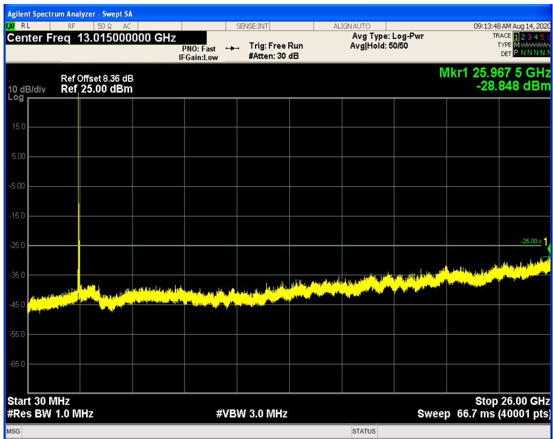
LTE Band41 QAM16 BW=15MHz Channel=40315 RB Size=1 Position=#0
