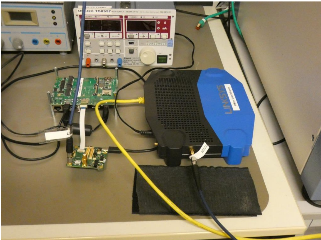
Photo 4: Test setup for conducted measurements
