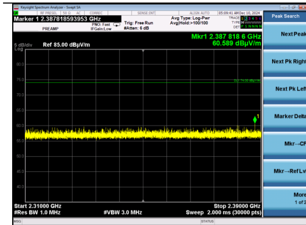
Channel 1 | 2M 2310-2390 MHz | Horizontal
