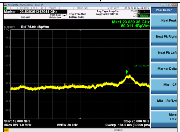
Channel 19 | 1M 18000-25000 MHz | Vertical
