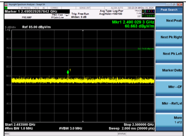
Channel 39 | 125k 2483.5-2500 MHz | Horizontal
