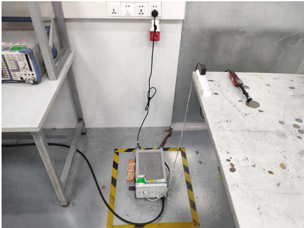
FCC ID: WQ8TBE200 Photo of Power Line Conducted Emission Test
