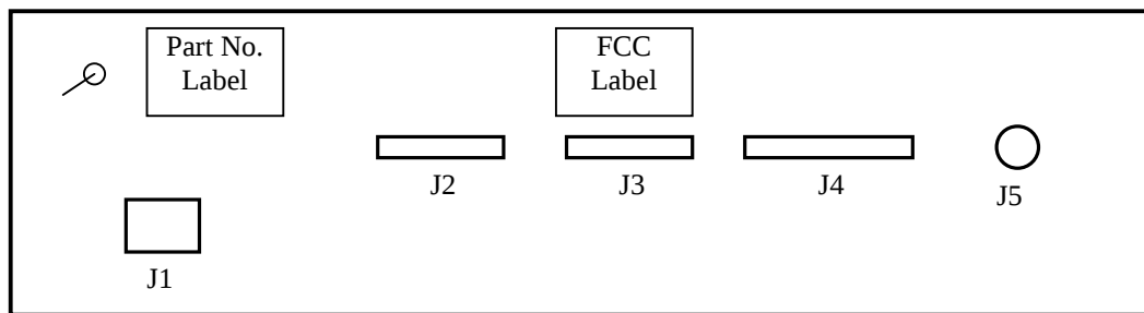
Figure 2 BDR (385700-3000) FCC Label Location
