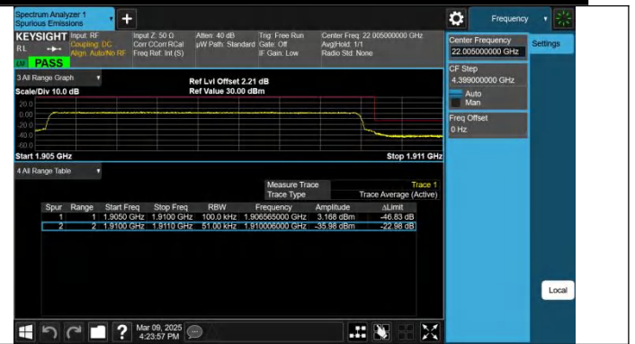
Band2-5MHz-QPSK-19175-25RB#0-PASS
