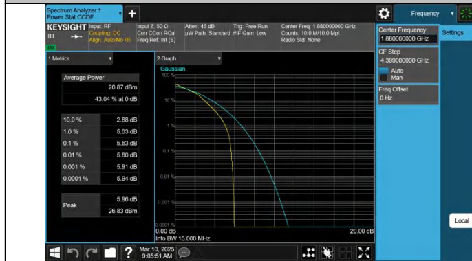
Band2-15MHz-16QAM-18900-27RB#0-PASS
