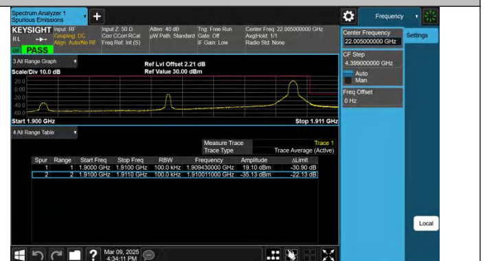
Band2-10MHz-QPSK-19150-1RB#49-PASS
