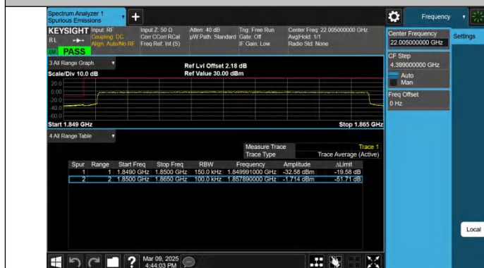
Band2-15MHz-QPSK-18675-75RB#0-PASS
