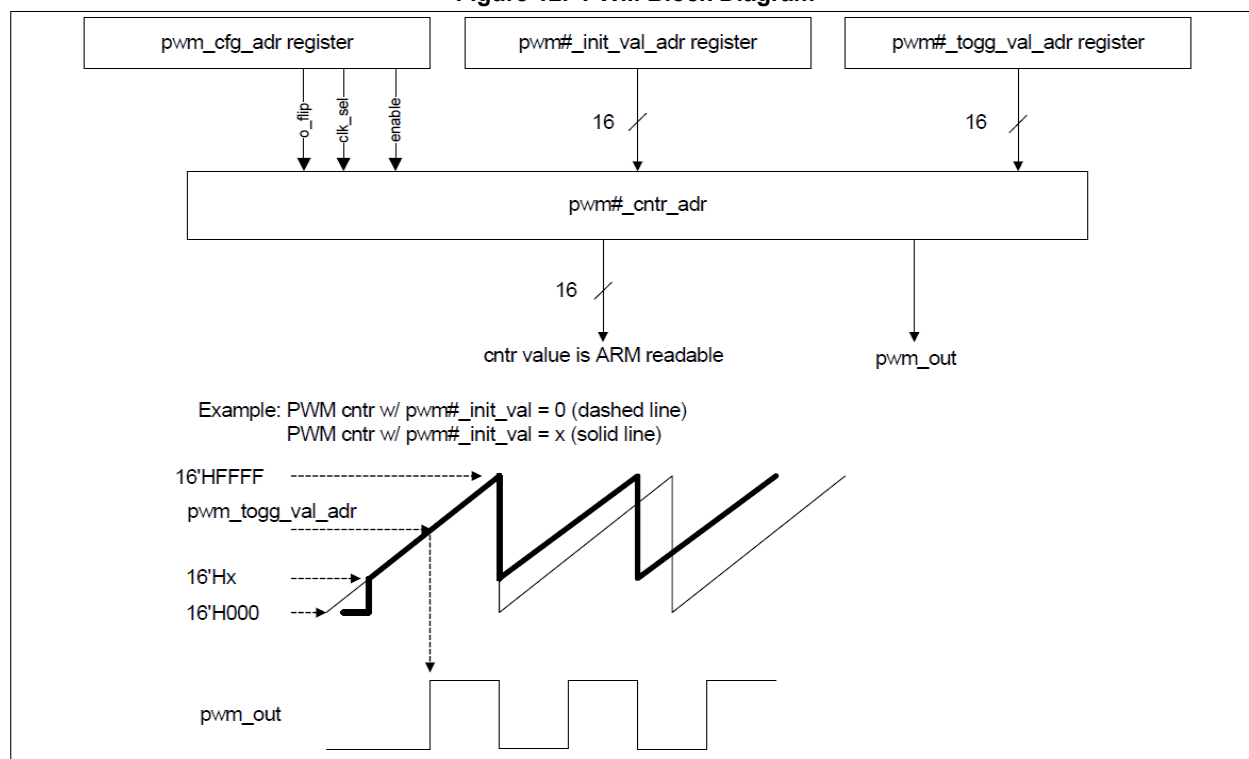
Figure 12. PWM Block Diagram
