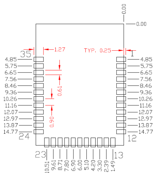
Figure 6. CYBT-213043-02 Host Layout (Relative to Origin)
