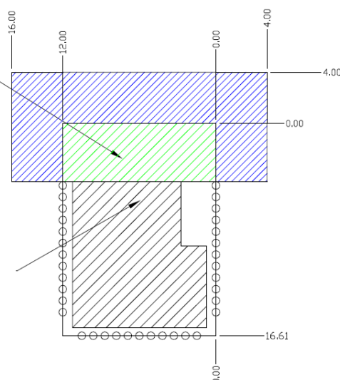
Figure 4. Optional Additional Host PCB Keep Out Area Around the CYBT-213043-02 PCB Antenna
