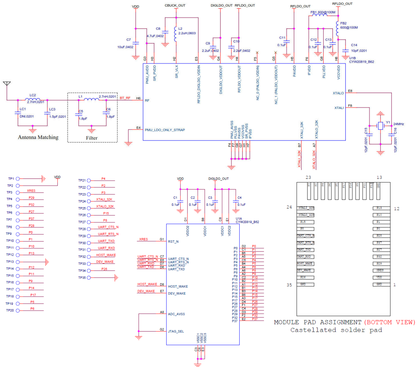
Figure 8. CYBT-213043-02 Schematic Diagram
