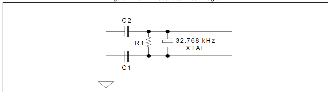
Figure 11. 32 kHz Oscillator Block Diagram
