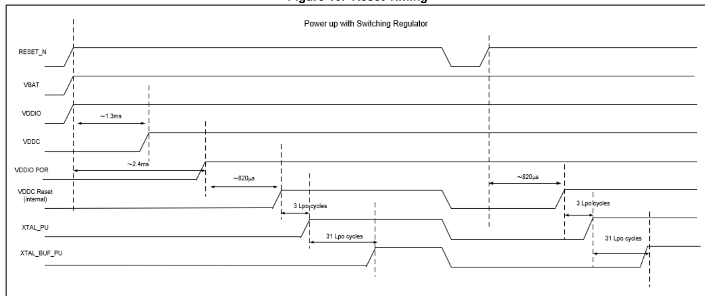
Figure 10. Reset Timing
