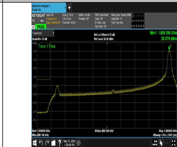
Band2_10MHz_16QAM_18650_1RB#49
