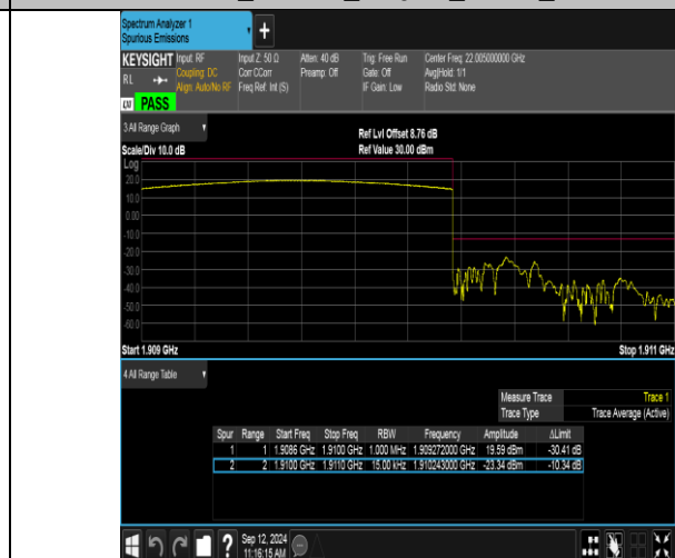
Band2_1.4MHz_16QAM_19193_6RB#0
