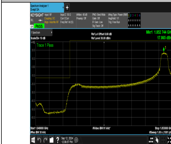
Band2_3MHz_QPSK_18615_1RB#14
