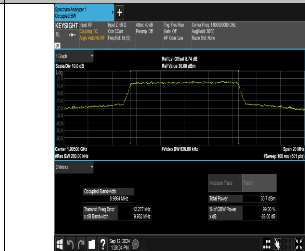
Band2-10MHz-16QAM-19150-50RB#0-PASS
