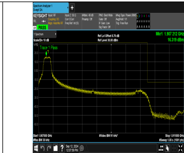
Band2_3MHz_16QAM_19185_1RB#0
