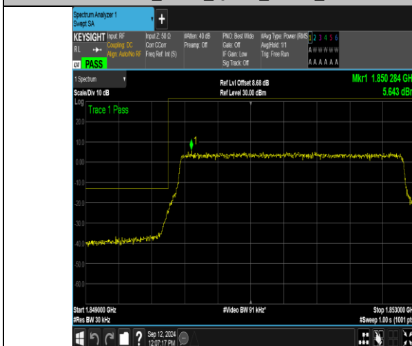
Band2_3MHz_QPSK_18615_15RB#0
