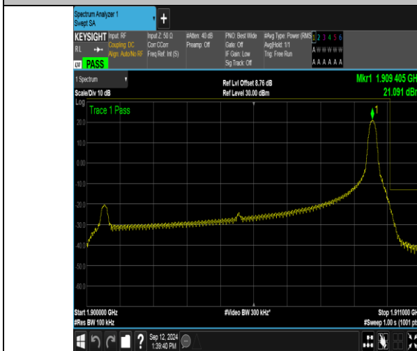
Band2_10MHz_QPSK_19150_1RB#49
