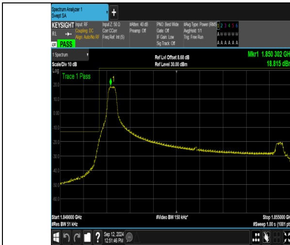
Band2_5MHz_QPSK_18625_1RB#0
