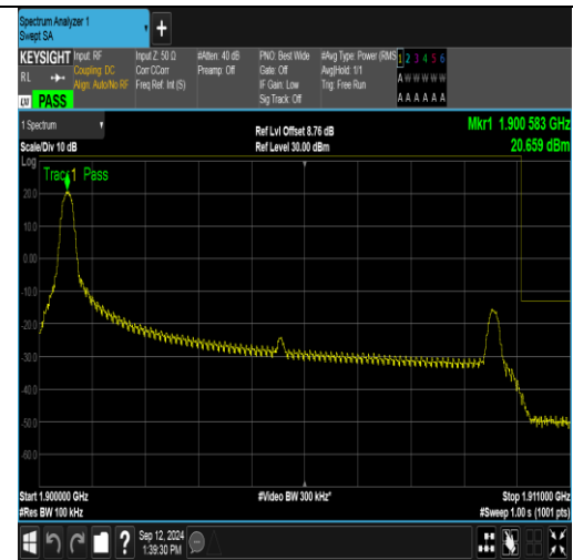
Band2_10MHz_16QAM_19150_1RB#0
