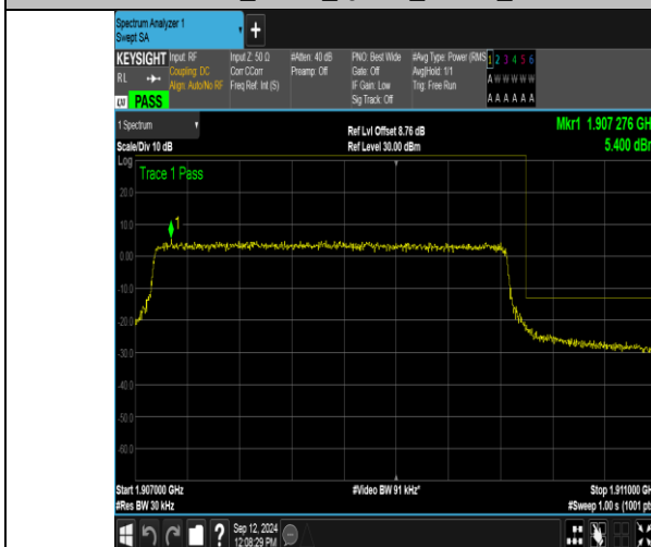
Band2_3MHz_QPSK_19185_15RB#0
