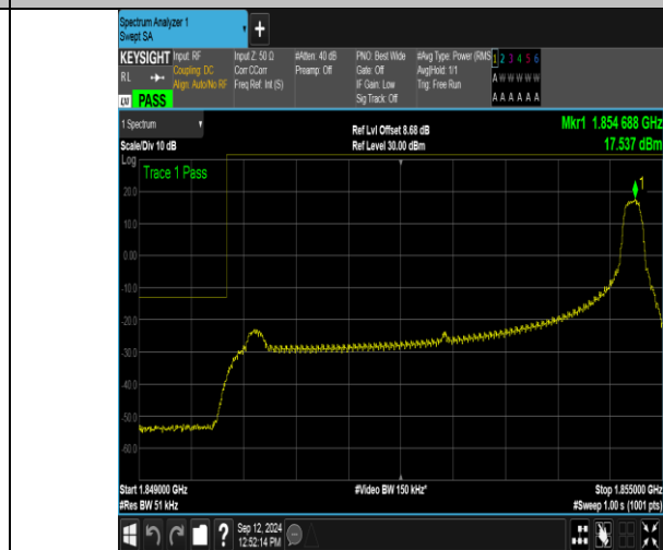
Band2_5MHz_16QAM_18625_1RB#24
