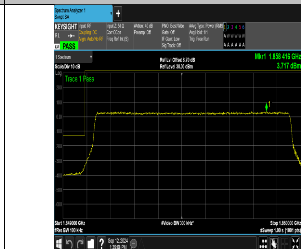
Band2_10MHz_16QAM_18650_50RB#0
