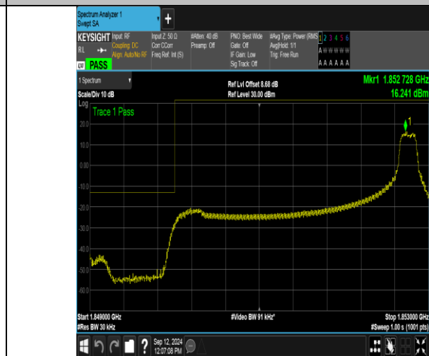
Band2_3MHz_16QAM_18615_1RB#14
