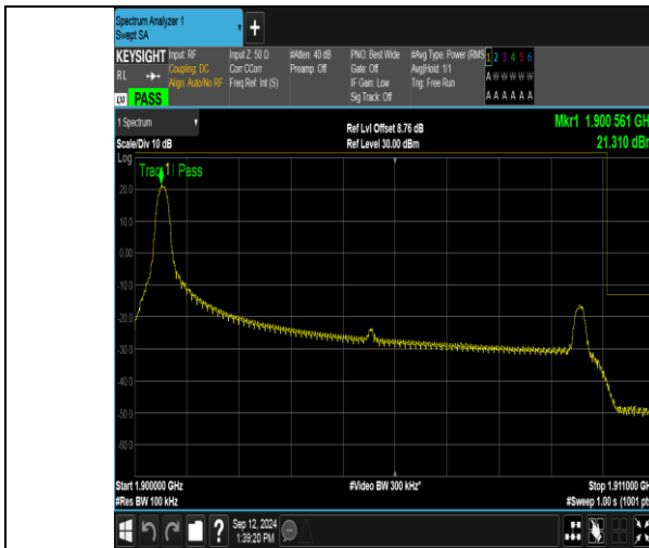
Band2_10MHz_QPSK_19150_1RB#0
