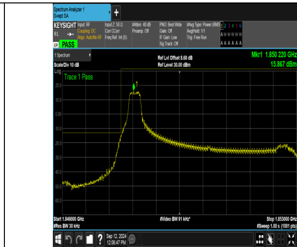
Band2_3MHz_16QAM_18615_1RB#0
