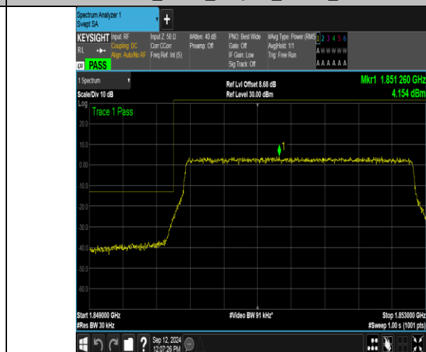
Band2_3MHz_16QAM_18615_15RB#0
