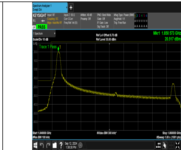
Band2_10MHz_16QAM_18650_1RB#0
