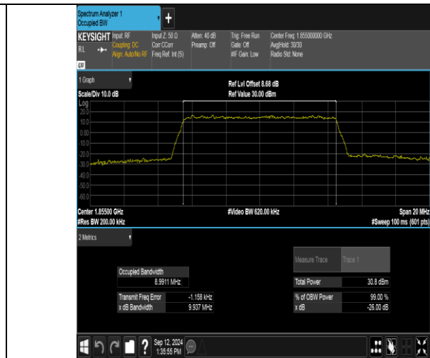
Band2-10MHz-16QAM-18650-50RB#0-PASS
