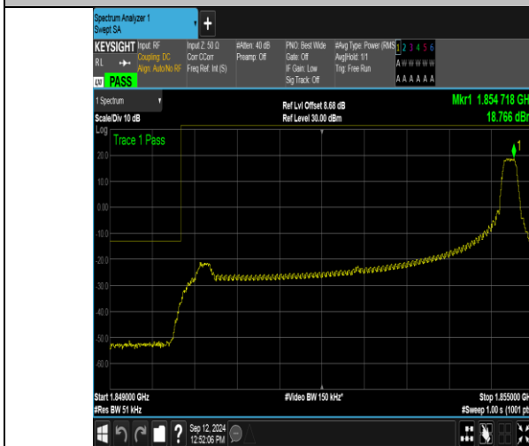
Band2_5MHz_QPSK_18625_1RB#24
