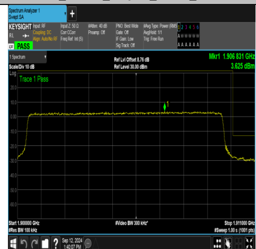
Band2_10MHz_16QAM_19150_50RB#0
