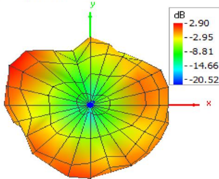
Figure G-1 Pattern at 5580 MHz (Top / Bottom view)
