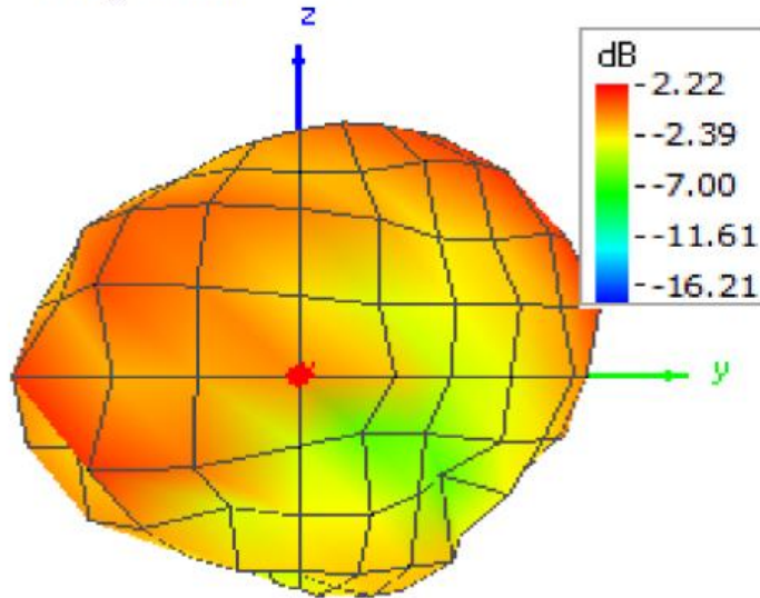
Figure D-2 Pattern at 2472 MHz (Front / Back view)
