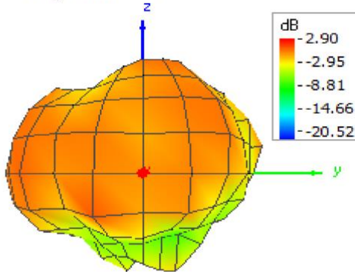
Figure G-2 Pattern at 5580 MHz (Front / Back view)
