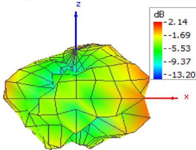
Figure B-3 Pattern at 2412 MHz (Left / Right view)
