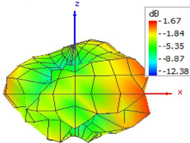
Figure C-3 Pattern at 2442 MHz (Left / Right view)
