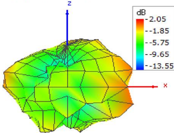
Figure A-3 Pattern at 2402 MHz (Left / Right view)
