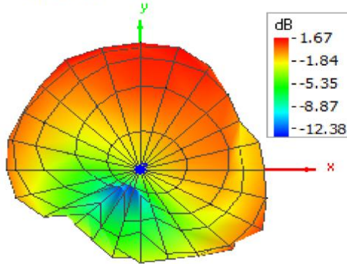
Figure C-1 Pattern at 2442 MHz (Top / Bottom view)
