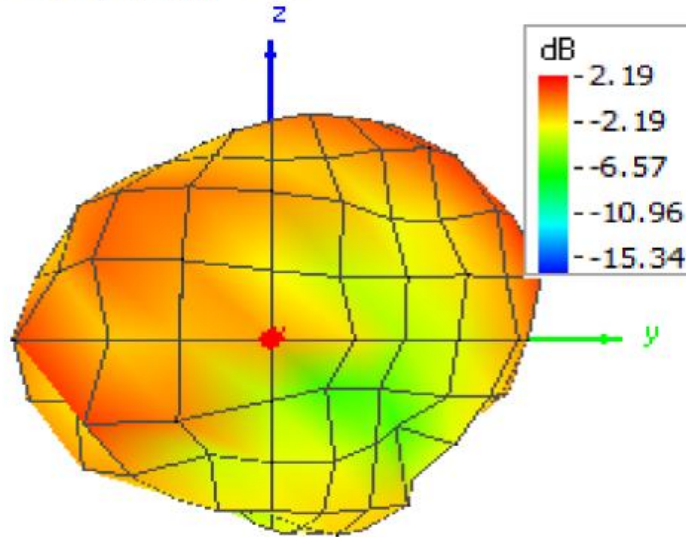
Figure E-2 Pattern at 2480 MHz (Front / Back view)
