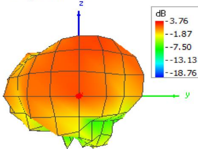
Figure F-2 Pattern at 5180 MHz (Front / Back view)
