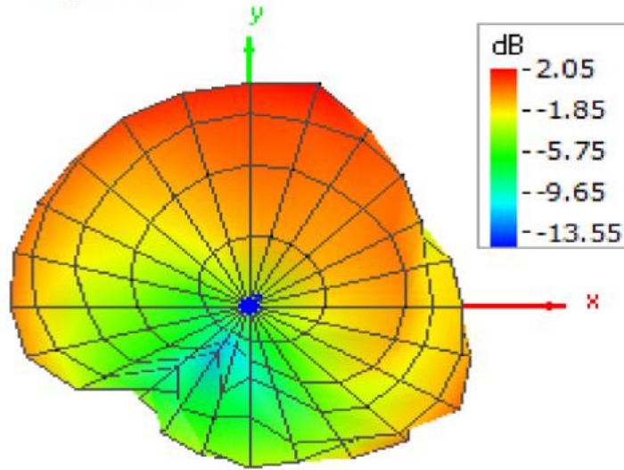
Figure A-1 Pattern at 2402 MHz (Top / Bottom view)
