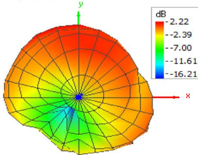
Figure D-1 Pattern at 2472 MHz (Top / Bottom view)
