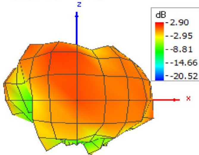
Figure G-3 Pattern at 5580 MHz (Left / Right view)
