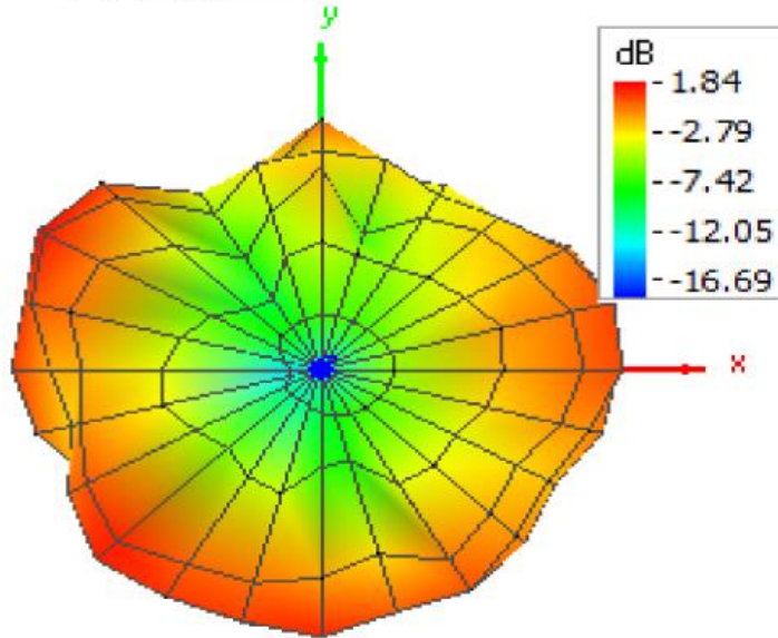
Figure H-1 Pattern at 5825 MHz (Top / Bottom view)
