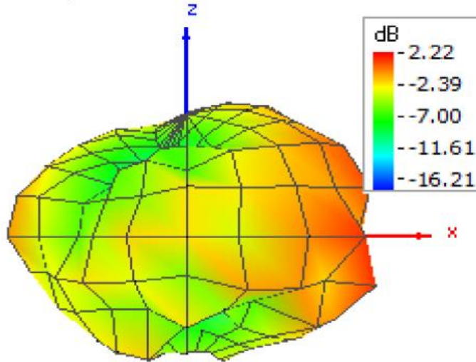
Figure D-3 Pattern at 2472 MHz (Left / Right view)
