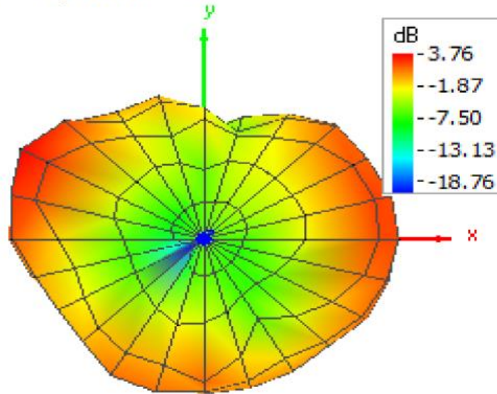
Figure F-1 Pattern at 5180 MHz (Top / Bottom view)
