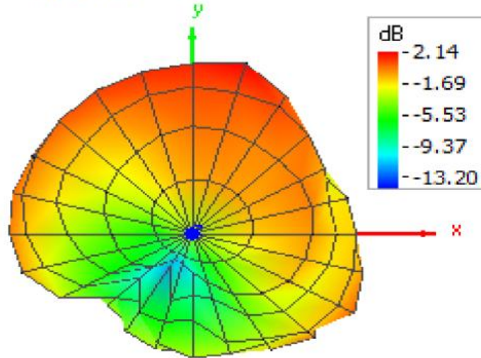
Figure B-1 Pattern at 2412 MHz (Top / Bottom view)
