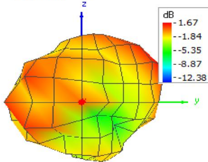
Figure C-2 Pattern at 2442 MHz (Front / Back view)
