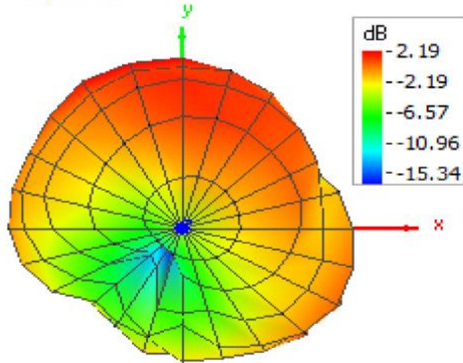
Figure E-1 Pattern at 2480 MHz (Top / Bottom view)
