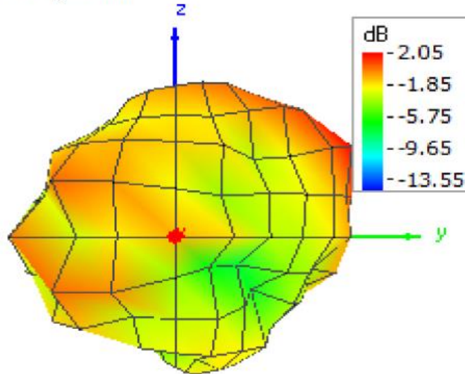
Figure A-2 Pattern at 2402 MHz (Front / Back view)
