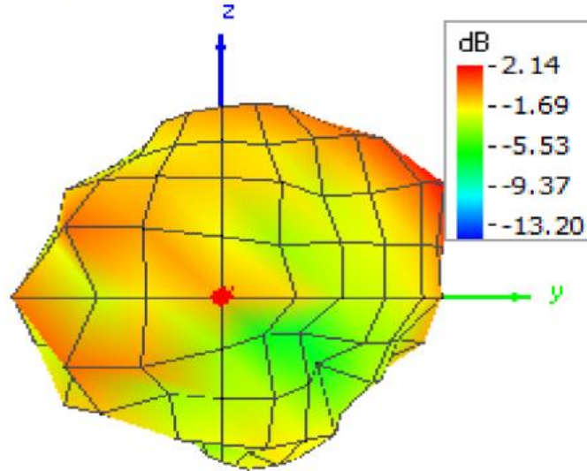
Figure B-2 Pattern at 2412 MHz (Front / Back view)
