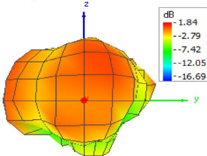
Figure H-2 Pattern at 5825 MHz (Front / Back view)
