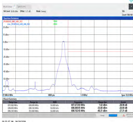
1-N71-15-5-H-5-CP-QPSK-Edge_1RB_Right-1@24-Ant1-1--PASS-see graph
