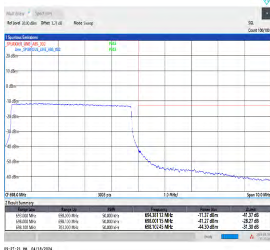
1-N71-15-5-H-6-CP-QPSK-Outer_Full-25@0-Ant1-1--PASS-see graph
