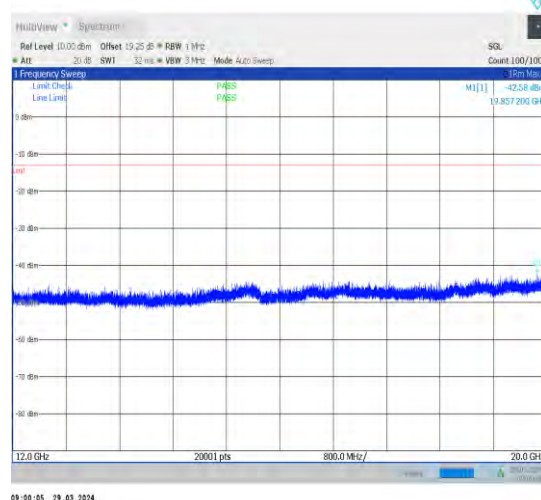
1-N71-15-20-M-1-DFT-PI2BPSK-Inner_1RB_Left-1@ 1-12000-20000-Ant1-19857.20--42.58--13-PASS
