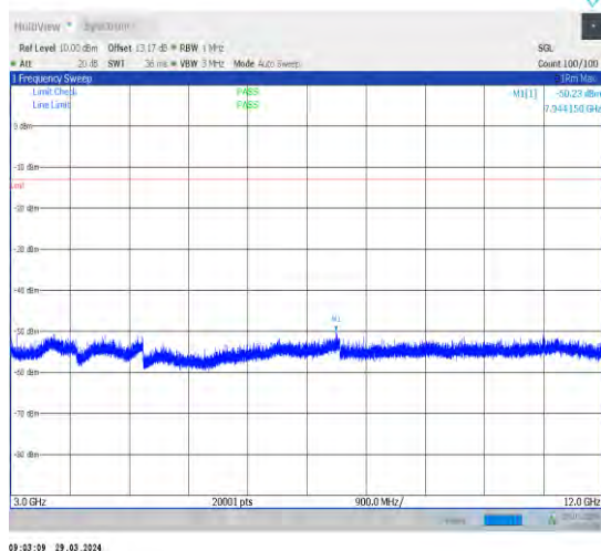
1-N71-15-20-H-1-DFT-PI2BPSK-Inner_1RB_Left-1 @1-3000-12000-Ant1-7944.15--50.23--13-PASS
