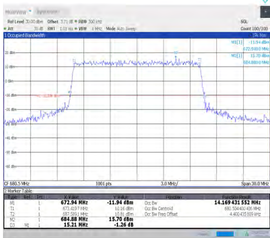
1-N71-15-15-M-7-CP-16QAM-Outer_Full-79@0-Ant1 1-14.169-15.210-≤15-PASS
