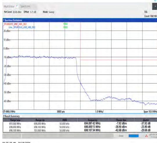
1-N71-15-5-H-3-DFT-PI2BPSK-Outer_Full-25@0-Ant1-1--PASS-see graph
