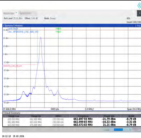
1-N71-15-15-L-1-DFT-PI2BPSK-Edge_1RB_Left-1@0-Ant1-1--PASS-see graph
