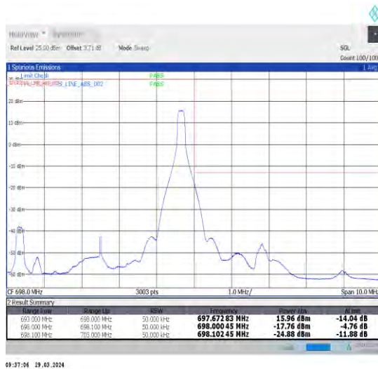
1-N71-15-5-H-5-CP-QPSK-Edge_1RB_Right-1@24-Ant1-1--PASS-see graph
