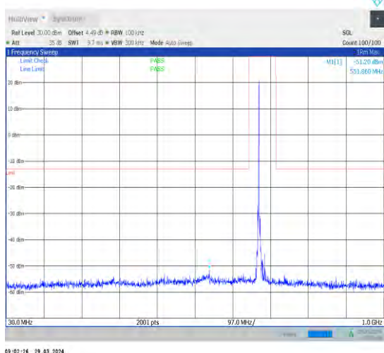
1-N71-15-20-H-1-DFT-PI2BPSK-Inner_1RB_Left-1 @1-30-1000-Ant1-551.86--51.20--13-PASS
