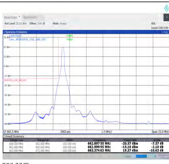
1-N71-15-10-L-1-DFT-PI2BPSK-Edge_1RB_Left-1@0-Ant1-1--PASS-see graph
