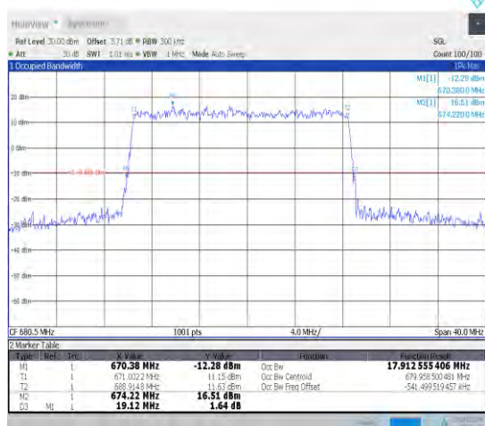
1-N71-15-20-M-1-DFT-QPSK-Outer_Full-100@0-Ant1 1-17.913-19.120-≤20-PASS
