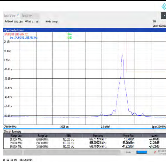
1-N71-15-15-H-2-DFT-PI2BPSK-Edge_1RB_Right-1@78-Ant1-1--PASS-see graph
