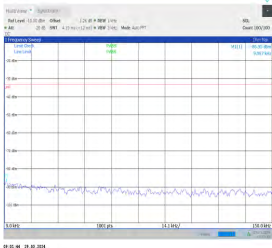
1-N71-15-20-H-1-DFT-PI2BPSK-Inner_1RB_Left-1 @1-0.009-0.15-Ant1-0.01--86.95--33-PASS
