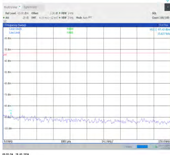
1-N71-15-20-L-1-DFT-PI2BPSK-Inner_1RB_Left-1 @1-0.009-0.15-Ant1-0.02--87.43--33-PASS
