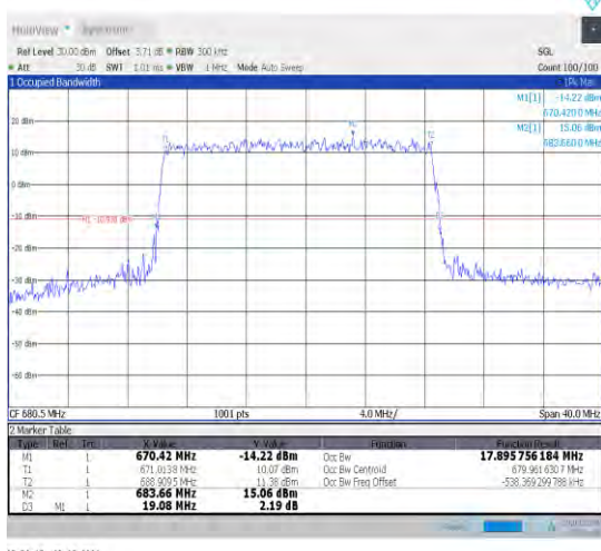
1-N71-15-20-M-4-DFT-64QAM-Outer_Full-100@0-A nt1-17.896-19.080-≤20-PASS
