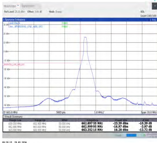
1-N71-15-5-L-4-CP-QPSK-Edge_1RB_Left-1@0-A nt1-1--PASS-see graph
