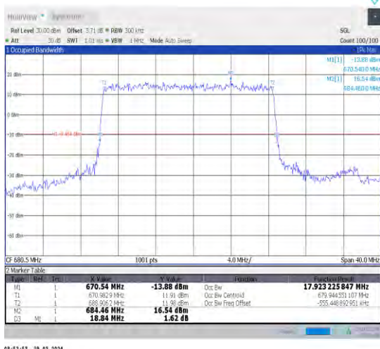
1-N71-15-20-M-2-DFT-PI2BPSK-Outer_Full-100@0-A Ant1-17.923-18.840-≤20-PASS
