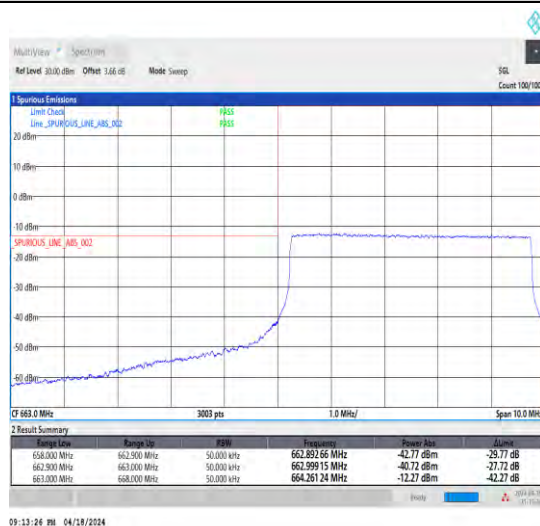
1-N71-15-5-L-6-CP-QPSK-Outer_Full-25@0-Ant1-1--PASS-see graph
