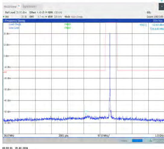
1-N71-15-20-M-1-DFT-PI2BPSK-Inner_1RB_Left-1 @1-30-1000-Ant1-526.64--52.83--13-PASS
