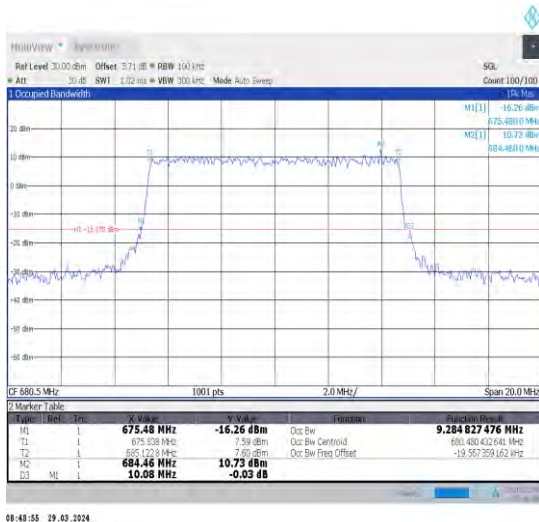
1-N71-15-10-M-6-CP-QPSK-Outer_Full-52@0-Ant1- 9.285-10.080-≤10-PASS
