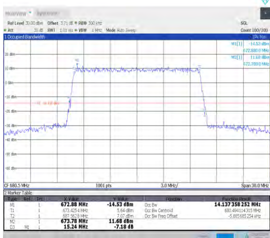
1-N71-15-15-M-9-CP-256QAM-Outer_Full-79@0-Ant1 1-14.137-15.240-≤15-PASS
