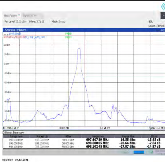
1-N71-15-5-H-2-DFT-PI2BPSK-Edge_1RB_Right-1@2 4-Ant1-1--PASS-see graph
