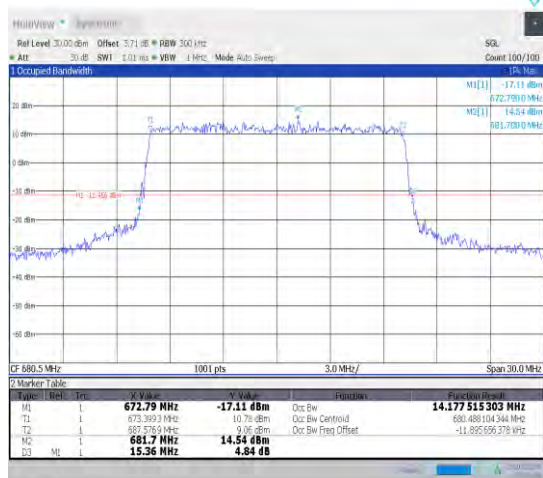
1-N71-15-15-M-8-CP-64QAM-Outer_Full-79@0-Ant1 1-14.178-15.360-≤15-PASS
