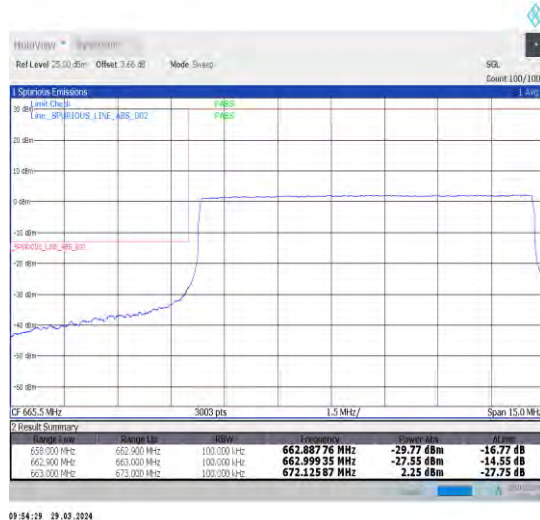
1-N71-15-10-L-6-CP-QPSK-Outer_Full-52@0-Ant1-1--PASS-see graph
