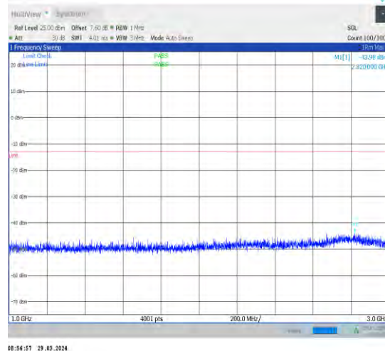
1-N71-15-20-L-1-DFT-PI2BPSK-Inner_1RB_Left-1@ 1-1000-3000-Ant1-2820.00--43.98--13-PASS
