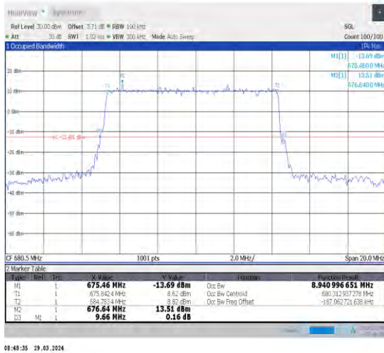
1-N71-15-10-M-4-DFT-64QAM-Outer_Full-50@0-Ant 1-8.941-9.660-≤10-PASS
