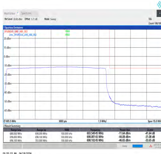
1-N71-15-10-H-6-CP-QPSK-Outer_Full-52@0-Ant1-1--PASS-see graph
