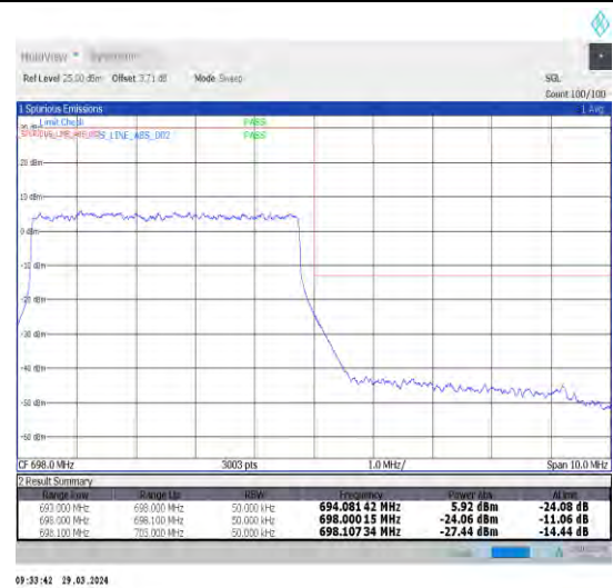
1-N71-15-5-H-3-DFT-PI2BPSK-Outer_Full-25@0-Ant1-1--PASS-see graph
