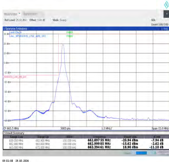
1-N71-15-10-L-4-CP-QPSK-Edge_1RB_Left-1@0-Ant1-1--PASS-see graph
