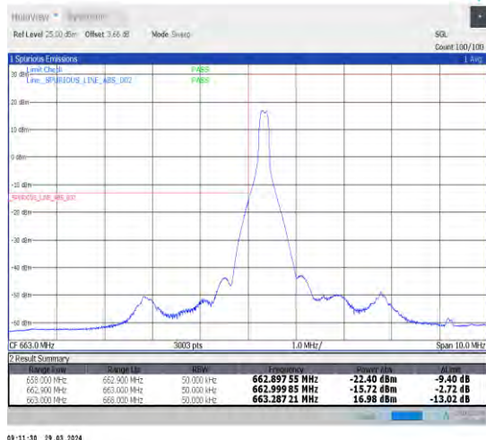
1-N71-15-5-L-1-DFT-PI2BPSK-Edge_1RB_Left-1@0-A nt1-1--PASS-see graph
