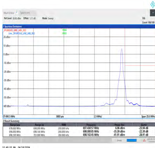
1-N71-15-20-H-5-CP-QPSK-Edge_1RB_Right-1@105-Ant1-1--PASS-see graph
