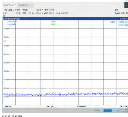
1-N71-15-20-H-1-DFT-PI2BPSK-Inner_1RB_Left-1@ 1-0.15-30-Ant1-9.64--83.55--23-PASS
