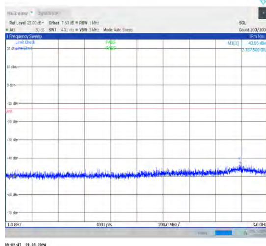
1-N71-15-20-H-1-DFT-PI2BPSK-Inner_1RB_Left-1@ 1-1000-3000-Ant1-2787.50--43.56--13-PASS
