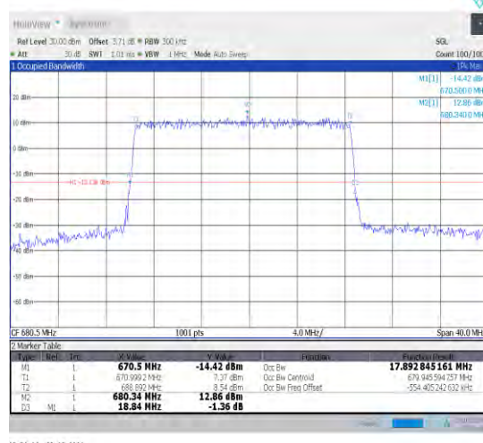
1-N71-15-20-M-5-DFT-256QAM-Outer_Full-100@0-A Ant1-17.893-18.840-≤20-PASS
