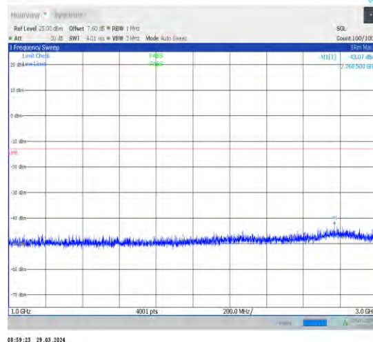
1-N71-15-20-M-1-DFT-PI2BPSK-Inner_1RB_Left-1@ 1-1000-3000-Ant1-2768.50--43.07--13-PASS
