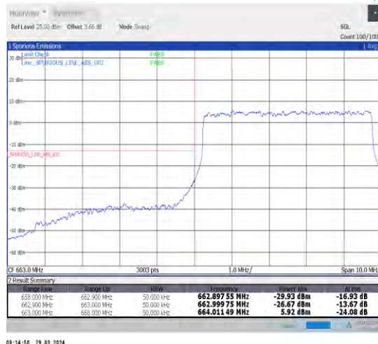
1-N71-15-5-L-3-DFT-PI2BPSK-Outer_Full-25@0-A Ant1-1--PASS-see graph
