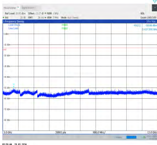
1-N71-15-20-M-1-DFT-PI2BPSK-Inner_1RB_Left-1 @1-3000-12000-Ant1-3637.20--50.06--13-PASS
