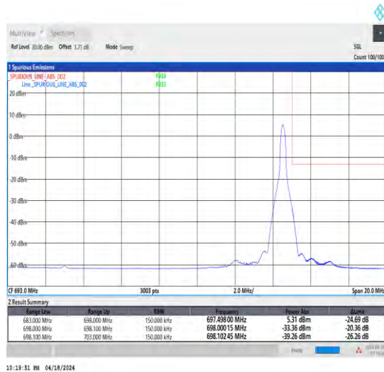
1-N71-15-15-H-5-CP-QPSK-Edge_1RB_Right-1@78-Ant1-1--PASS-see graph
