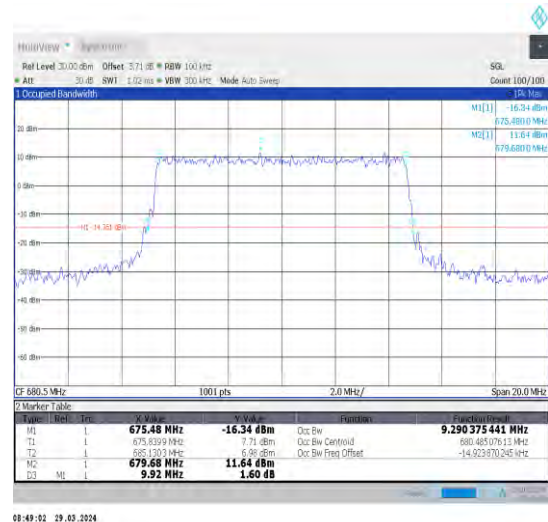
1-N71-15-10-M-7-CP-16QAM-Outer_Full-52@0-Ant 1-9.29-9.920-≤10-PASS
