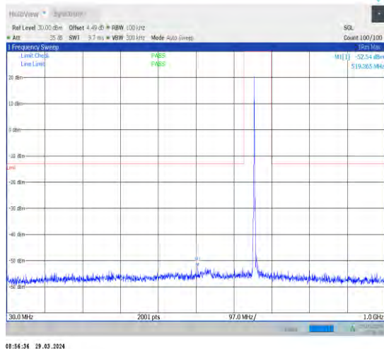
1-N71-15-20-L-1-DFT-PI2BPSK-Inner_1RB_Left-1 @1-30-1000-Ant1-519.37--52.54--13-PASS
