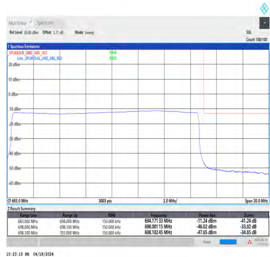
1-N71-15-15-H-6-CP-QPSK-Outer_Full-79@0-Ant1-1--PASS-see graph
