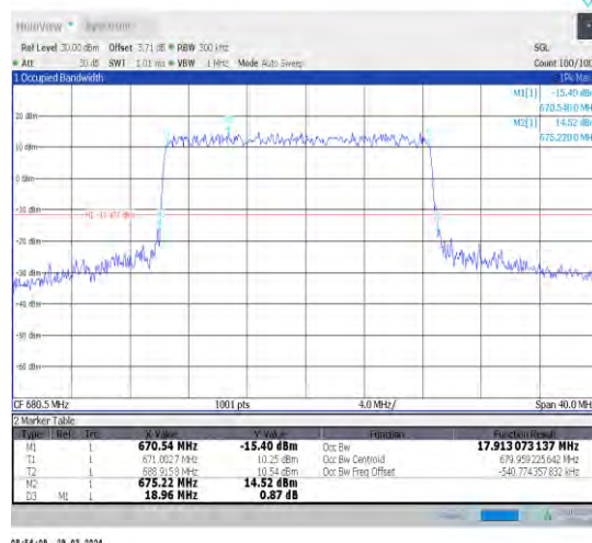
1-N71-15-20-M-3-DFT-16QAM-Outer_Full-100@0-A nt1-17.913-18.960-≤20-PASS
