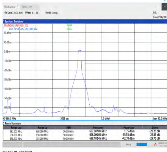
1-N71-15-5-H-2-DFT-PI2BPSK-Edge_1RB_Right-1@2 4-Ant1-1--PASS-see graph
