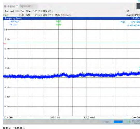
1-N71-15-20-H-1-DFT-PI2BPSK-Inner_1RB_Left-1@ 1-12000-20000-Ant1-19906.00--42.54--13-PASS
